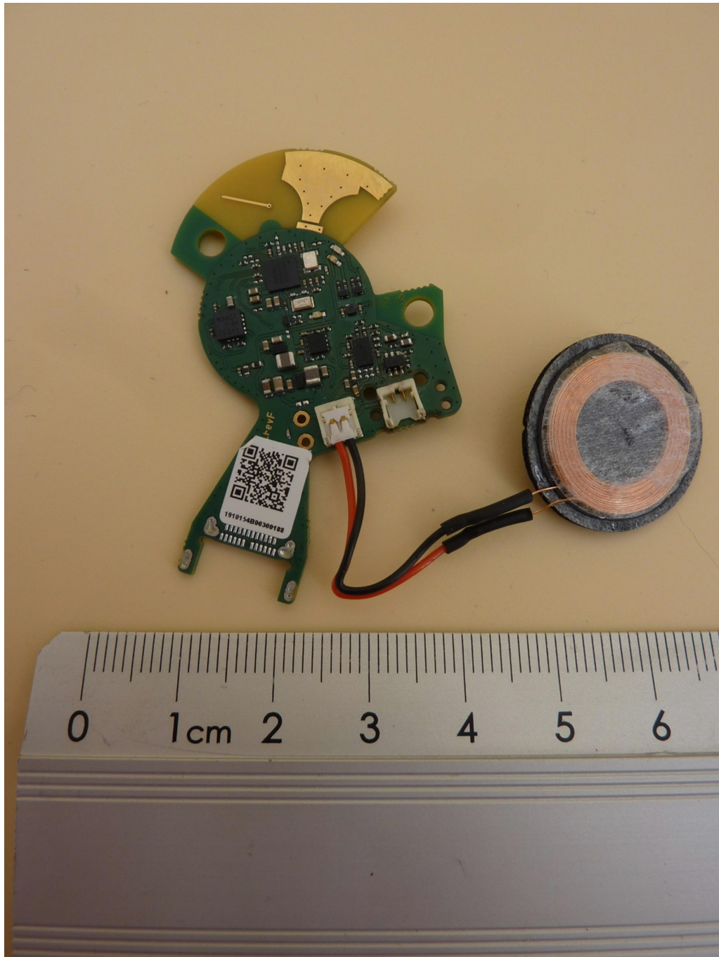
omlox WTag, internal view 3 (housing and battery removed)
