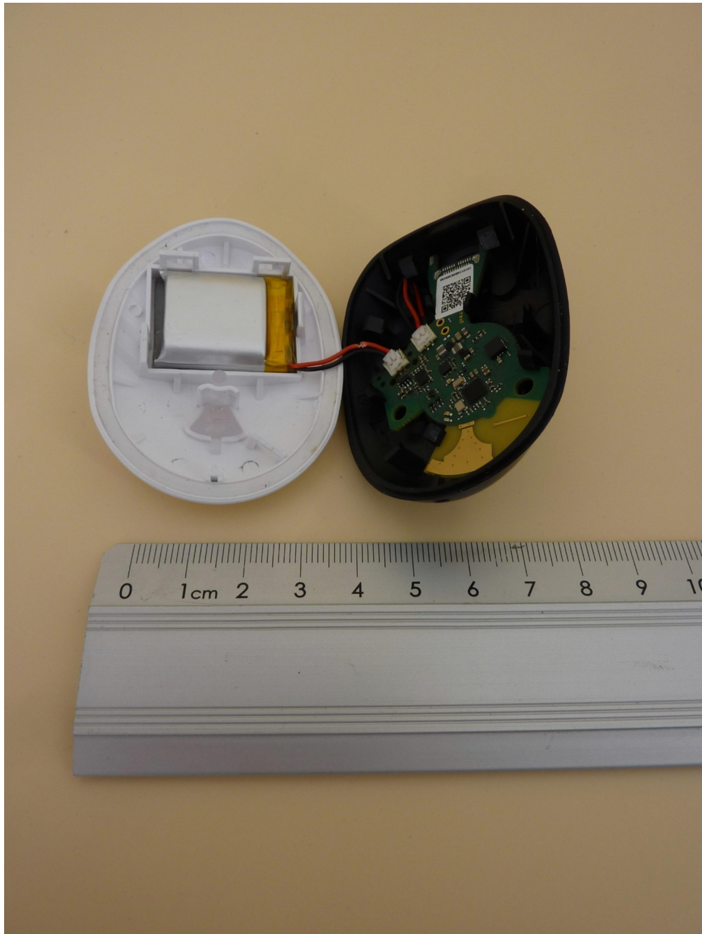
omlox WTag, internal view 1
