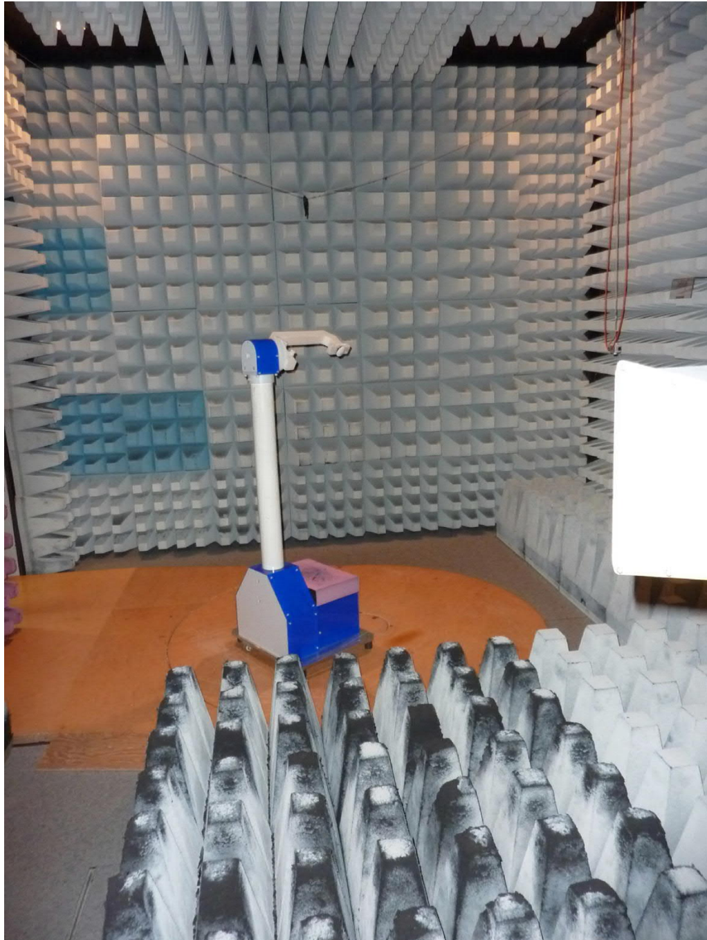
Test setup fully anechoic chamber spurious emissions from 1 GHz to 10.6 GHz
