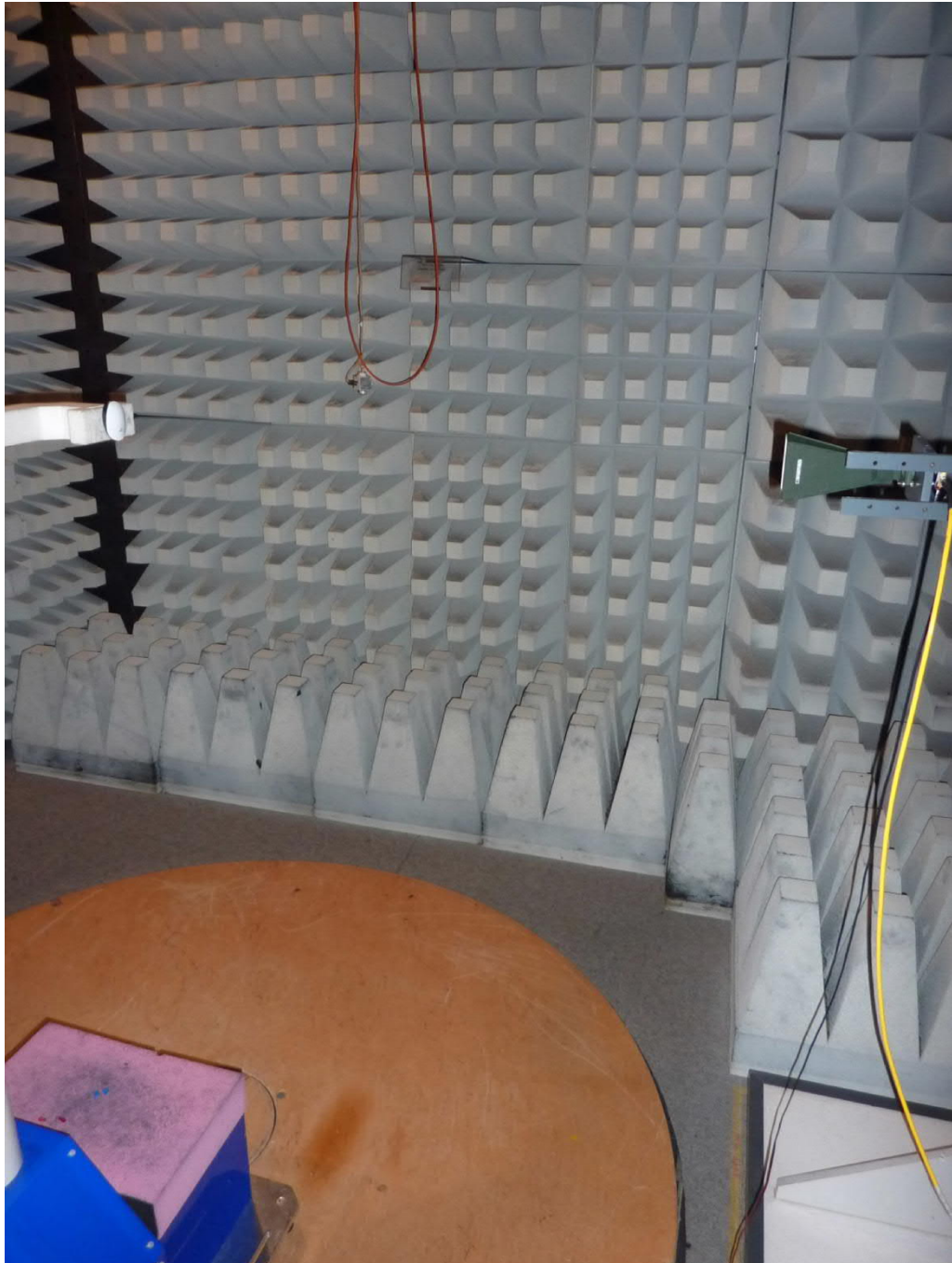
Test setup fully anechoic chamber spurious emissions above 10.6 GHz
