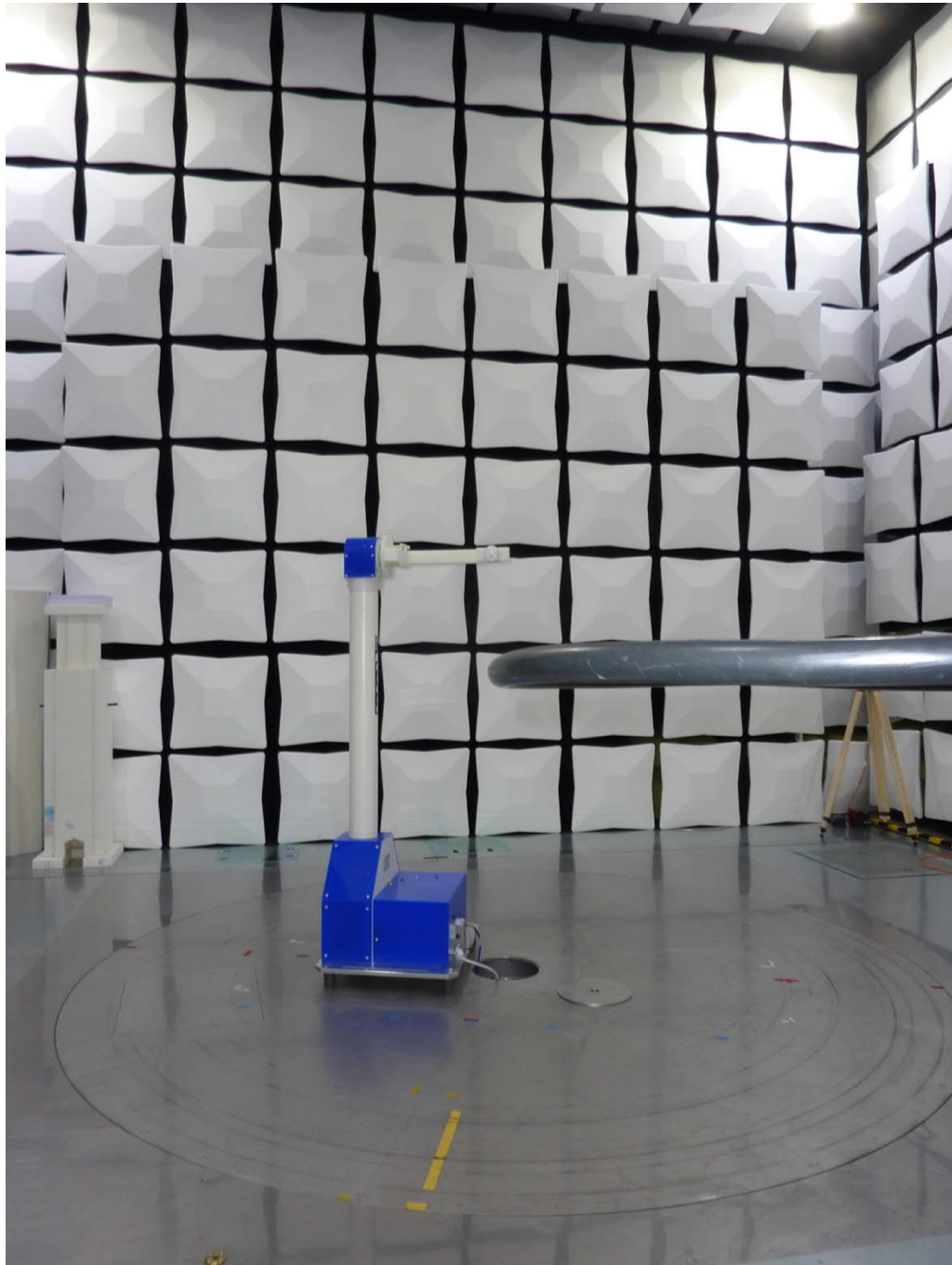
Test setup semi anechoic chamber spurious emissions from 150 kHz to 30 MHz
