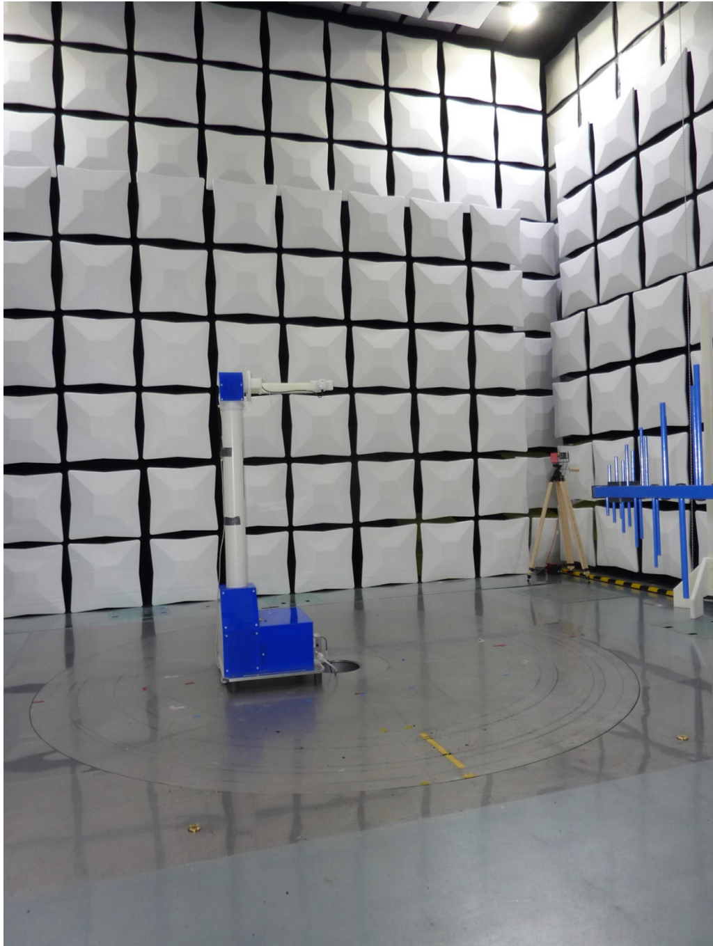
Test setup semi anechoic chamber spurious emissions from 30 MHz to 1 GHz
