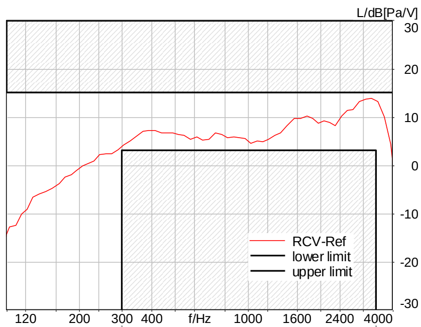
Figure C.3-26 – LTE Band 66 8N FF Narrowband Frequency Response
