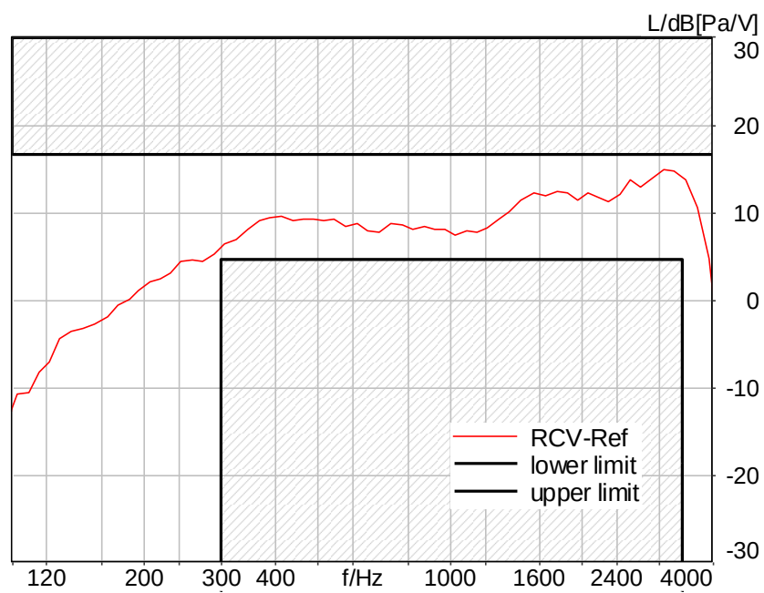
Figure C.3-18 – LTE Band 17 8N FF Narrowband Frequency Response
