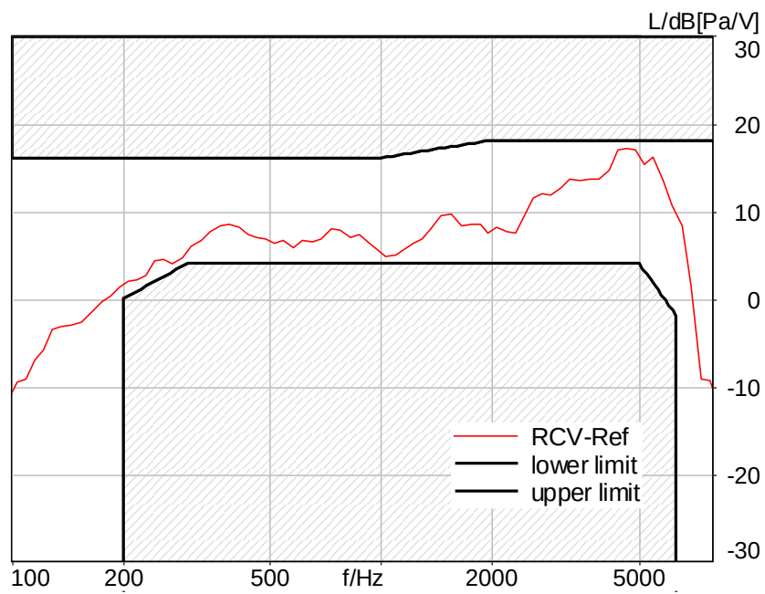
Figure C.3-23 – LTE Band 41 2N FF Wideband Frequency Response
