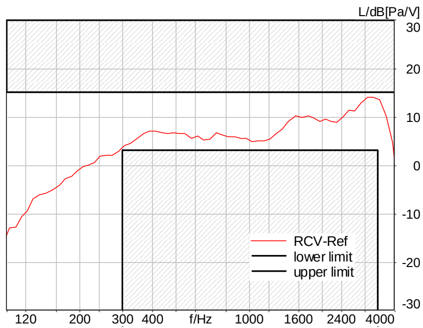
Figure C.3-17 – LTE Band 17 2N FF Narrowband Frequency Response
