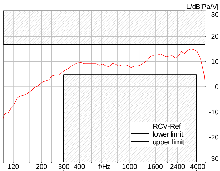
Figure C.3-30 – LTE Band 71 8N FF Narrowband Frequency Response
