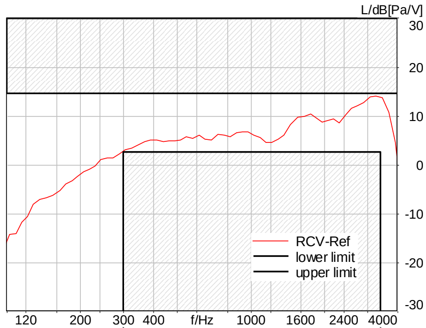
Figure C.1-1 – GSM850 2N FF Narrowband Frequency Response
