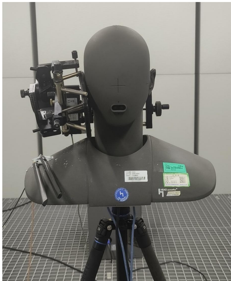
Figure E-1 – Test Layout (Handset)
