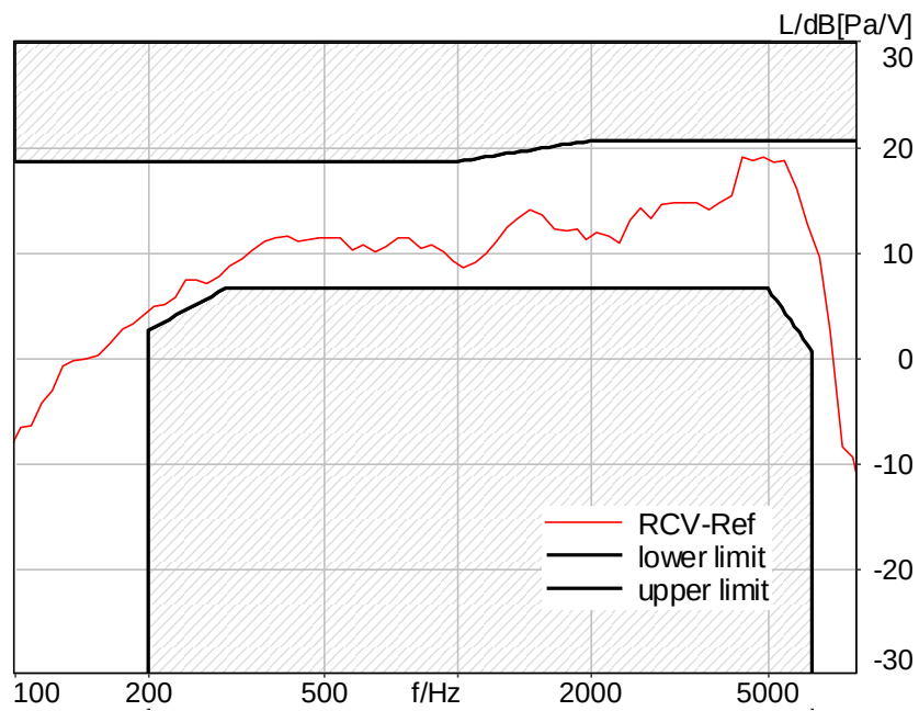
Figure C.3-20 – LTE Band 17 8N FF Wideband Frequency Response
