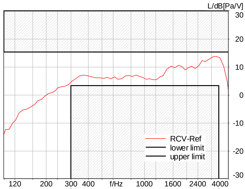
Figure C.3-21 – LTE Band 41 2N FF Narrowband Frequency Response
