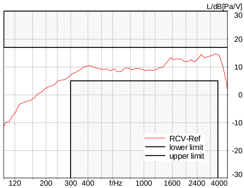
Figure C.3-22 – LTE Band 41 8N FF Narrowband Frequency Response
