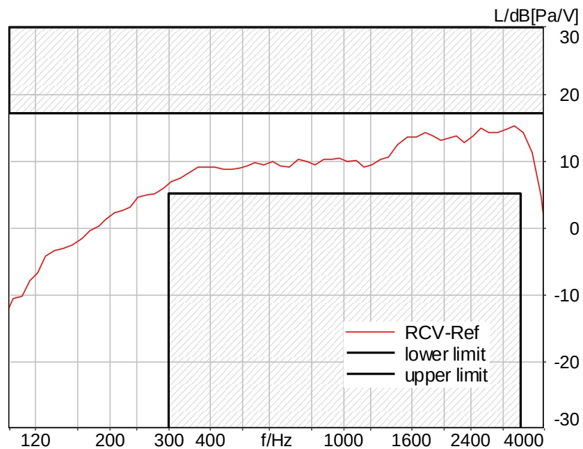
Figure C.1-2 – GSM850 8N FF Narrowband Frequency Response
