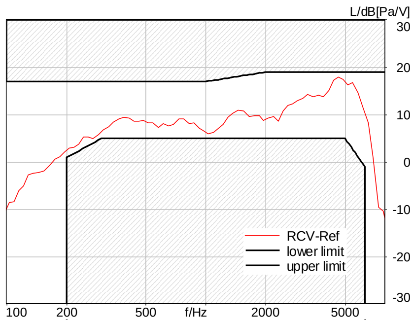
Figure C.3-31 – LTE Band 71 2N FF Wideband Frequency Response
