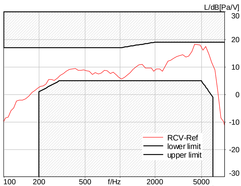
Figure C.3-28 – LTE Band 66 8N FF Wideband Frequency Response
