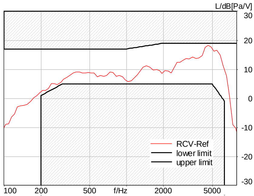
Figure C.3-19 – LTE Band 17 2N FF Wideband Frequency Response
