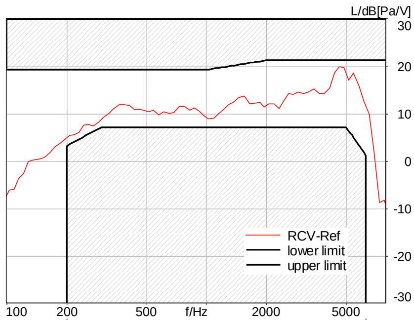
Figure C.3-24 – LTE Band 41 8N FF Wideband Frequency Response
