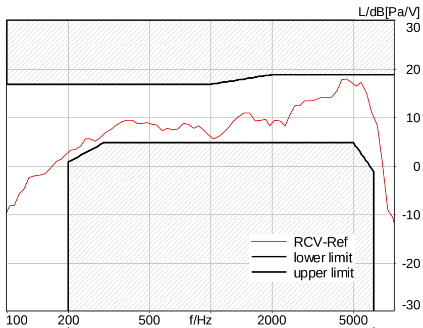
Figure C.3-27 – LTE Band 66 2N FF Wideband Frequency Response
