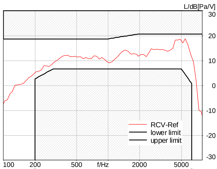
Figure C.3-32 – LTE Band 71 8N FF Wideband Frequency Response
