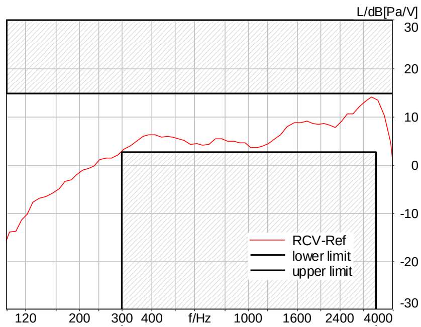
Figure C.3-25 – LTE Band 66 2N FF Narrowband Frequency Response
