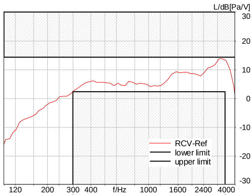
Figure C.3-29 – LTE Band 71 2N FF Narrowband Frequency Response
