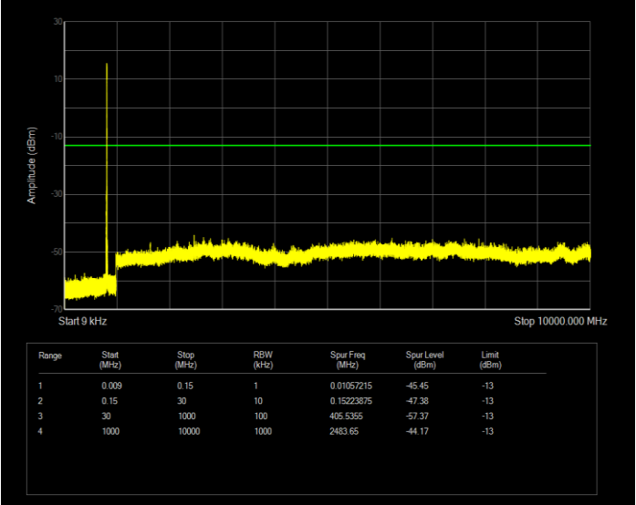
Band5 QAM16 BW=5MHz Channel=20425 RB Size=25 Position=#0
