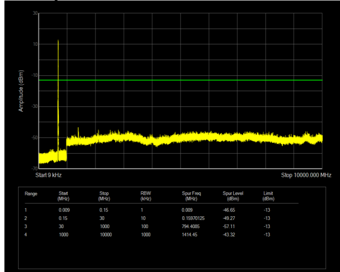
Band17 QAM16 BW=10MHz Channel=23780 RB Size=50 Position=#0
