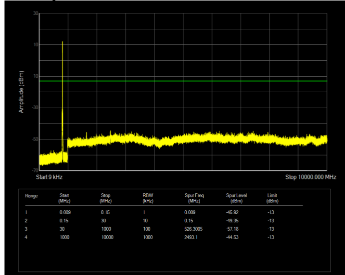
Band5 QAM16 BW=10MHz Channel=20450 RB Size=50 Position=#0
