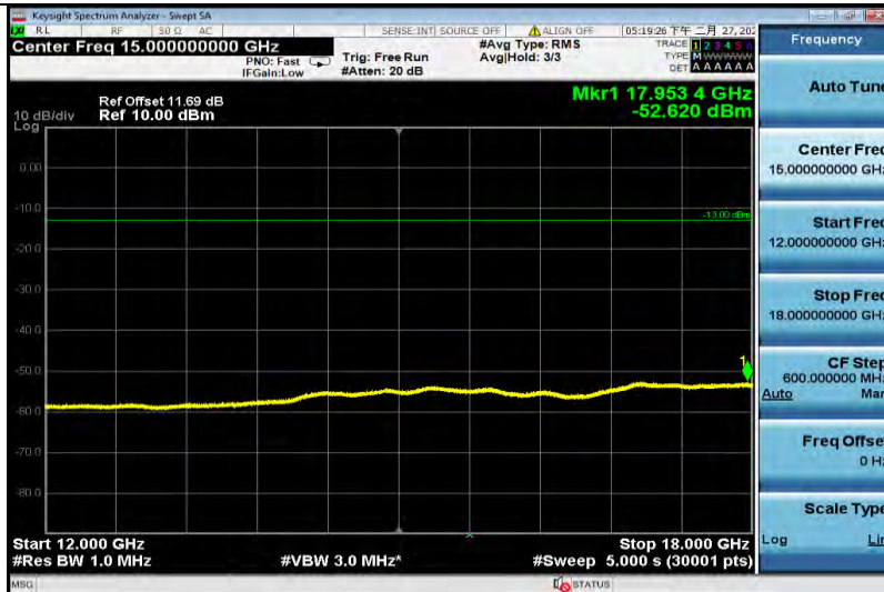
EGPRS850-128-12000~18000
