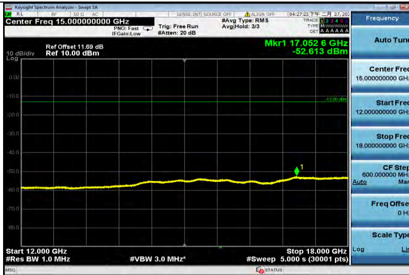
GPRS850-128-12000~18000
