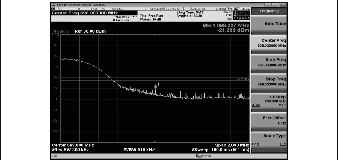
Band71-20MHz-QPSK-133222-100RB#0
