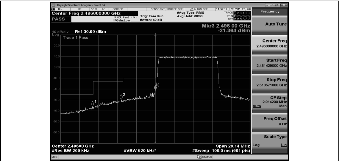
Band41-10MHz-QPSK-40620-50RB#0
