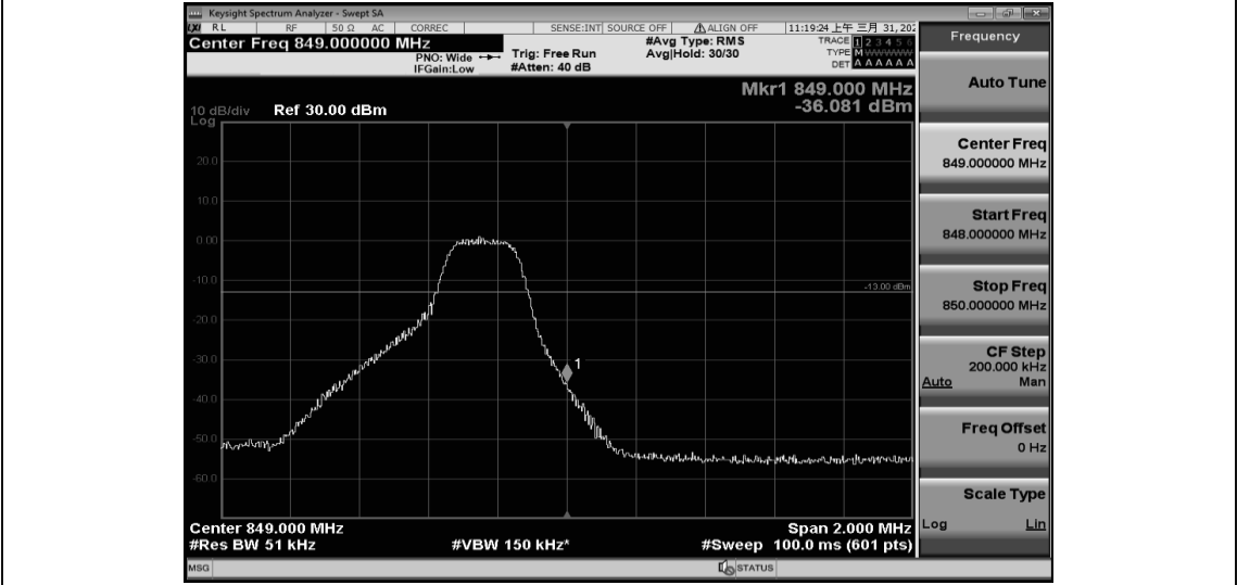
Band26-3MHz-16QAM-27025-15RB#0
