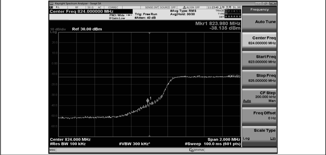
Band26-5MHz-16QAM-26915-1RB#24
