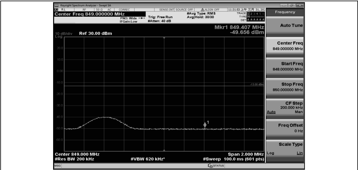
Band26-10MHz-QPSK-26990-1RB#49
