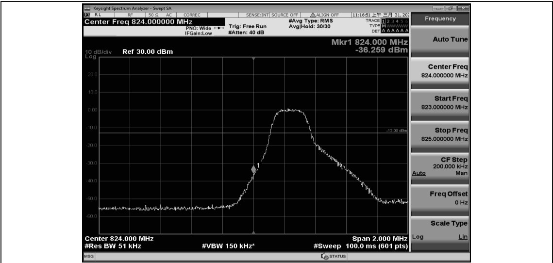
Band26-3MHz-16QAM-26805-1RB#14
