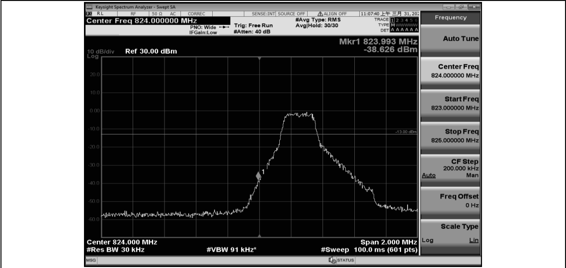
Band26-1.4MHz-16QAM-26797-6RB#0
