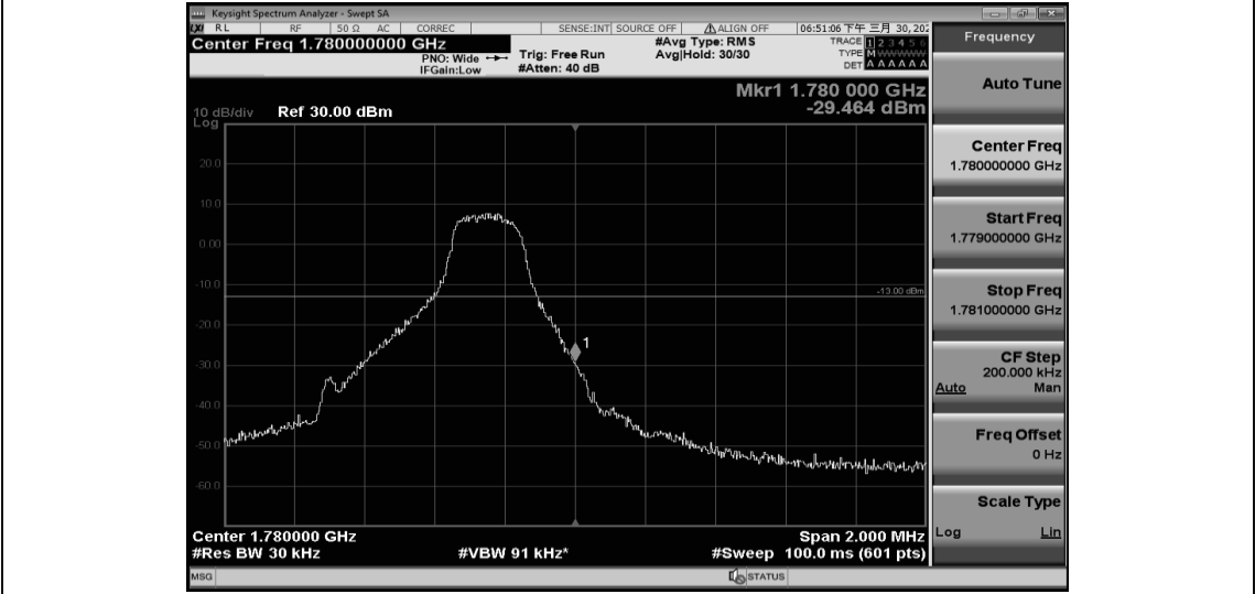
Band66-1.4MHz-QPSK-132665-6RB#0
