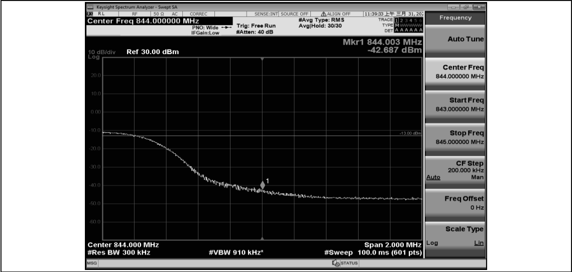
Band26-15MHz-QPSK-26965-1RB#74
