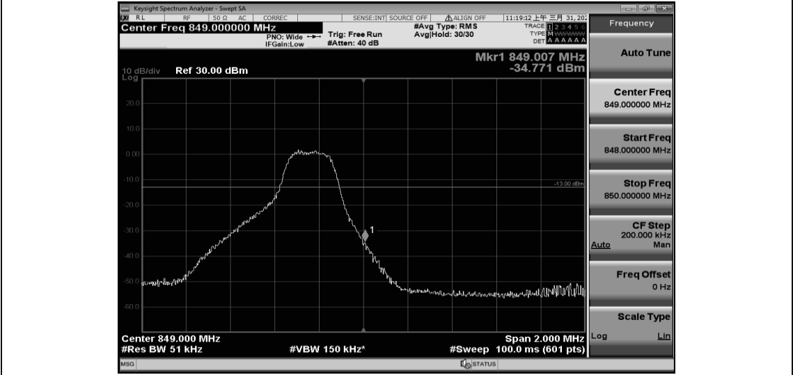
Band26-3MHz-QPSK-27025-15RB#0
