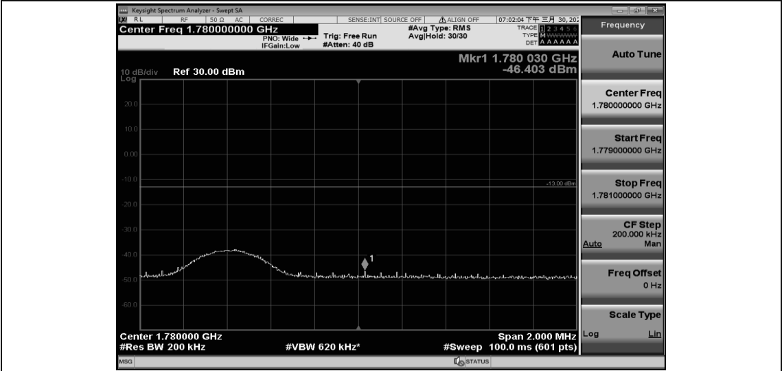
Band66-10MHz-QPSK-132622-1RB#49
