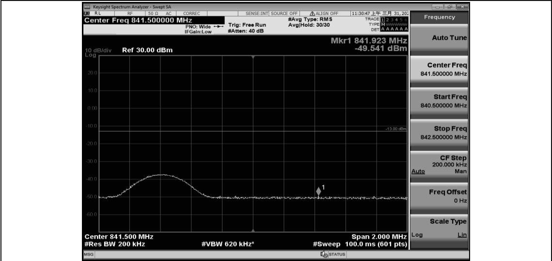
Band26-10MHz-QPSK-26915-50RB#0
