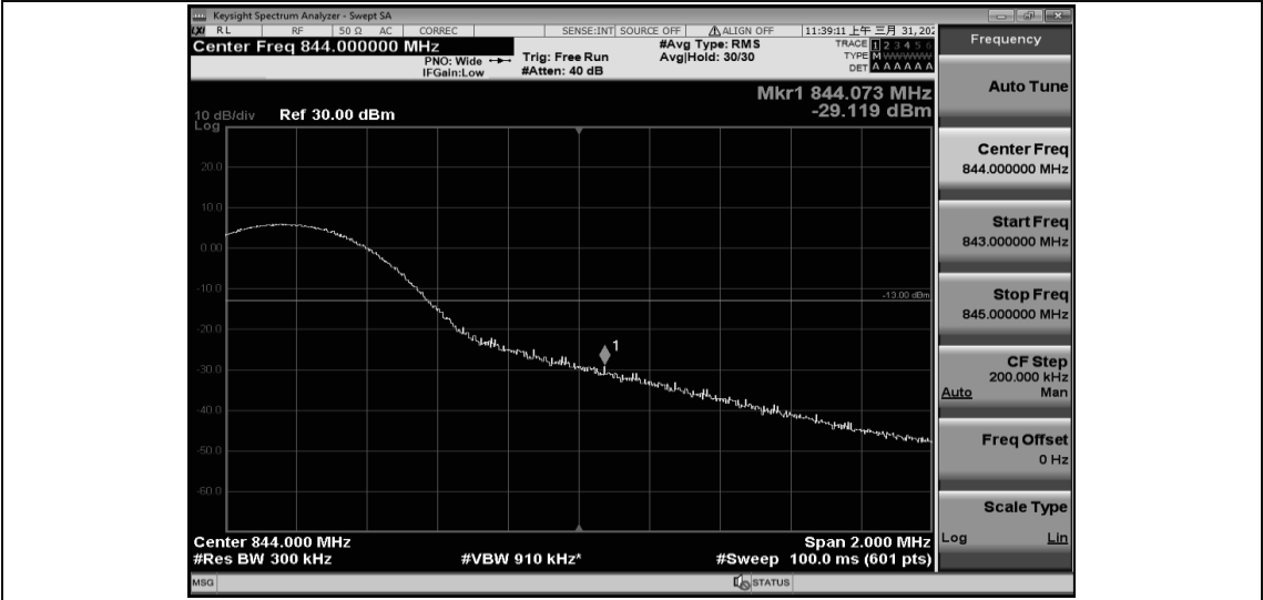
Band26-15MHz-QPSK-26915-75RB#0
