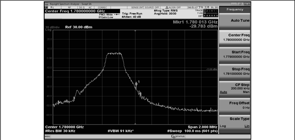
Band66-1.4MHz-16QAM-132665-1RB#0
