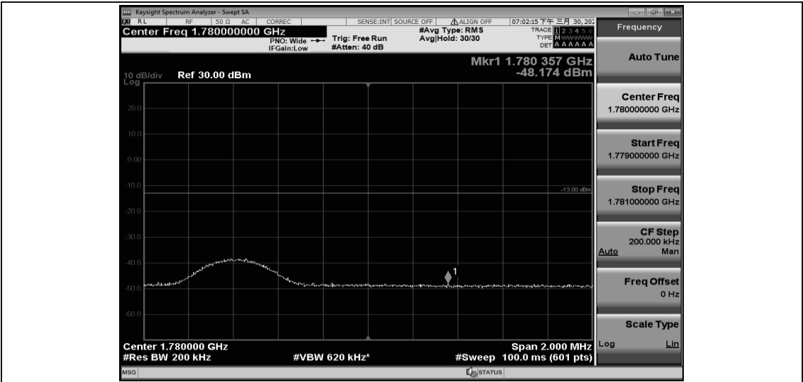
Band66-10MHz-16QAM-132622-1RB#49
