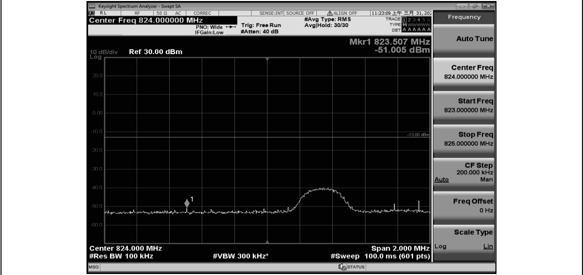
Band26-5MHz-QPSK-26815-25RB#0
