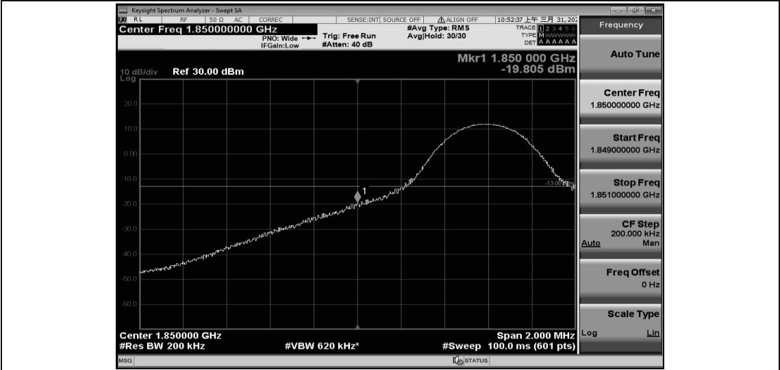
Band25-10MHz-QPSK-26090-1RB#49
