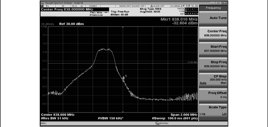
Band26-3MHz-16QAM-26915-15RB#0
