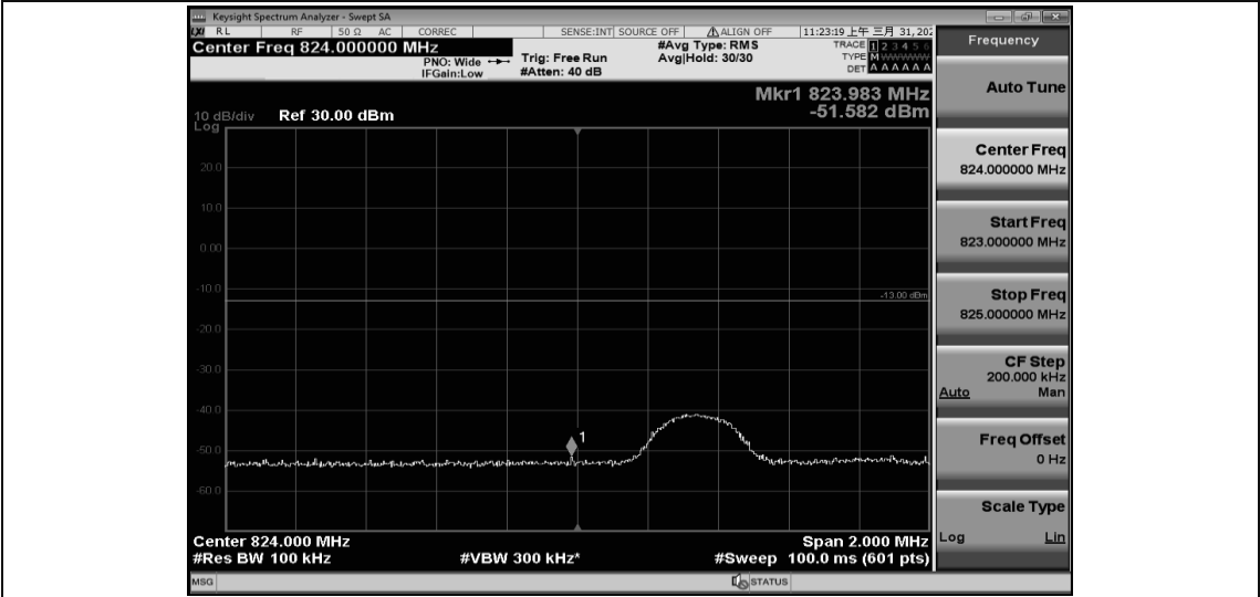
Band26-5MHz-16QAM-26815-1RB#0
