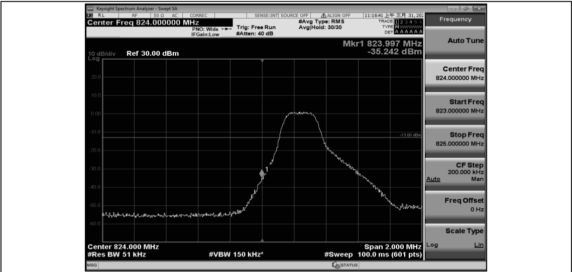
Band26-3MHz-QPSK-26805-1RB#14
