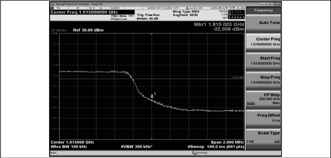
Band25-10MHz-QPSK-26090-1RB#0
