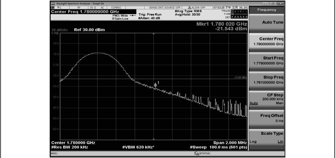
Band66-10MHz-QPSK-132622-50RB#0
