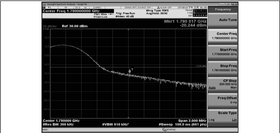
Band66-15MHz-QPSK-132597-1RB#0
