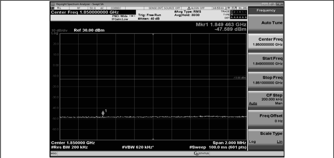
Band25-10MHz-16QAM-26090-50RB#0
