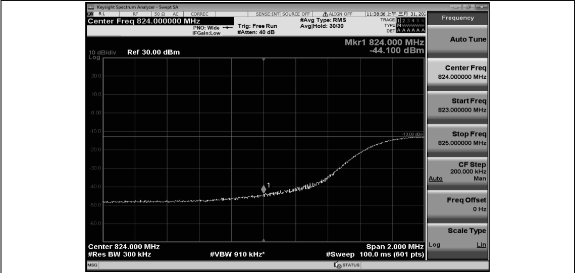
Band26-15MHz-16QAM-26915-1RB#74
