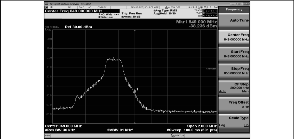
Band26-1.4MHz-16QAM-27033-1RB#0
