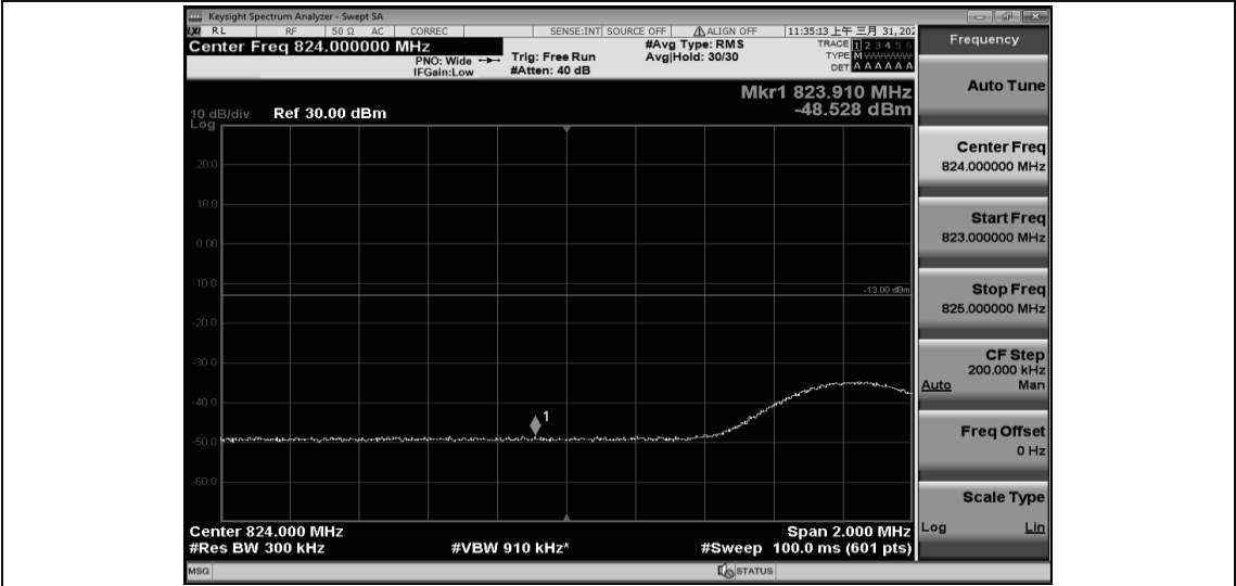
Band26-15MHz-16QAM-26865-1RB#0
