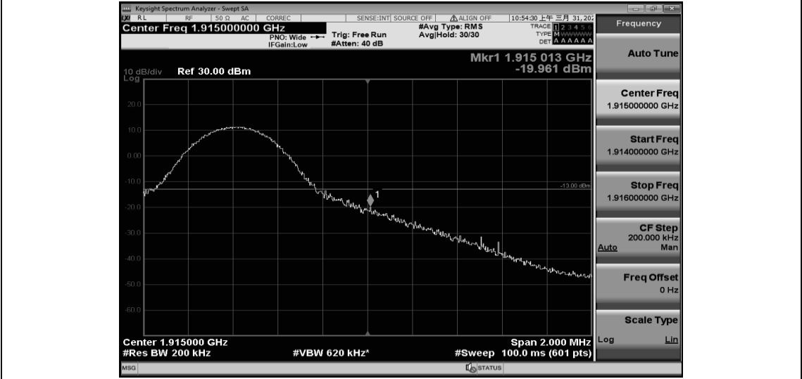
Band25-10MHz-16QAM-26640-50RB#0
