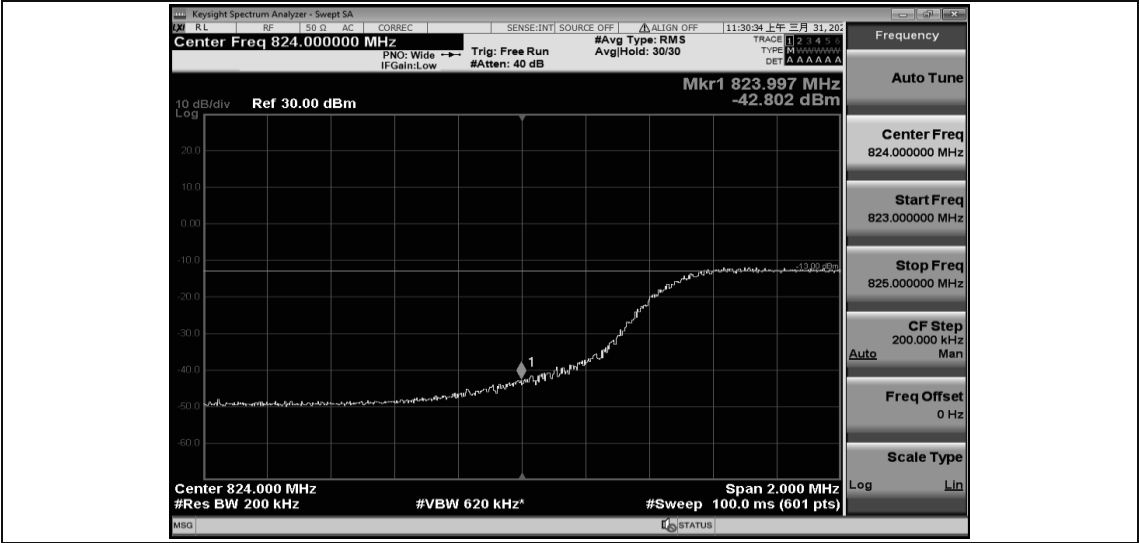
Band26-10MHz-16QAM-26915-1RB#0
