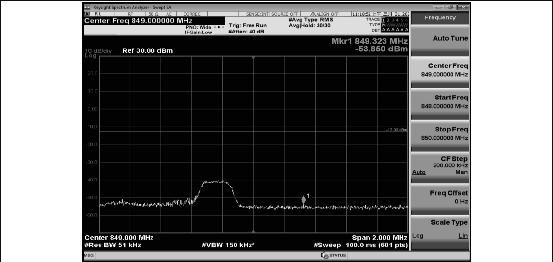
Band26-3MHz-QPSK-27025-1RB#14
