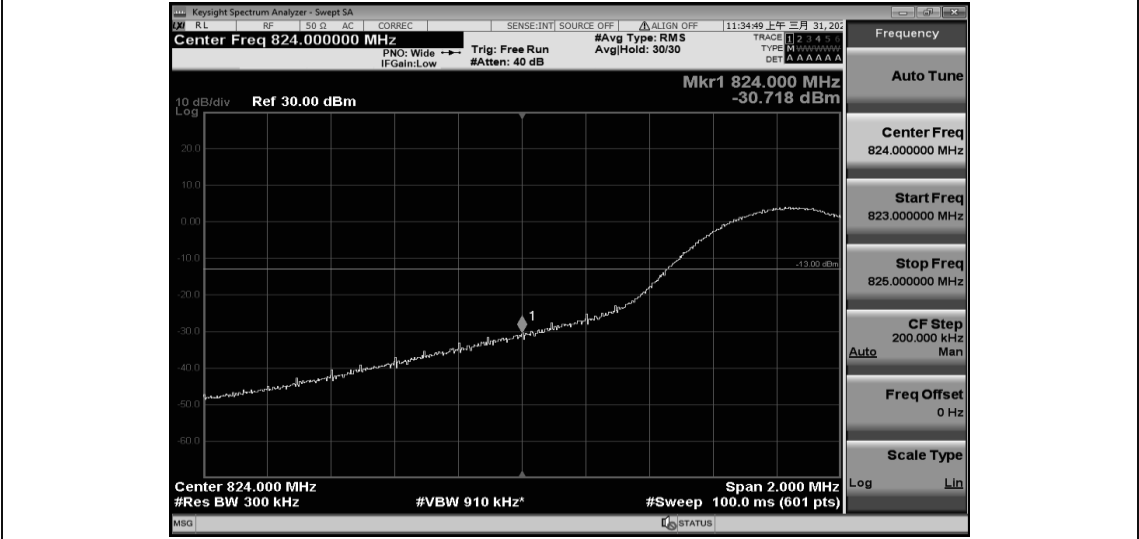
Band26-15MHz-16QAM-26865-75RB#0
