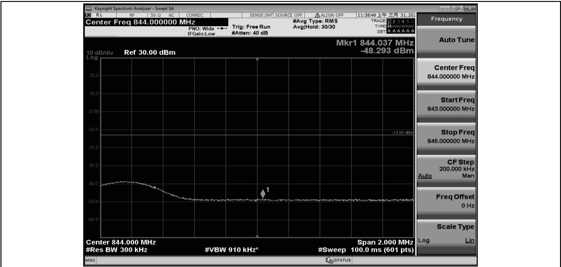
Band26-15MHz-QPSK-26915-1RB#74
