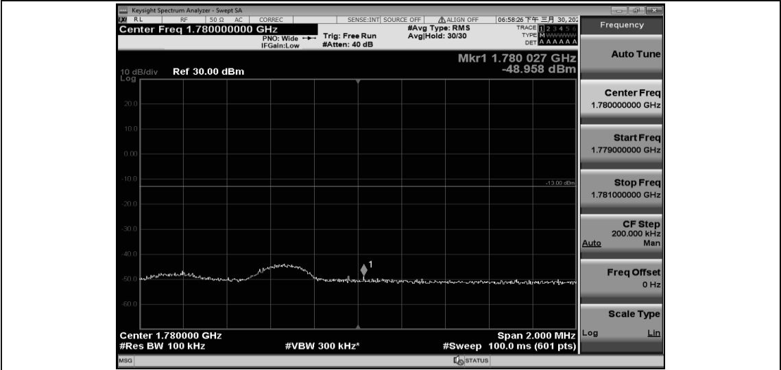
Band66-5MHz-QPSK-132647-1RB#24
