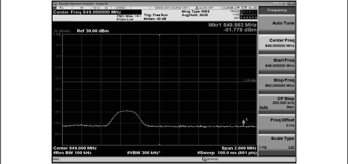
Band26-5MHz-QPSK-27015-25RB#0
