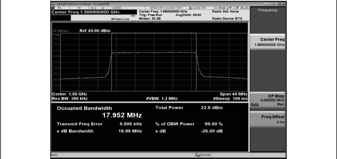
Band2-20MHz-16QAM-19100-100RB#0-17.979
