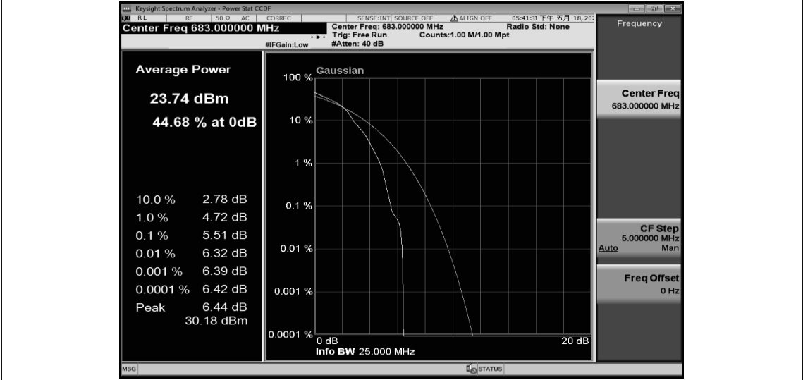
Band71-20MHz-16QAM-133322-100RB#0
