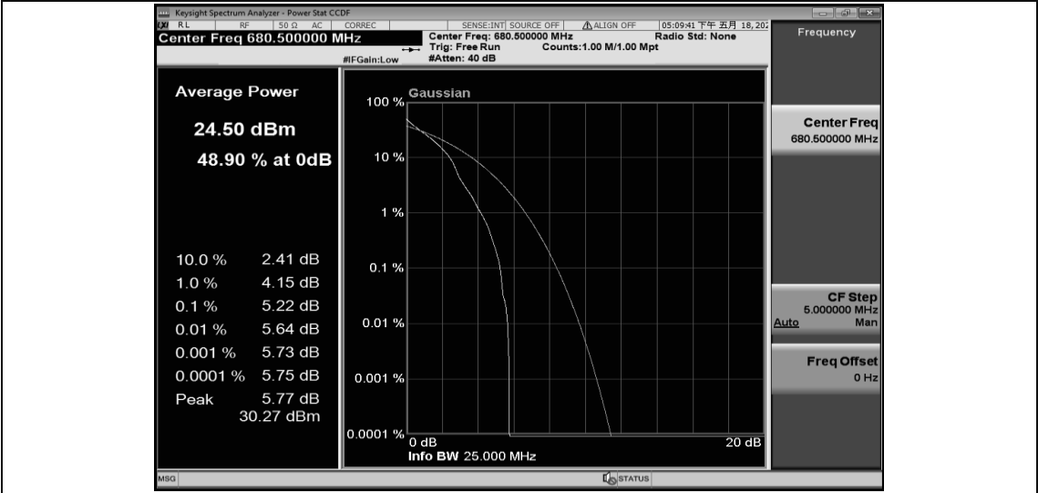
Band71-15MHz-QPSK-133297-75RB#0
