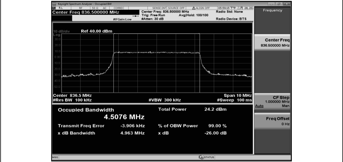
Band5-5MHz-16QAM-20625-25RB#0-9.9051
