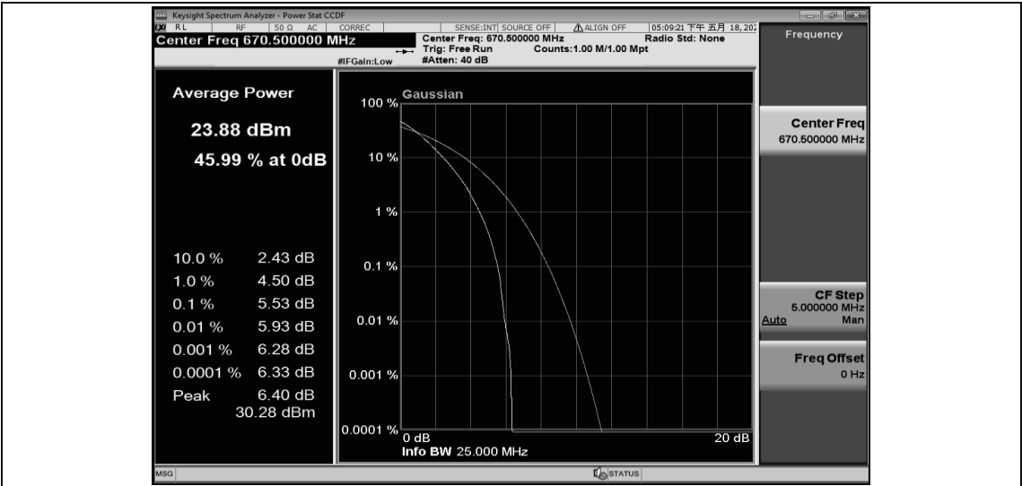
Band71-15MHz-QPSK-133297-1RB#0
