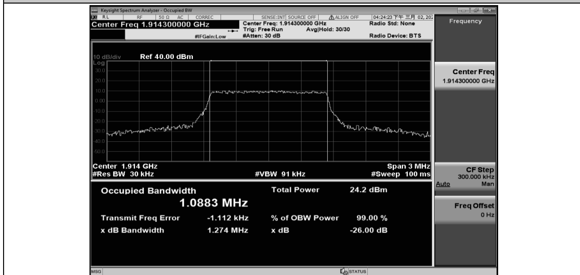
Band25-3MHz-QPSK-26055-15RB#0-2.6884
