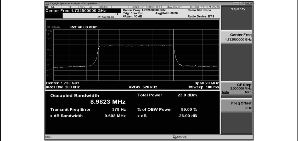
Band4-10MHz-16QAM-20350-50RB#0-8.9864
