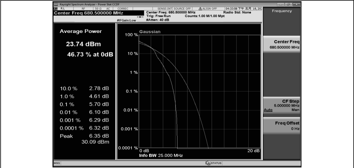
Band71-10MHz-16QAM-133297-50RB#0
