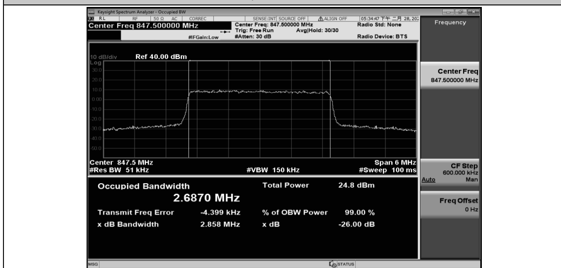
Band5-3MHz-16QAM-20415-15RB#0-2.6870
