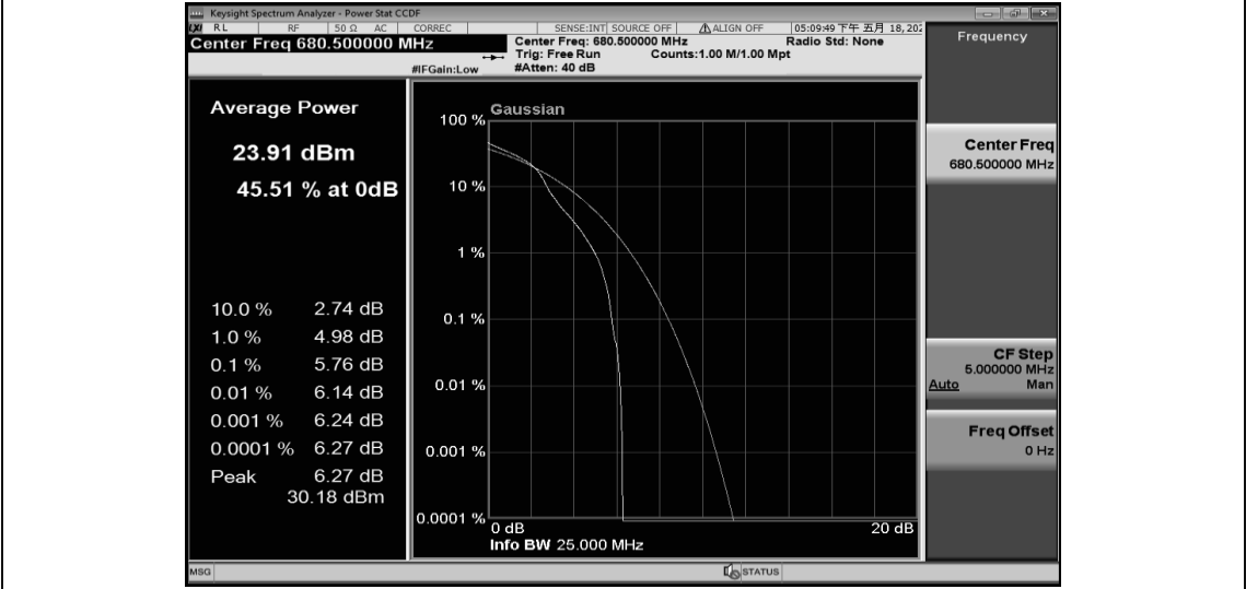
Band71-15MHz-16QAM-133297-75RB#0
