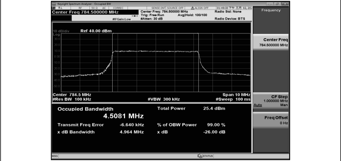
Band13-5MHz-16QAM-23205-25RB#0-4.5031
