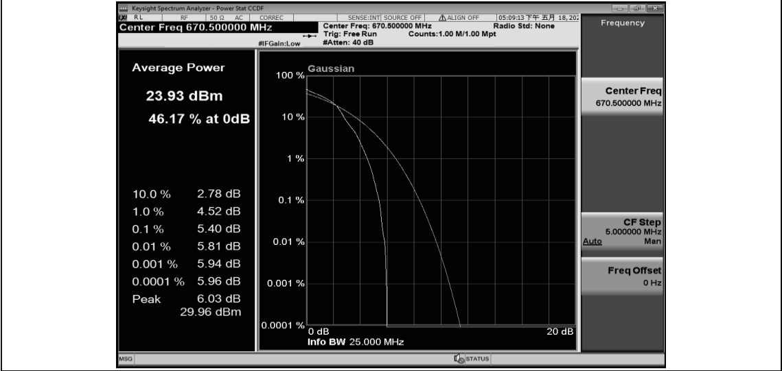
Band71-15MHz-16QAM-133197-75RB#0
