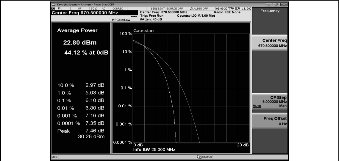
Band71-15MHz-16QAM-133297-1RB#0
