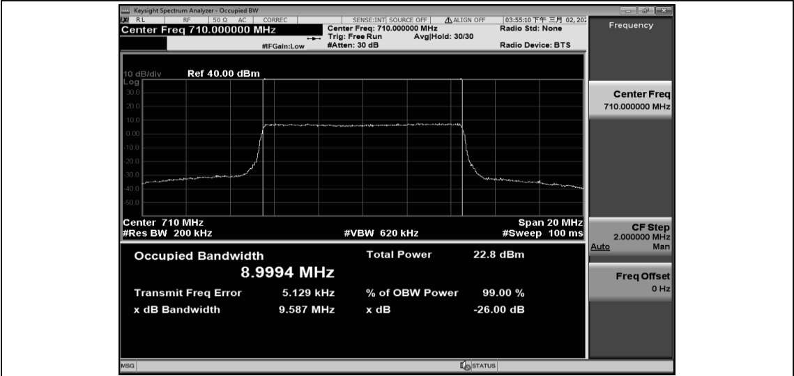
Band17-10MHz-16QAM-23800-50RB#0-8.9835
