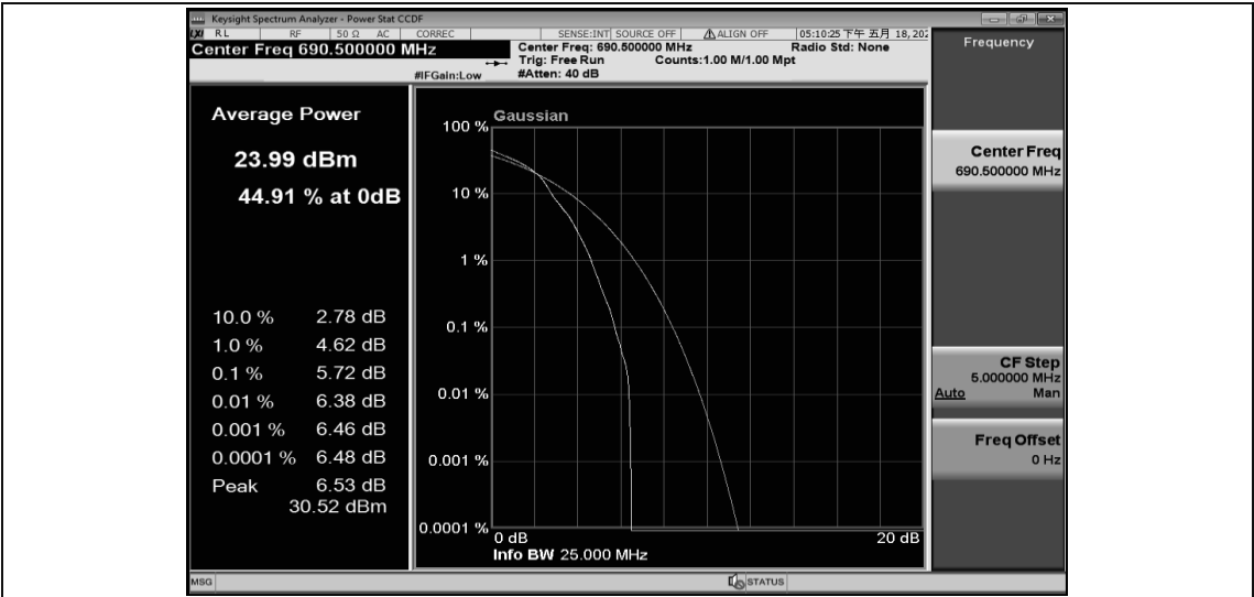
Band71-15MHz-16QAM-133397-75RB#0
