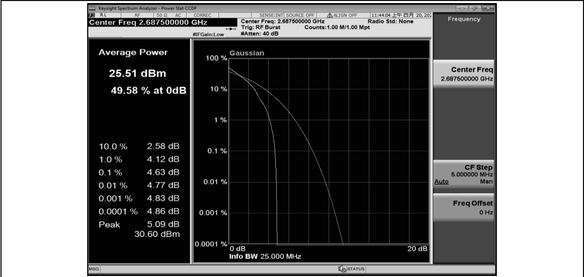
Band41-5MHz-QPSK-41565-25RB#0
