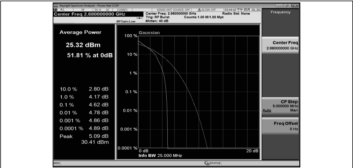
Band41-20MHz-QPSK-41490-100RB#0
