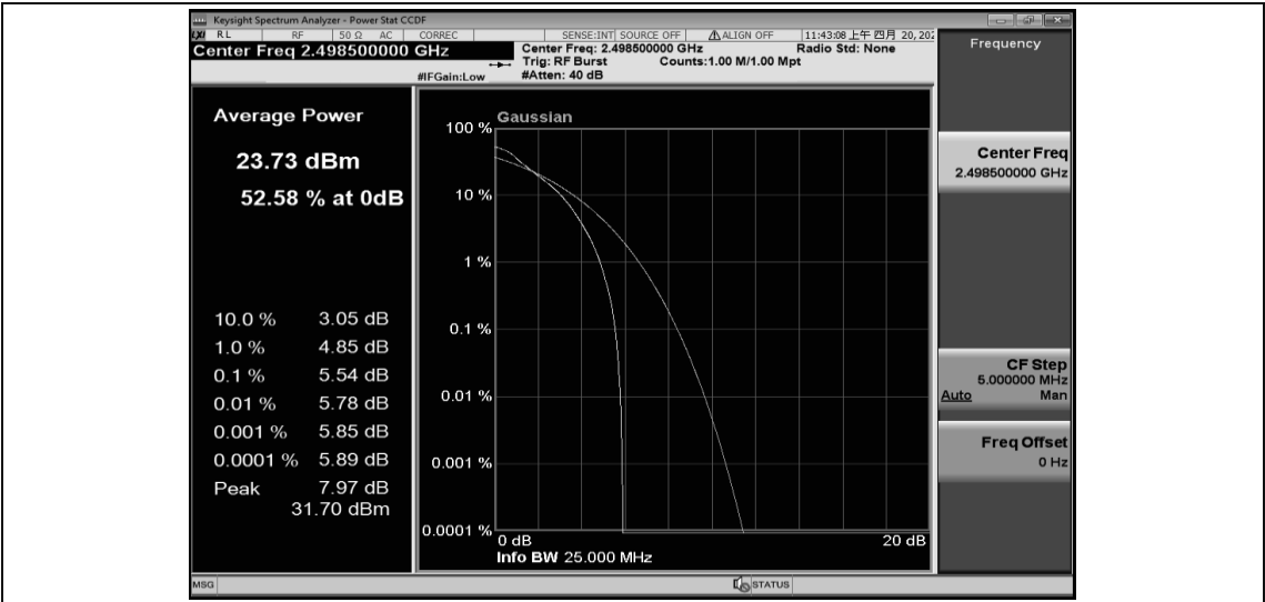
Band41-5MHz-QPSK-40620-1RB#0
