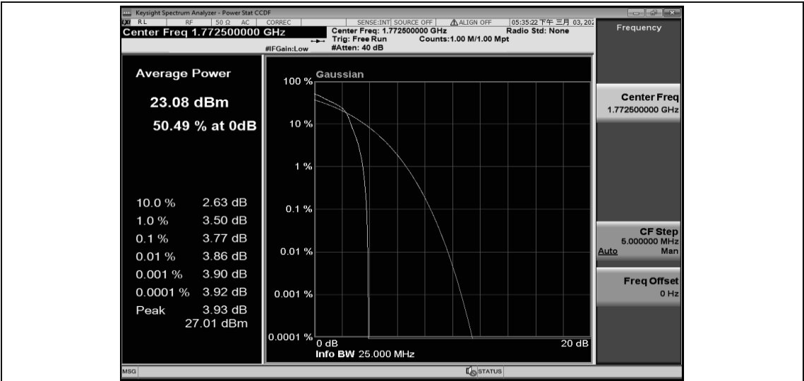
Band66-15MHz-16QAM-132597-75RB#0
