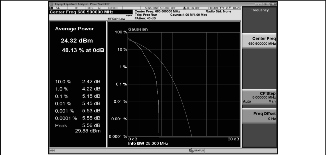
Band71-10MHz-QPSK-133297-50RB#0
