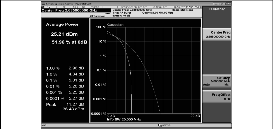
Band41-10MHz-QPSK-41540-50RB#0
