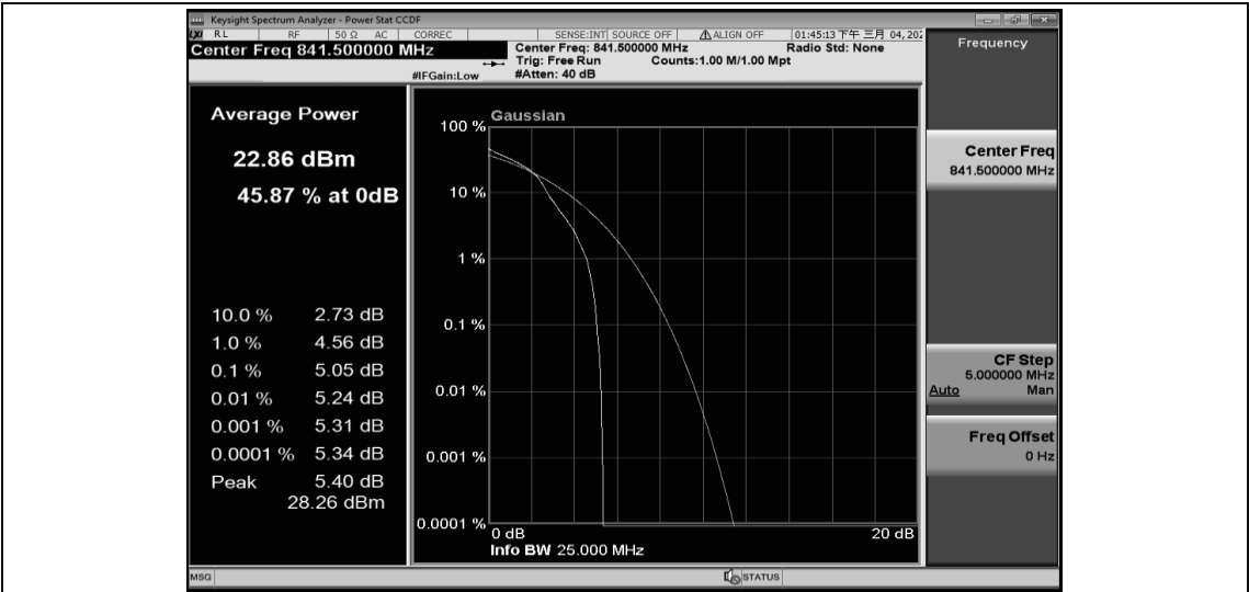
Band26-15MHz-16QAM-26965-75RB#0
