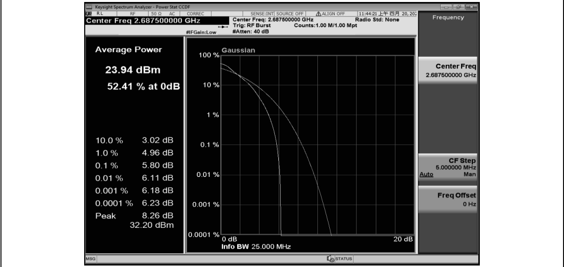
Band41-5MHz-16QAM-39675-1RB#0
