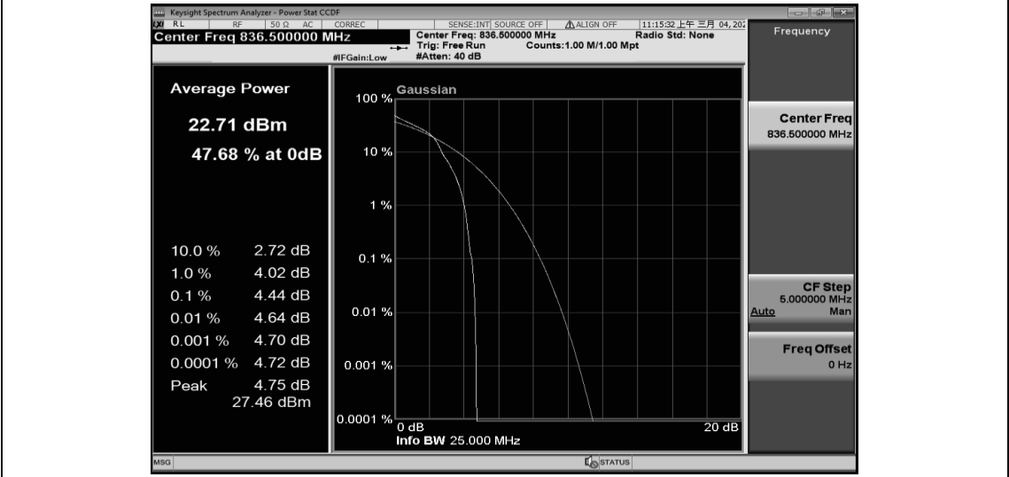
Band26-5MHz-16QAM-26915-25RB#0
