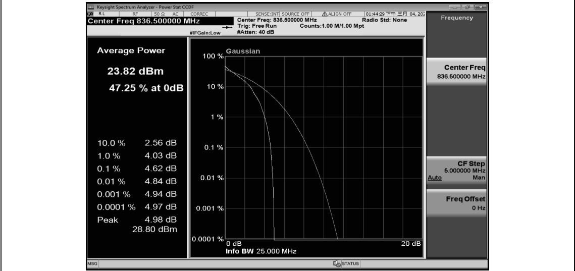
Band26-15MHz-QPSK-26915-75RB#0
