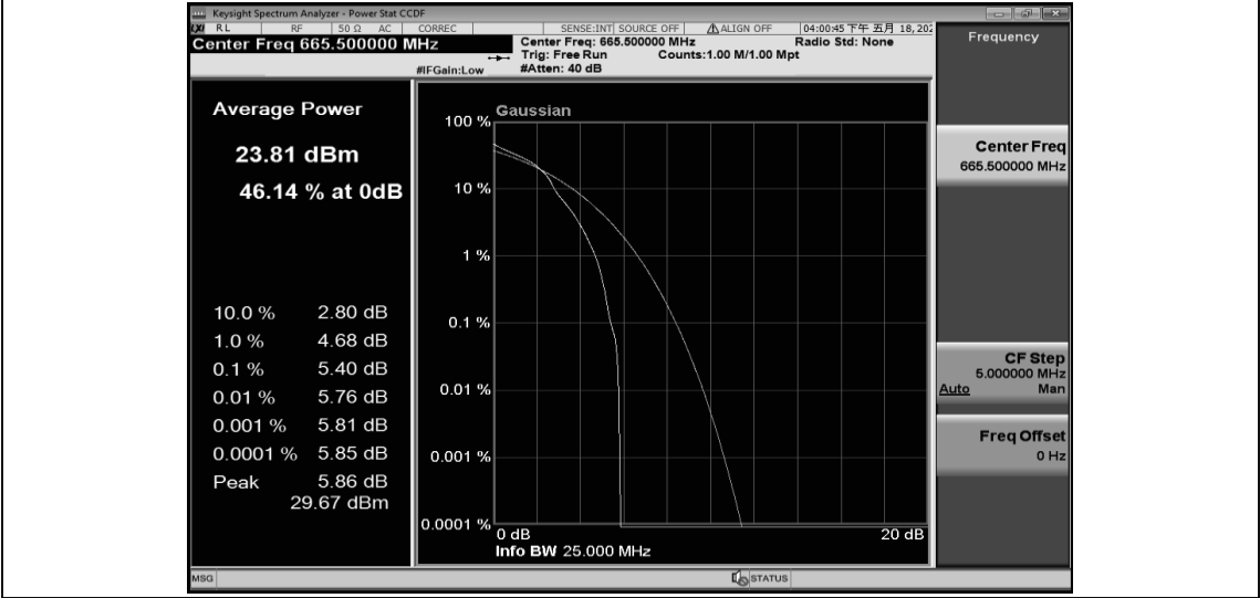
Band71-5MHz-16QAM-133147-25RB#0
