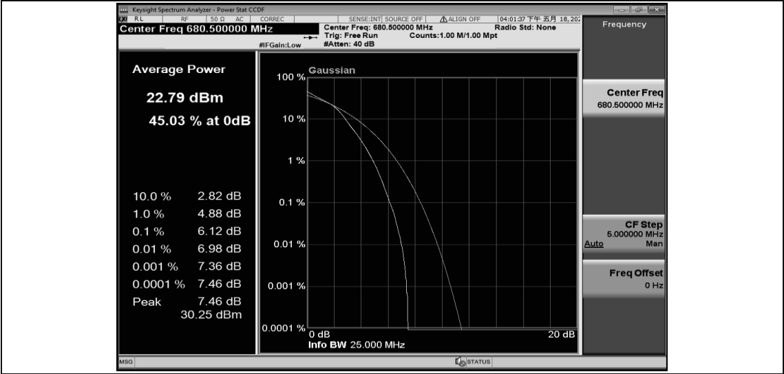
Band71-5MHz-16QAM-133447-1RB#0
