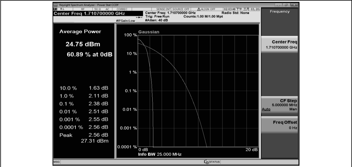
Band66-1.4MHz-QPSK-131979-6RB#0
