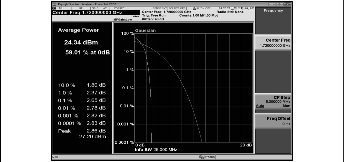
Band66-20MHz-QPSK-132072-100RB#0
