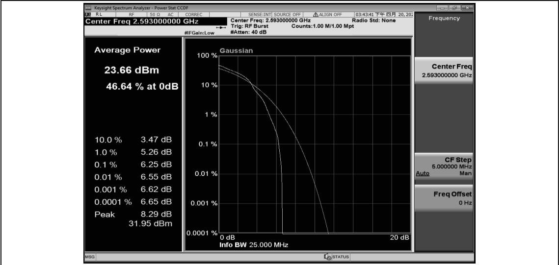
Band41-20MHz-16QAM-40620-100RB#0
