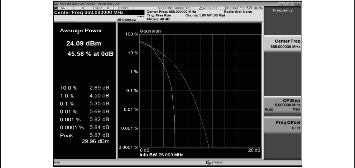
Band71-10MHz-16QAM-133172-50RB#0
