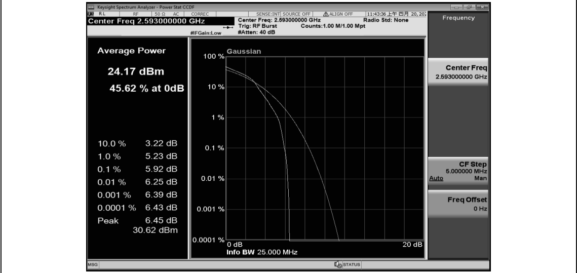
Band41-5MHz-16QAM-40620-25RB#0
