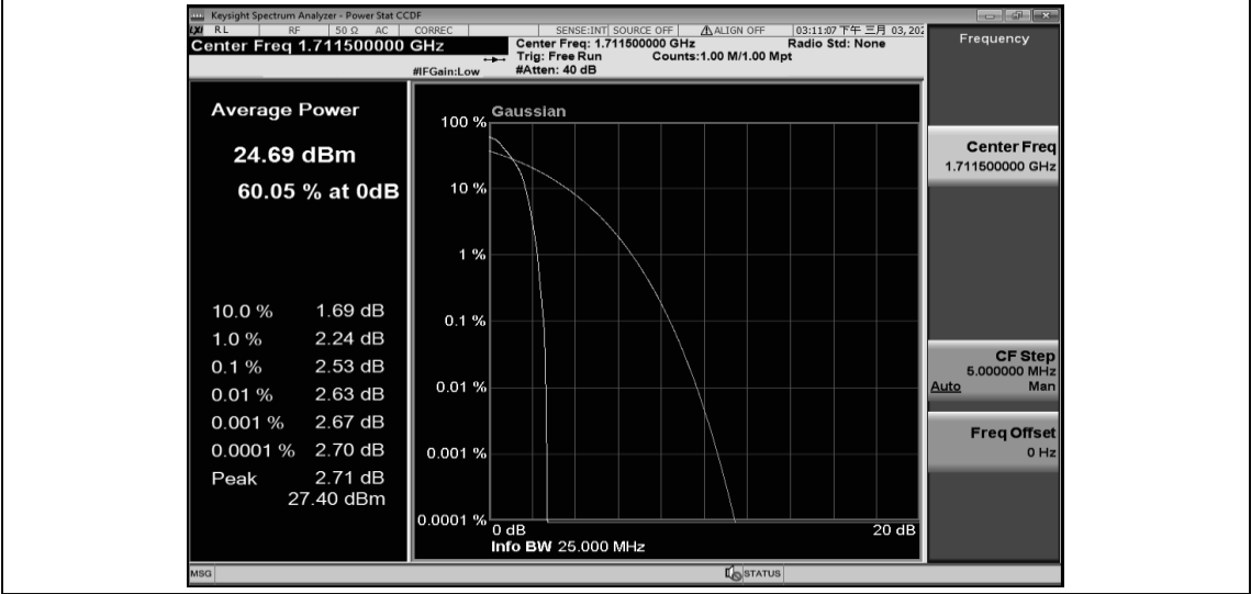
Band66-3MHz-QPSK-131987-15RB#0
