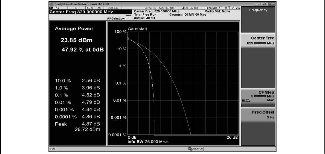
Band26-10MHz-QPSK-26840-50RB#0
