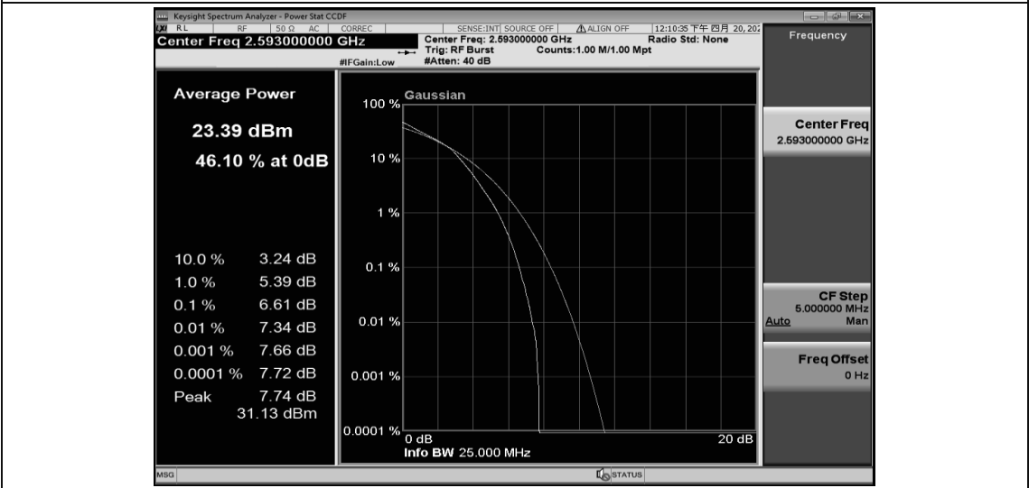
Band41-10MHz-16QAM-41540-1RB#0
