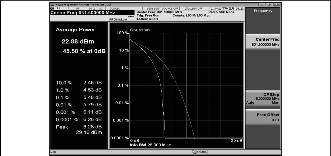
Band26-15MHz-QPSK-26915-1RB#0
