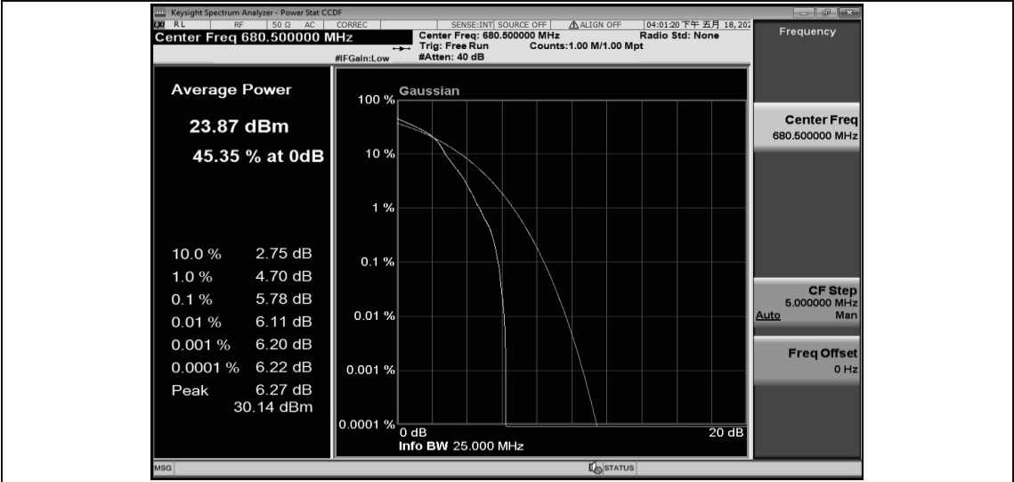
Band71-5MHz-16QAM-133297-25RB#0
