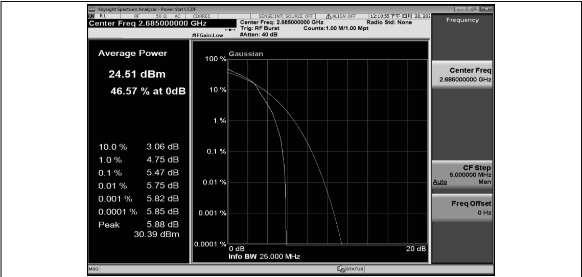
Band41-10MHz-16QAM-41540-50RB#0
