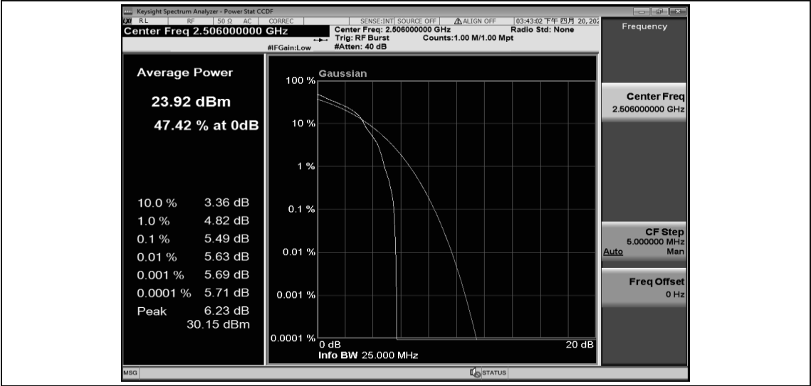
Band41-20MHz-16QAM-39750-100RB#0
