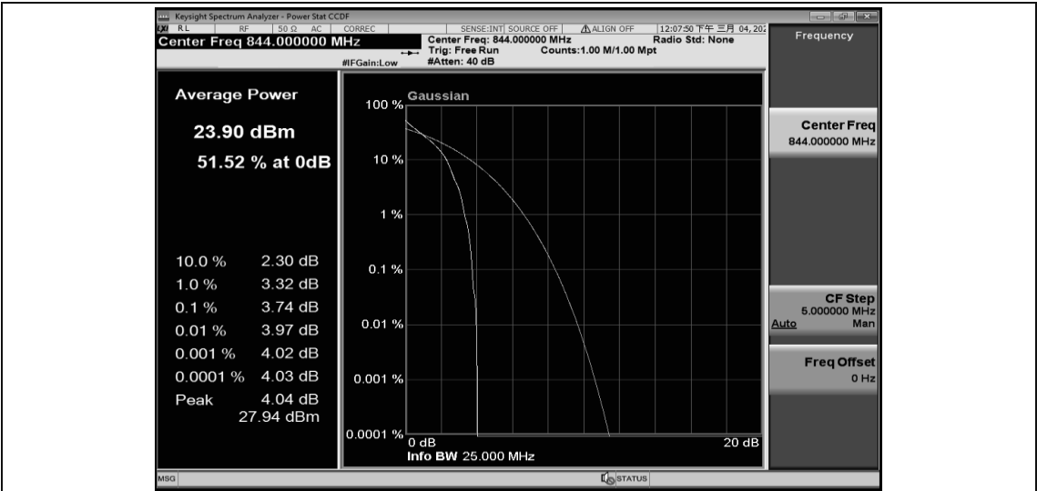
Band26-10MHz-QPSK-26990-50RB#0
