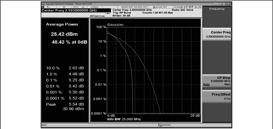
Band41-5MHz-QPSK-40620-25RB#0
