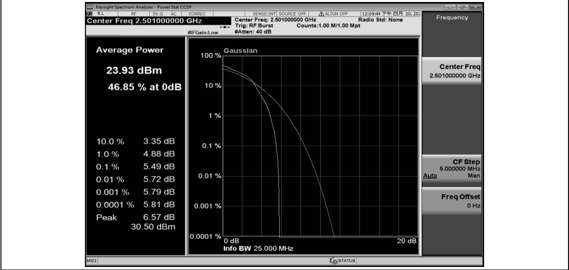
Band41-10MHz-16QAM-39700-50RB#0
