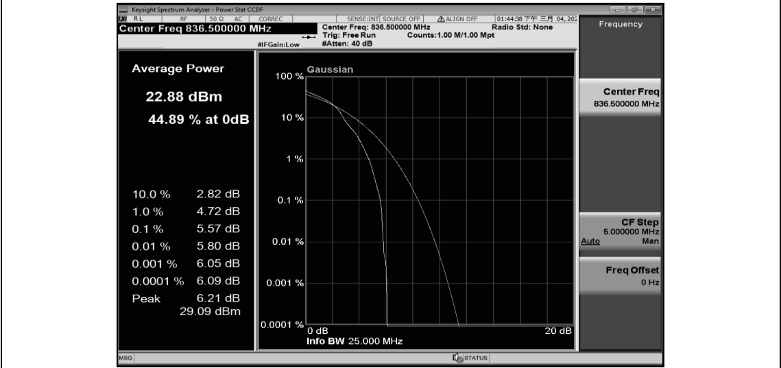
Band26-15MHz-16QAM-26915-75RB#0
