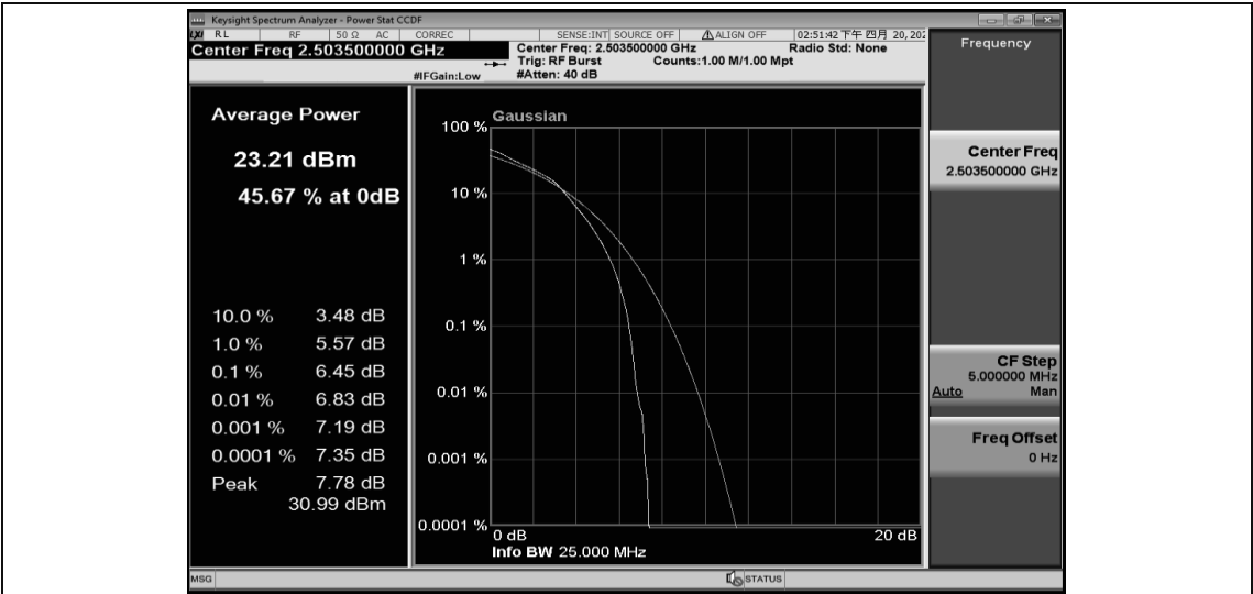
Band41-15MHz-16QAM-40620-1RB#0
