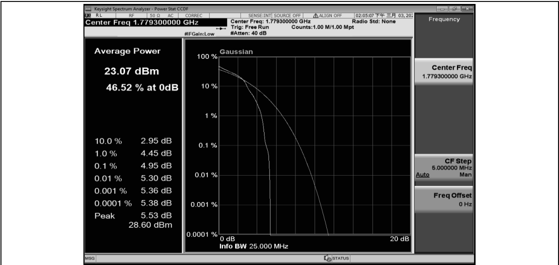
Band66-1.4MHz-16QAM-132665-6RB#0
