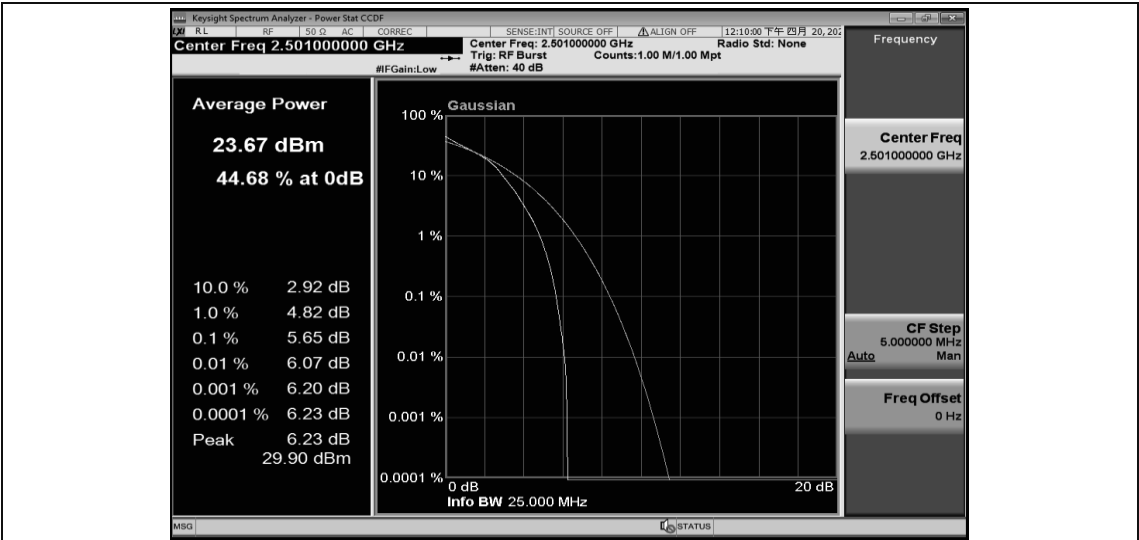
Band41-10MHz-16QAM-40620-1RB#0
