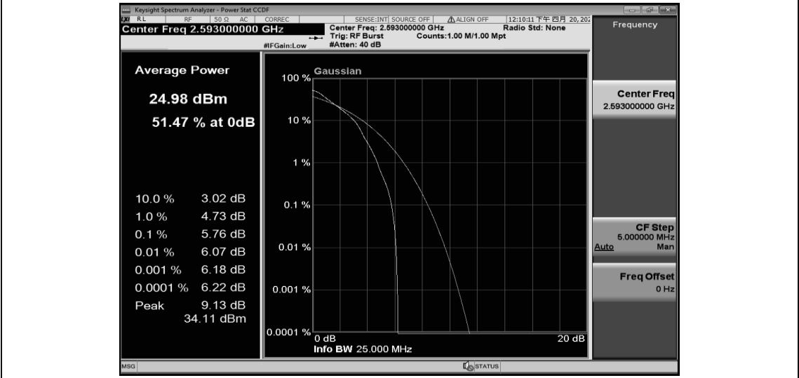
Band41-10MHz-QPSK-40620-50RB#0
