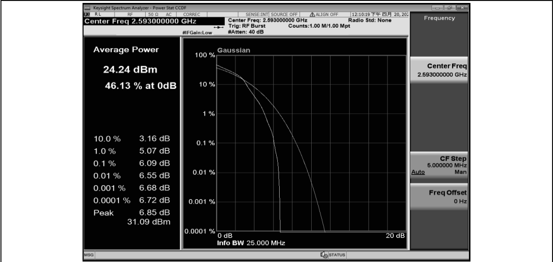
Band41-10MHz-16QAM-40620-50RB#0
