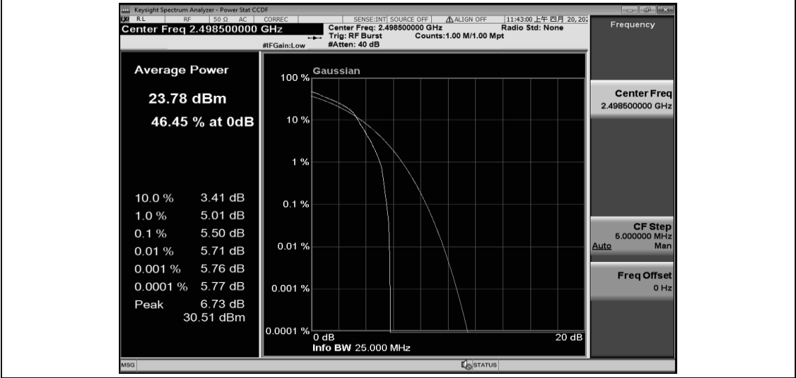
Band41-5MHz-16QAM-39675-25RB#0
