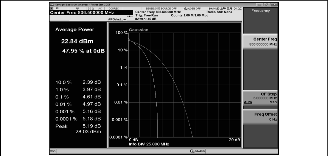
Band26-3MHz-QPSK-27025-1RB#0
