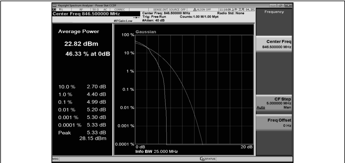
Band26-5MHz-16QAM-27015-25RB#0
