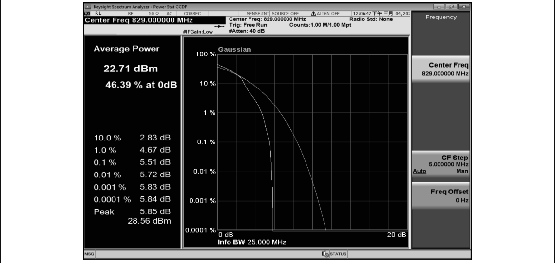
Band26-10MHz-16QAM-26840-50RB#0
