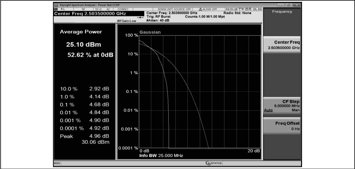
Band41-15MHz-QPSK-39725-75RB#0
