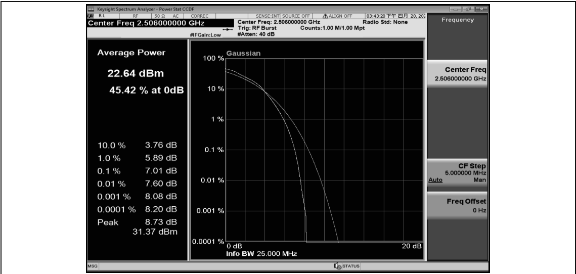
Band41-20MHz-16QAM-40620-1RB#0
