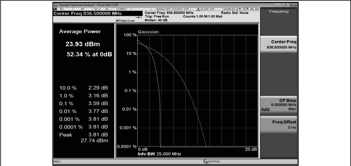
Band26-3MHz-QPSK-26915-15RB#0
