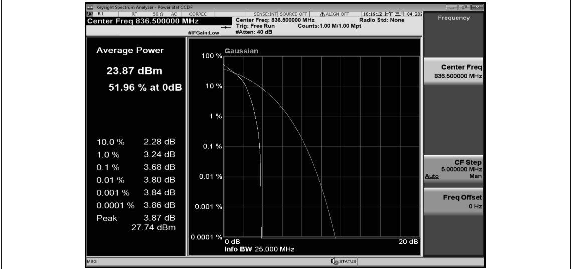
Band26-1.4MHz-QPSK-26915-6RB#0
