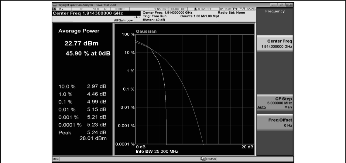
Band25-1.4MHz-16QAM-26683-6RB#0
