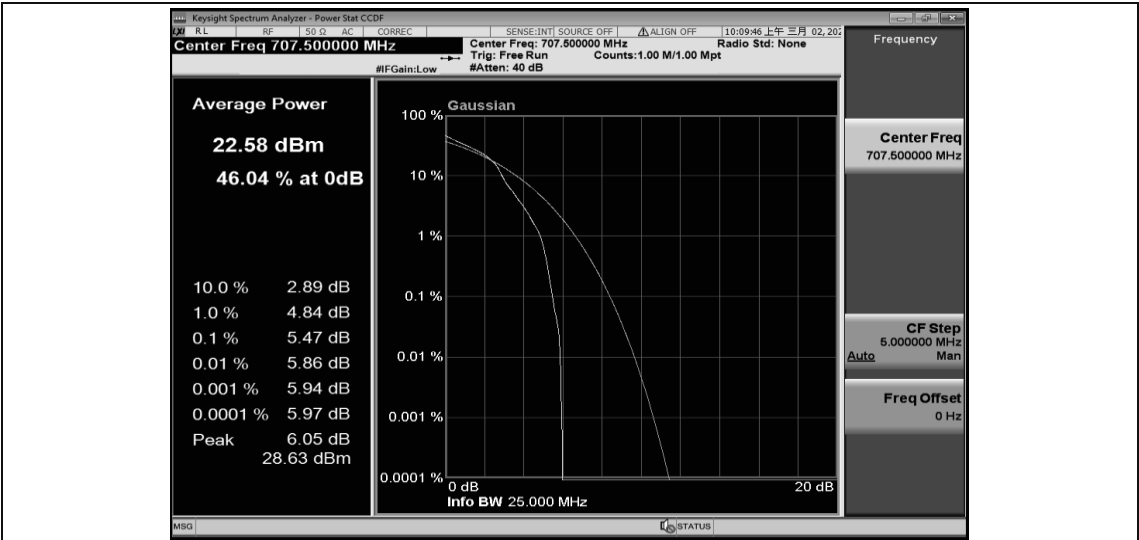
Band12-1.4MHz-16QAM-23095-6RB#0
