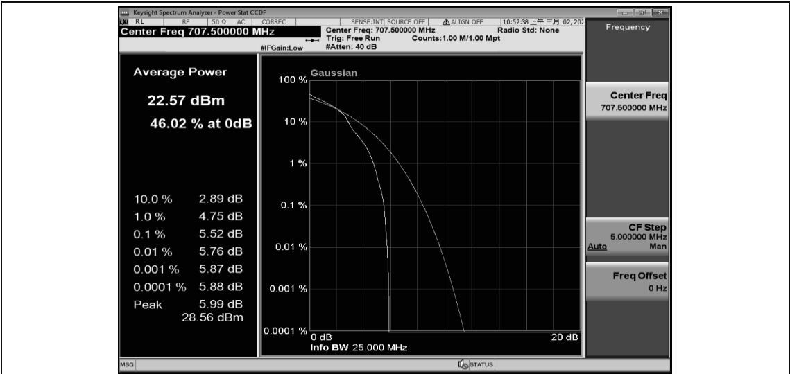
Band12-3MHz-16QAM-23095-15RB#0
