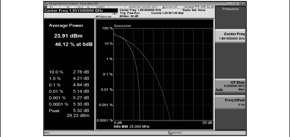
Band25-3MHz-16QAM-26055-15RB#0
