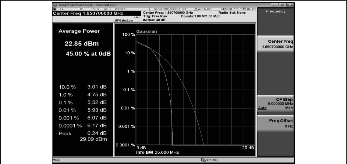
Band25-1.4MHz-16QAM-26365-1RB#0
