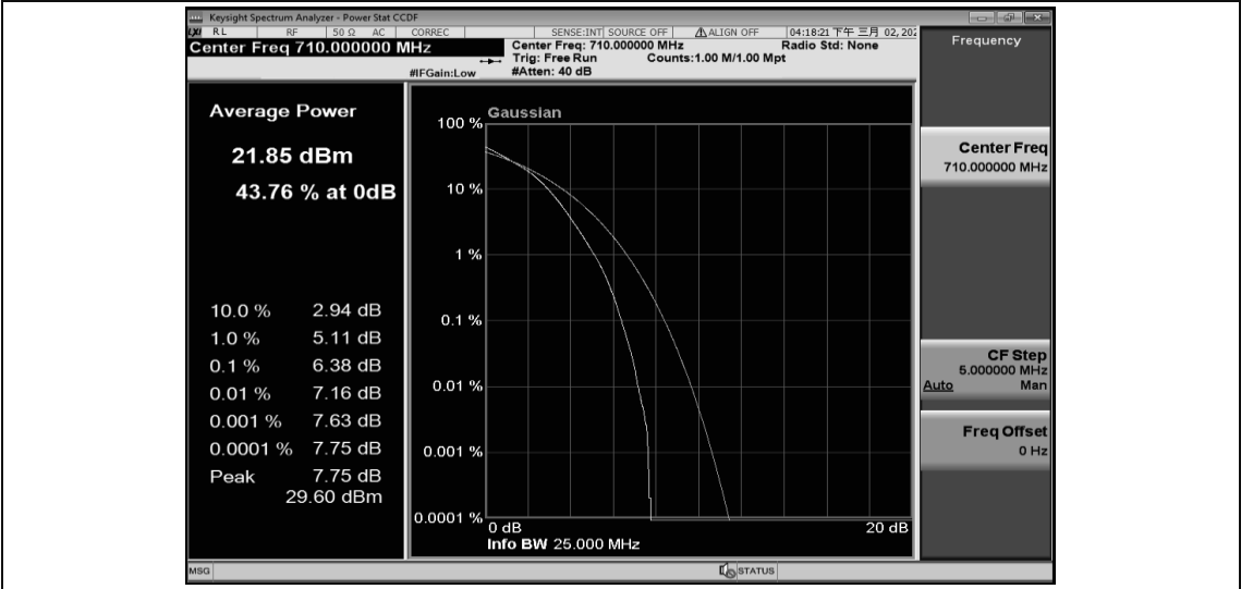
Band17-10MHz-16QAM-23800-1RB#0
