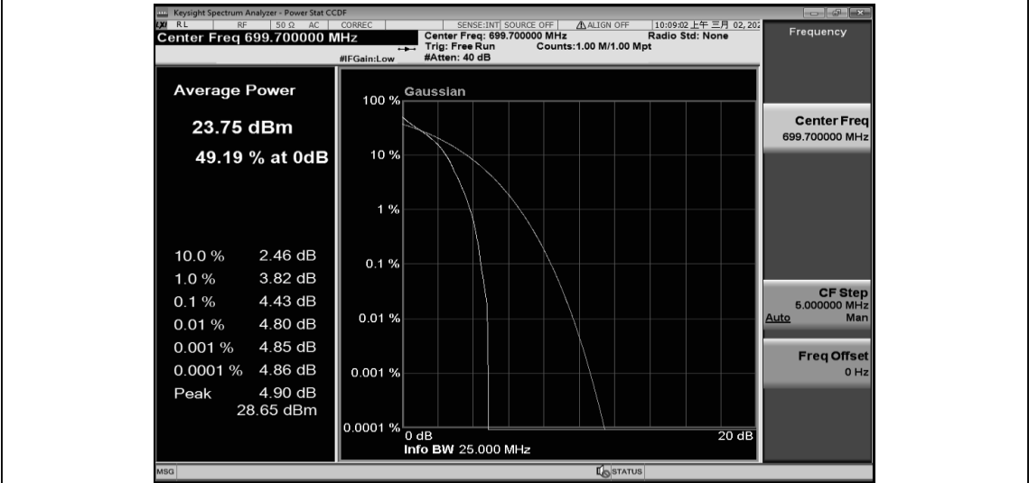
Band12-1.4MHz-QPSK-23017-6RB#0
