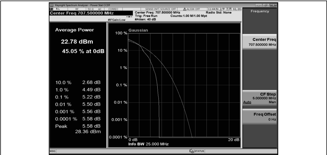
Band12-5MHz-16QAM-23095-25RB#0
