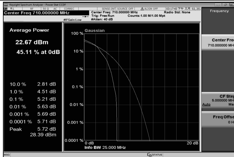
Band17-5MHz-16QAM-23790-25RB#0
