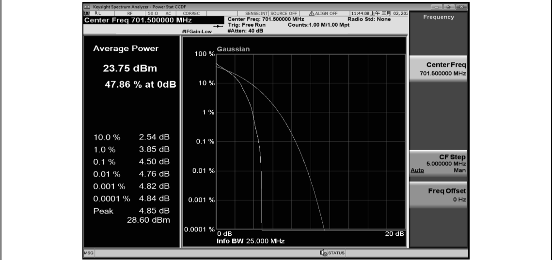
Band12-5MHz-QPSK-23035-25RB#0
