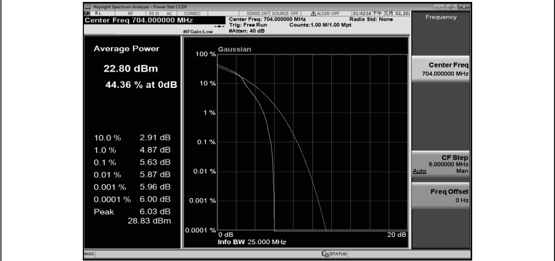
Band12-10MHz-16QAM-23060-50RB#0
