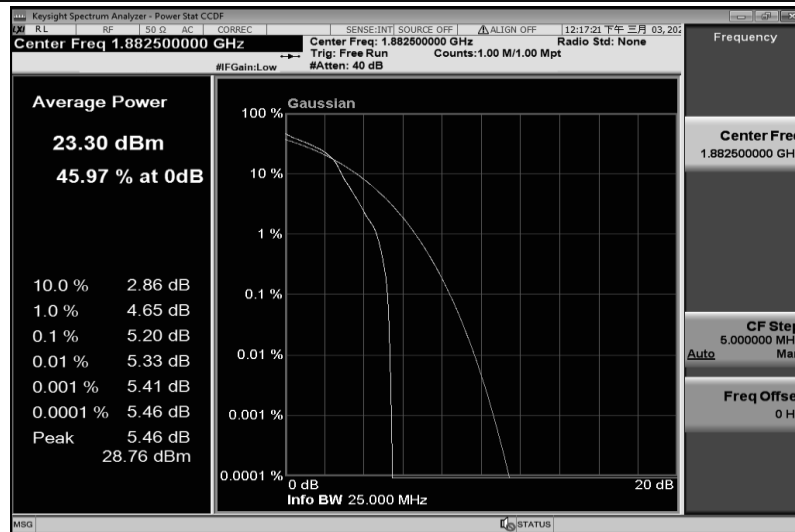
Band25-15MHz-16QAM-26365-75RB#0
