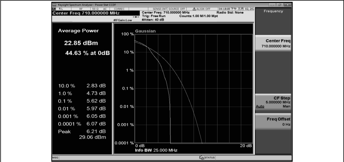
Band17-10MHz-16QAM-23790-50RB#0
