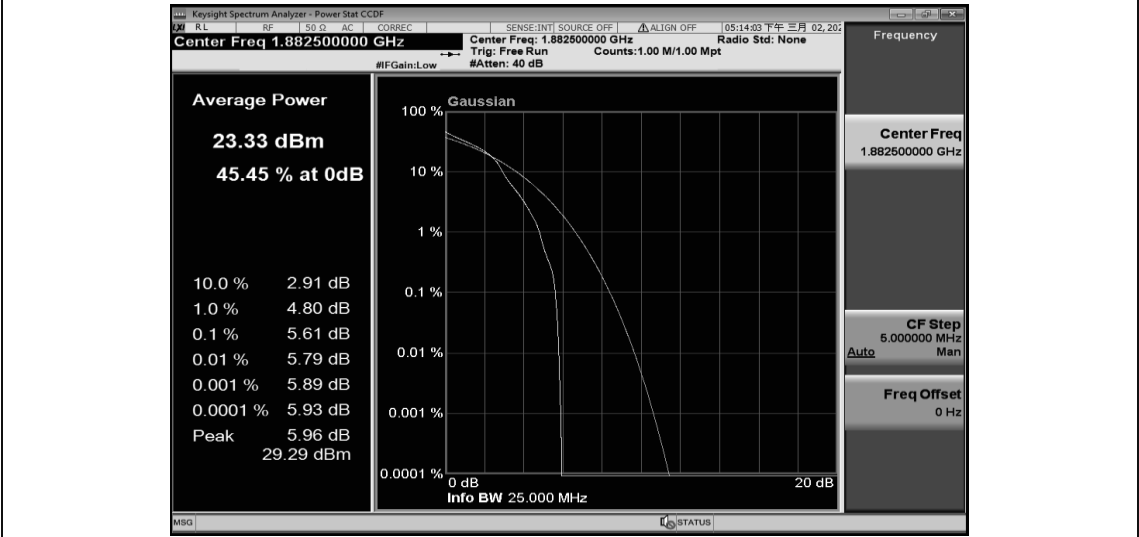
Band25-1.4MHz-16QAM-26365-6RB#0
