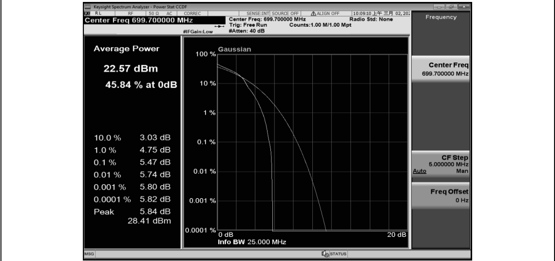
Band12-1.4MHz-16QAM-23017-6RB#0
