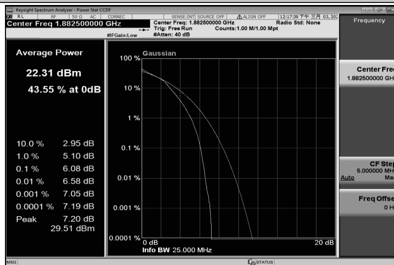
Band25-15MHz-16QAM-26615-1RB#0
