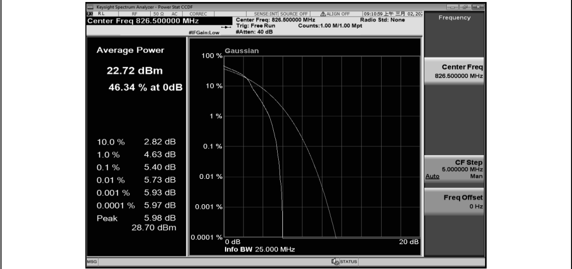
Band5-5MHz-16QAM-20425-25RB#0
