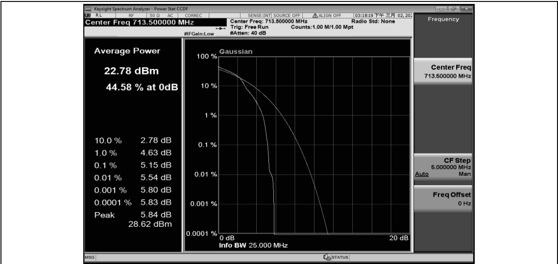
Band17-5MHz-16QAM-23825-25RB#0
