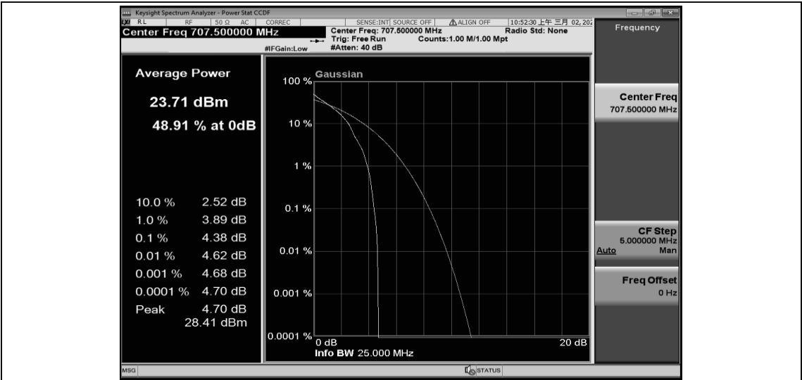
Band12-3MHz-QPSK-23095-15RB#0
