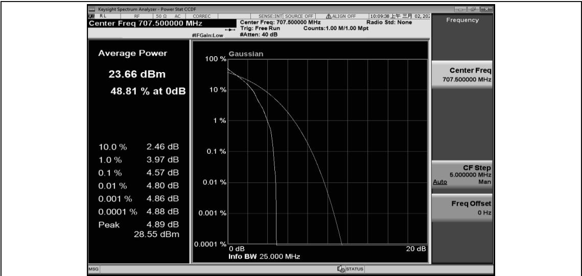
Band12-1.4MHz-QPSK-23095-6RB#0
