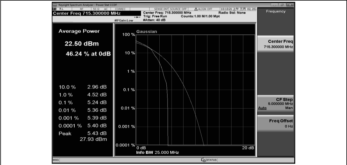
Band12-1.4MHz-16QAM-23173-6RB#0
