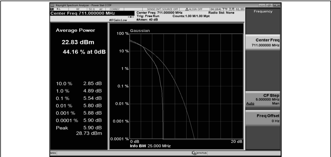
Band17-10MHz-16QAM-23800-50RB#0
