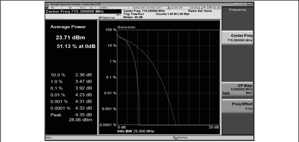
Band12-1.4MHz-QPSK-23173-6RB#0
