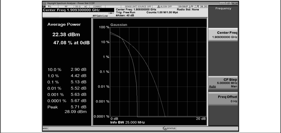
Band2-1.4MHz-16QAM-19193-6RB#0
