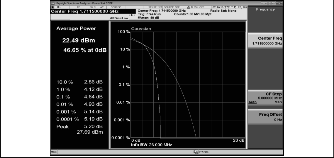
Band4-3MHz-16QAM-20175-1RB#0
