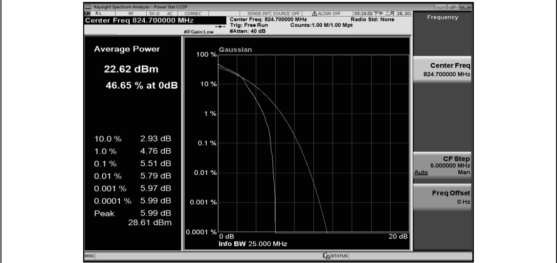
Band5-1.4MHz-16QAM-20407-6RB#0
