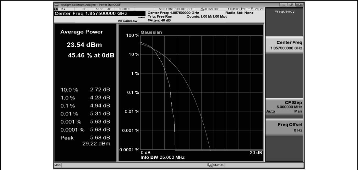
Band2-15MHz-16QAM-18675-75RB#0
