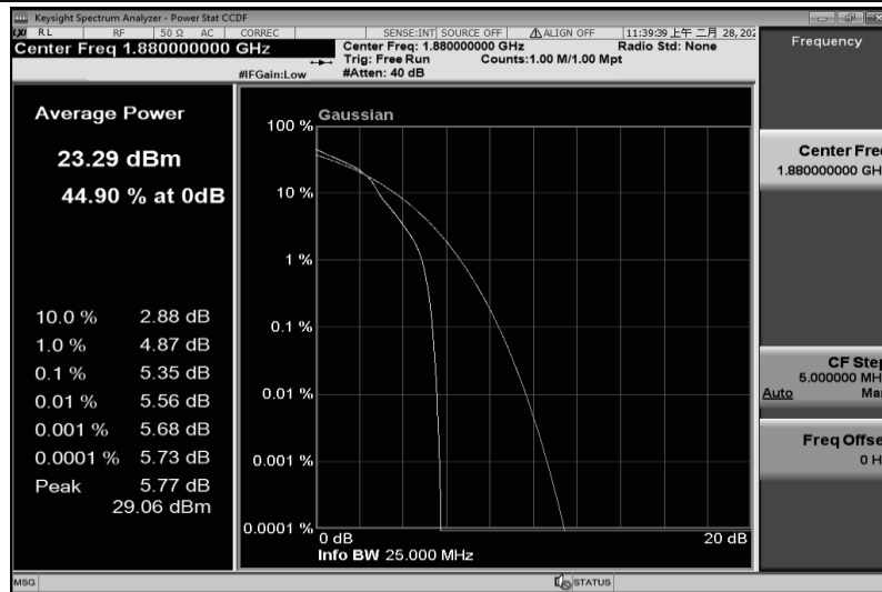
Band2-15MHz-16QAM-18900-75RB#0
