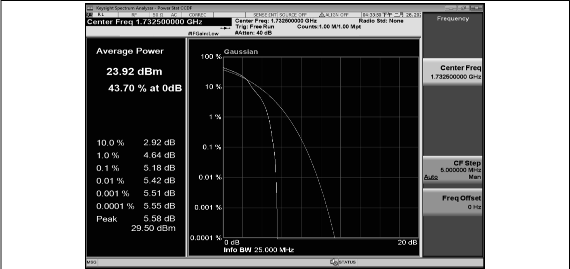
Band4-15MHz-16QAM-20175-75RB#0
