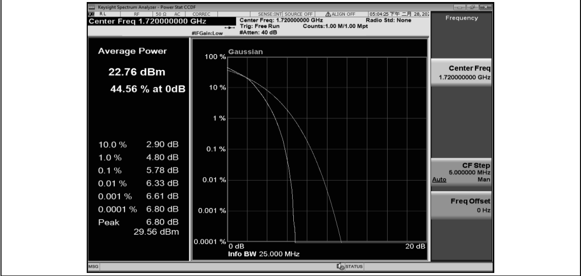
Band4-20MHz-16QAM-20175-1RB#0
