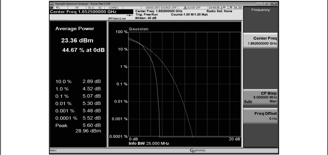
Band2-5MHz-16QAM-18625-25RB#0
