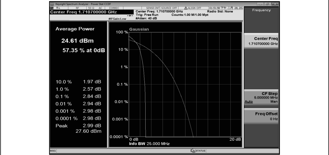
Band4-1.4MHz-QPSK-19957-6RB#0
