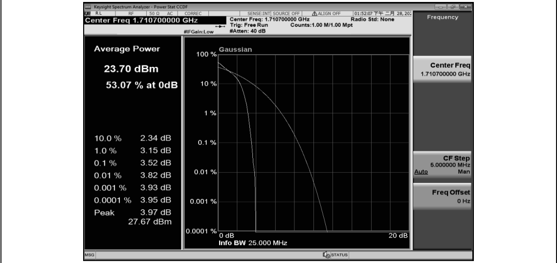
Band4-1.4MHz-QPSK-20175-1RB#0
