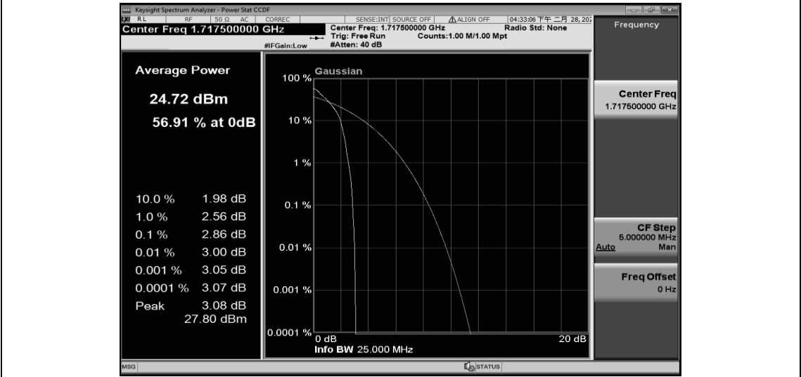
Band4-15MHz-QPSK-20025-75RB#0
