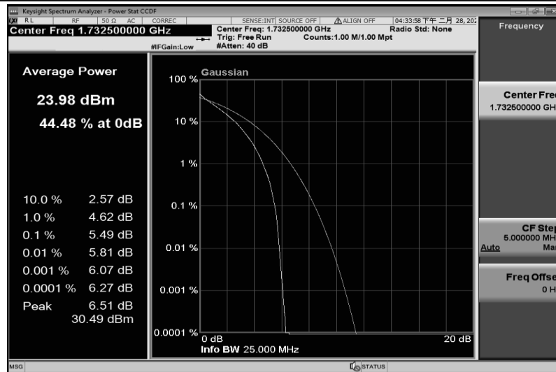
Band4-15MHz-QPSK-20325-1RB#0
