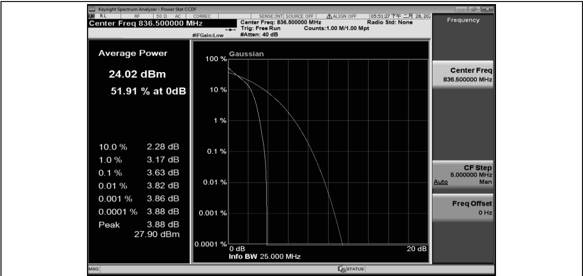
Band5-3MHz-QPSK-20525-15RB#0
