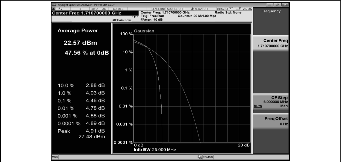
Band4-1.4MHz-16QAM-20175-1RB#0
