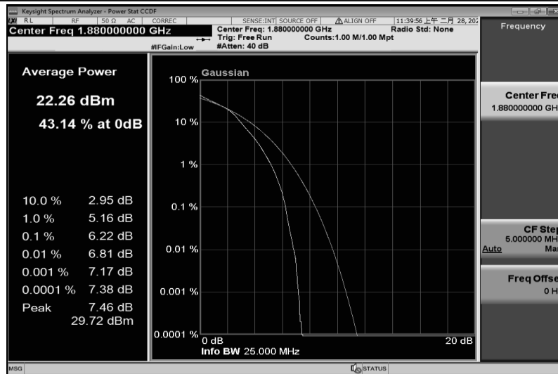
Band2-15MHz-16QAM-19125-1RB#0
