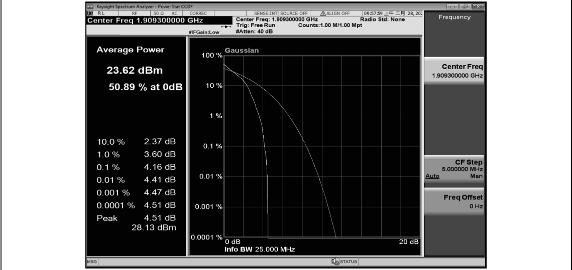
Band2-1.4MHz-QPSK-19193-6RB#0
