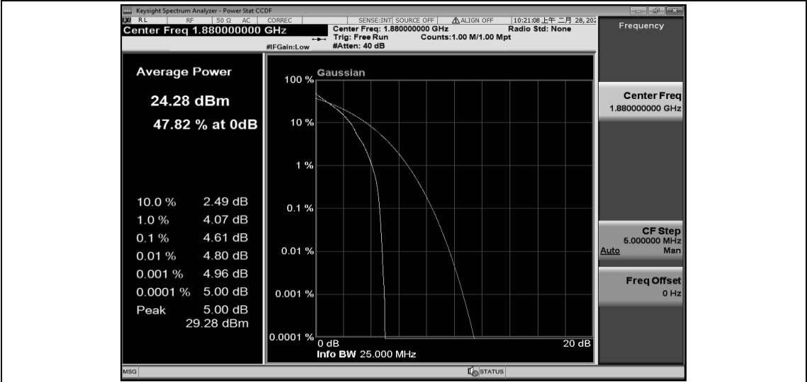
Band2-3MHz-QPSK-18900-15RB#0
