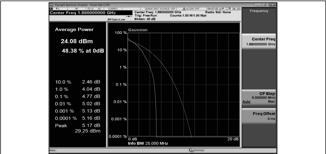
Band2-1.4MHz-QPSK-18900-6RB#0
