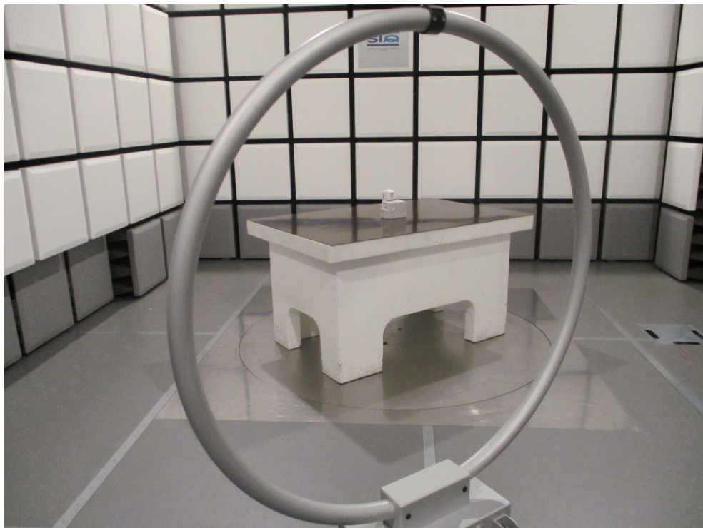
Figure 1: Radiated emission test from 9 kHz to 30 MHz
