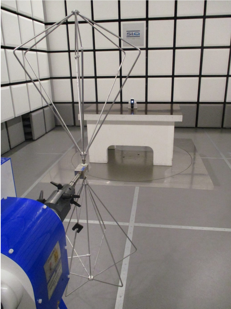
Figure 2: Radiated emission test from 30 MHz to 200 MHz
