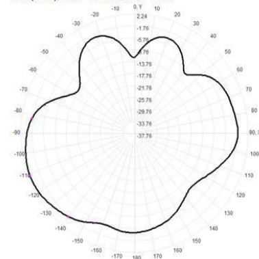
Total(H-XY), Max= 1.61dBi, CirD=14.96
