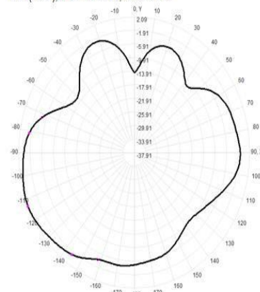
Total(H-XY), Max= 2.05dBi, CirD=16.36
