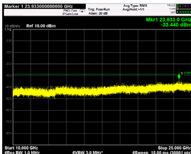
802.11g_CH High(Above 1 GHz)
