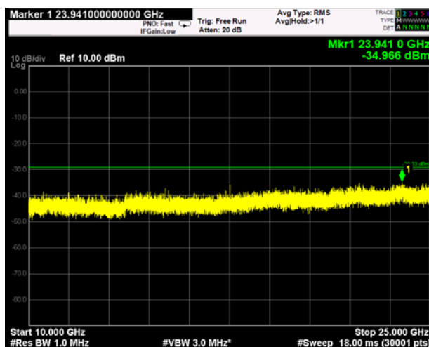
802.11g_CH Middle(Above 1 GHz)
