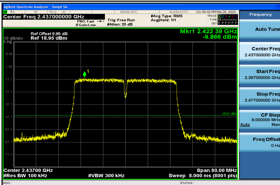
RF Conducted Spurious Emissions_11N40SISO_2437_Ant2
