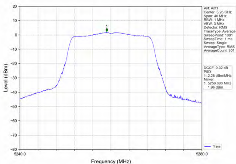
802.11ac(VHT20)_LCH_5260MHz_Ant1_NTNV
