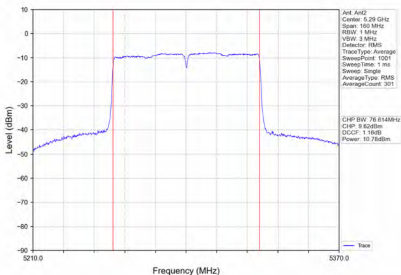
802.11ac(VHT80)_MCH_5290MHz_Ant2_NTNV
