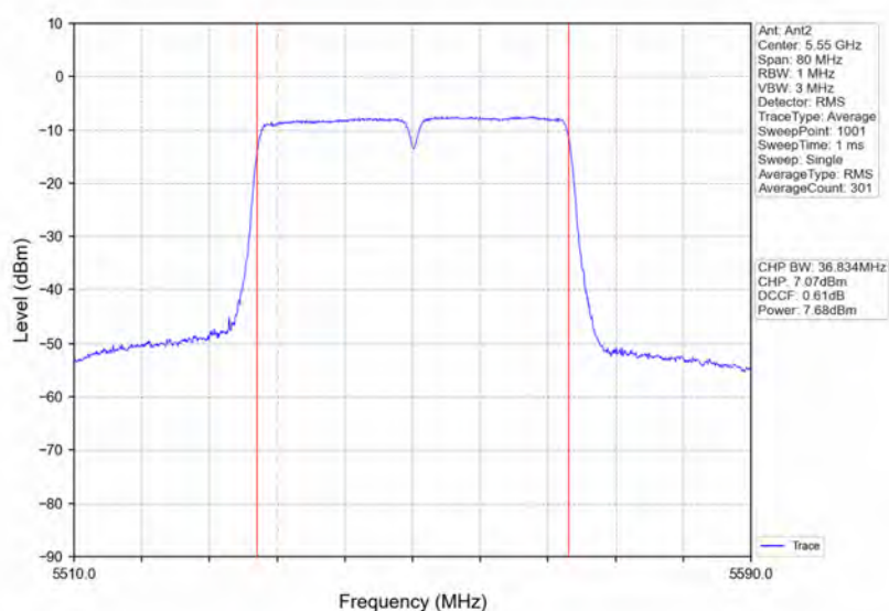
802.11ac(VHT40)_MCH_5550MHz_Ant2_NTNV
