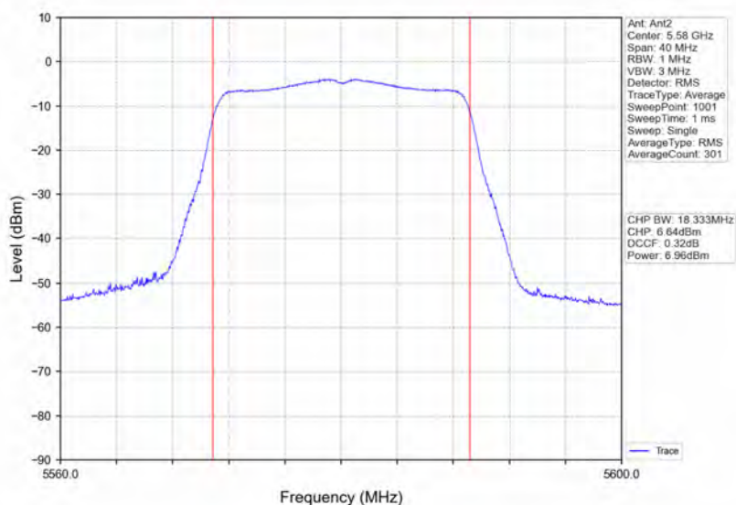
802.11ac(VHT20)_MCH_5580MHz_Ant2_NTNV
