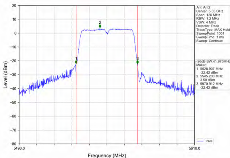
802.11ac(VHT40)_MCH_5550MHz_Ant2_NTNV
