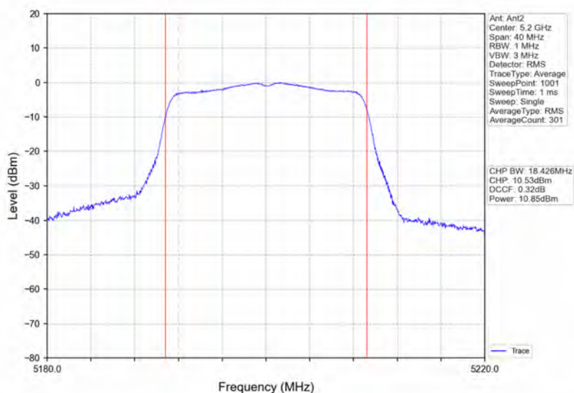
802.11ac(VHT20)_MCH_5200MHz_Ant2_NTNV
