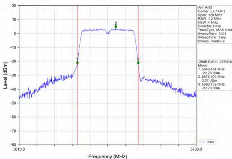
802.11ac(VHT40)_HCH_5670MHz_Ant2_NTNV
