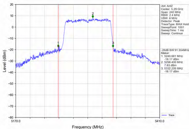
802.11ac(VHT80)_MCH_5290MHz_Ant2_NTNV
