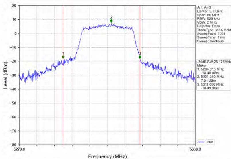
802.11ac(VHT20)_MCH_5300MHz_Ant2_NTNV
