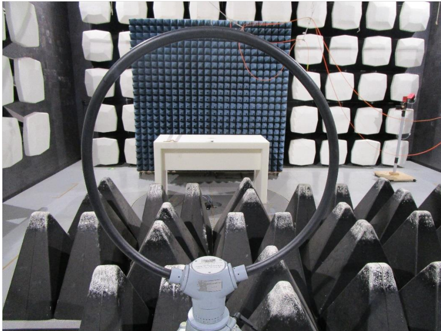
Photograph 5: EUT Setup Electrical Field Measurements in the Semi anechoic chamber
