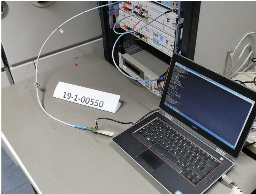
Photograph 1: EUT Test Setup in RadioLab1, conducted measurements
