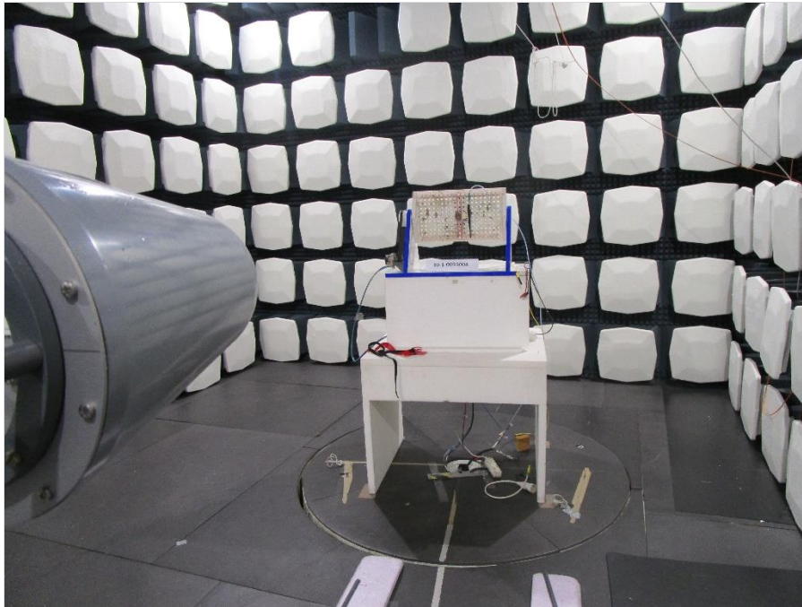
Photograph 7: EUT Setup Electrical Field Measurements in the Fully anechoic chamber
