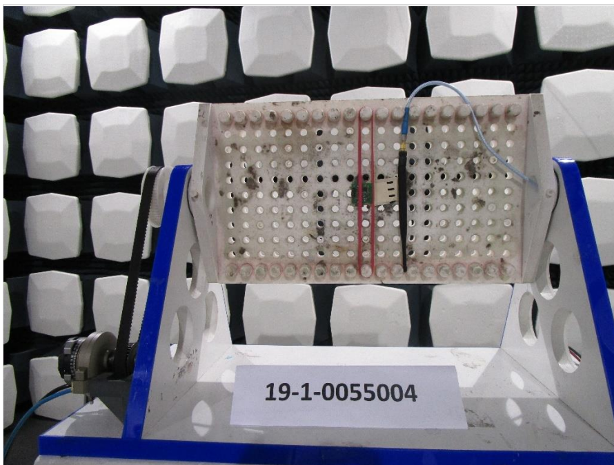
Photograph 8: EUT Setup Electrical Field Measurements in the Fully anechoic chamber
