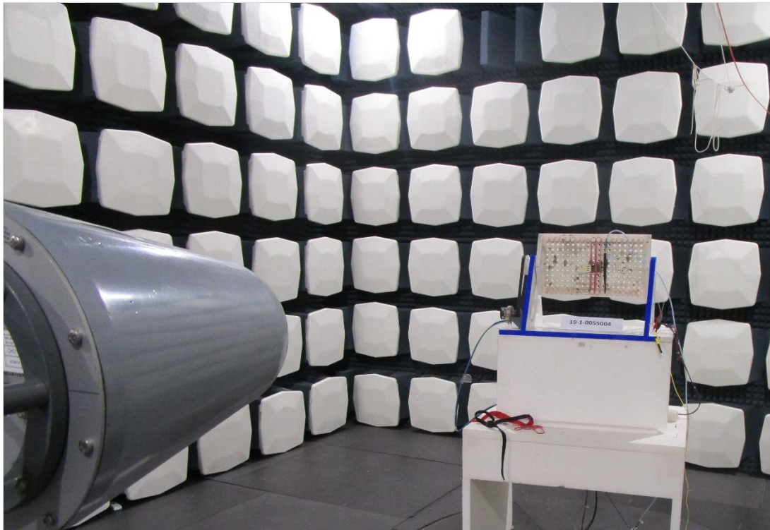
Photograph 1: EUT Test Setup in the fully anechoic chamber, Radiated interference field strength
