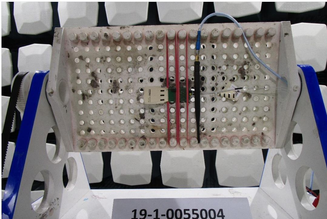
Photograph 2: EUT Test Setup in the fully anechoic chamber, Radiated interference field strength
