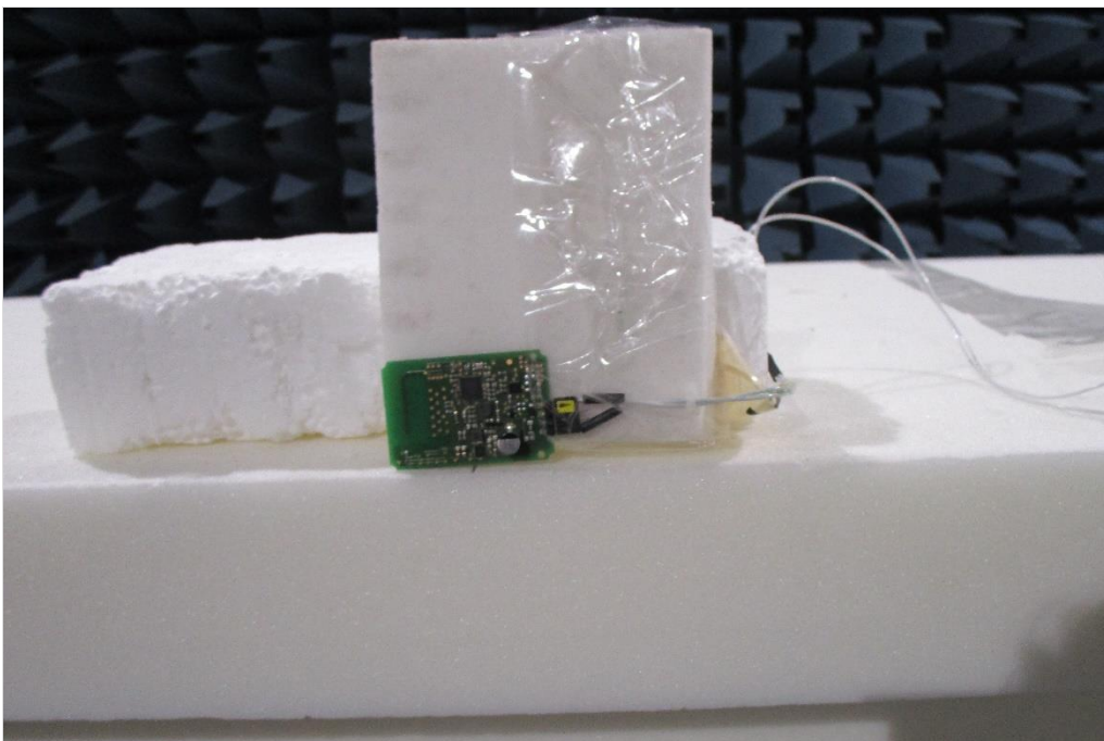
Photograph 6: EUT Setup Magnetic Field Measurements in the Semi anechoic chamber
