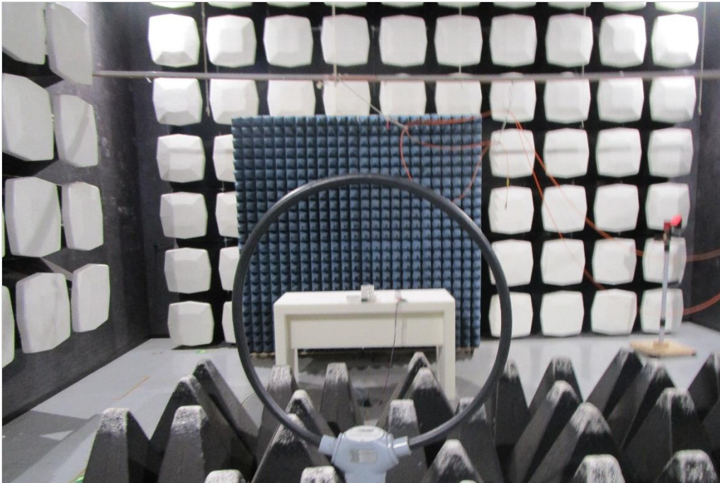
Photograph 5: EUT Setup Magnetic Field Measurements in the Semi anechoic chamber
