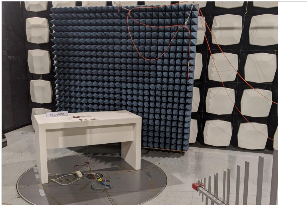
Photograph 3: EUT Test Setup in the semi anechoic chamber, Radiated interference field strength
