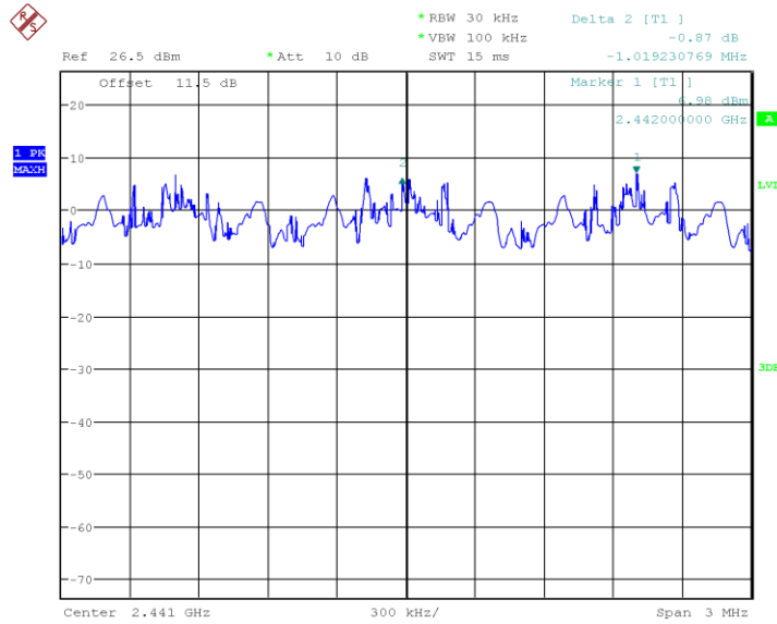
Plot 22. Hopping Separation for 2DH5
