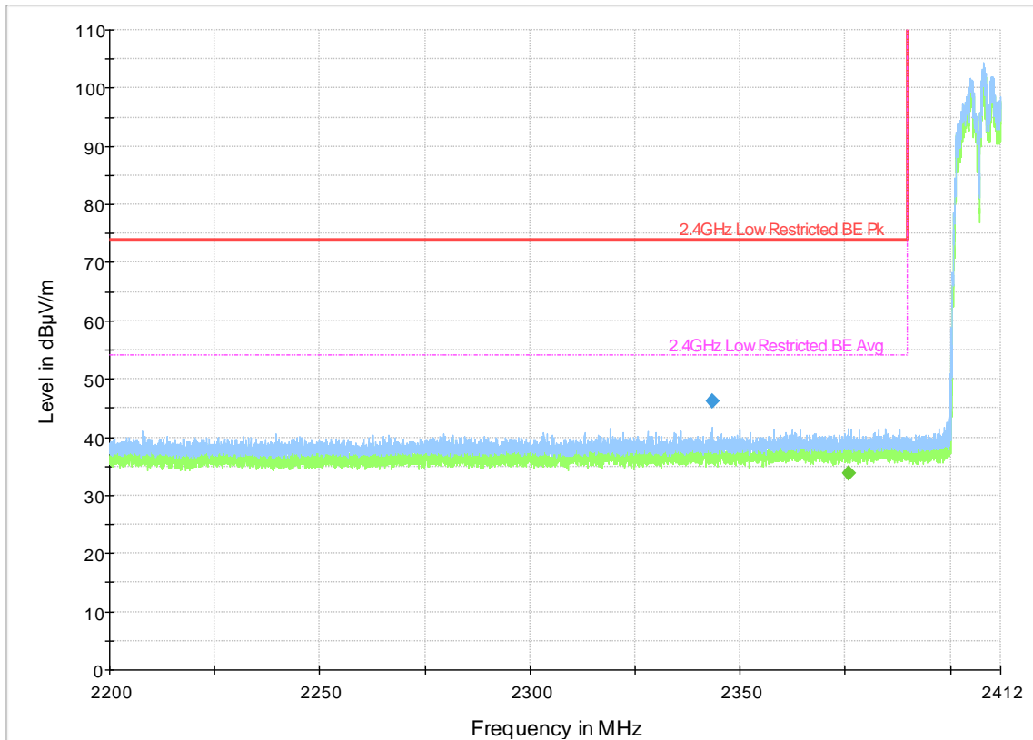
Plot 43. Lower Restricted Band Edge, 2402MHz, 3DH5, Hopping
