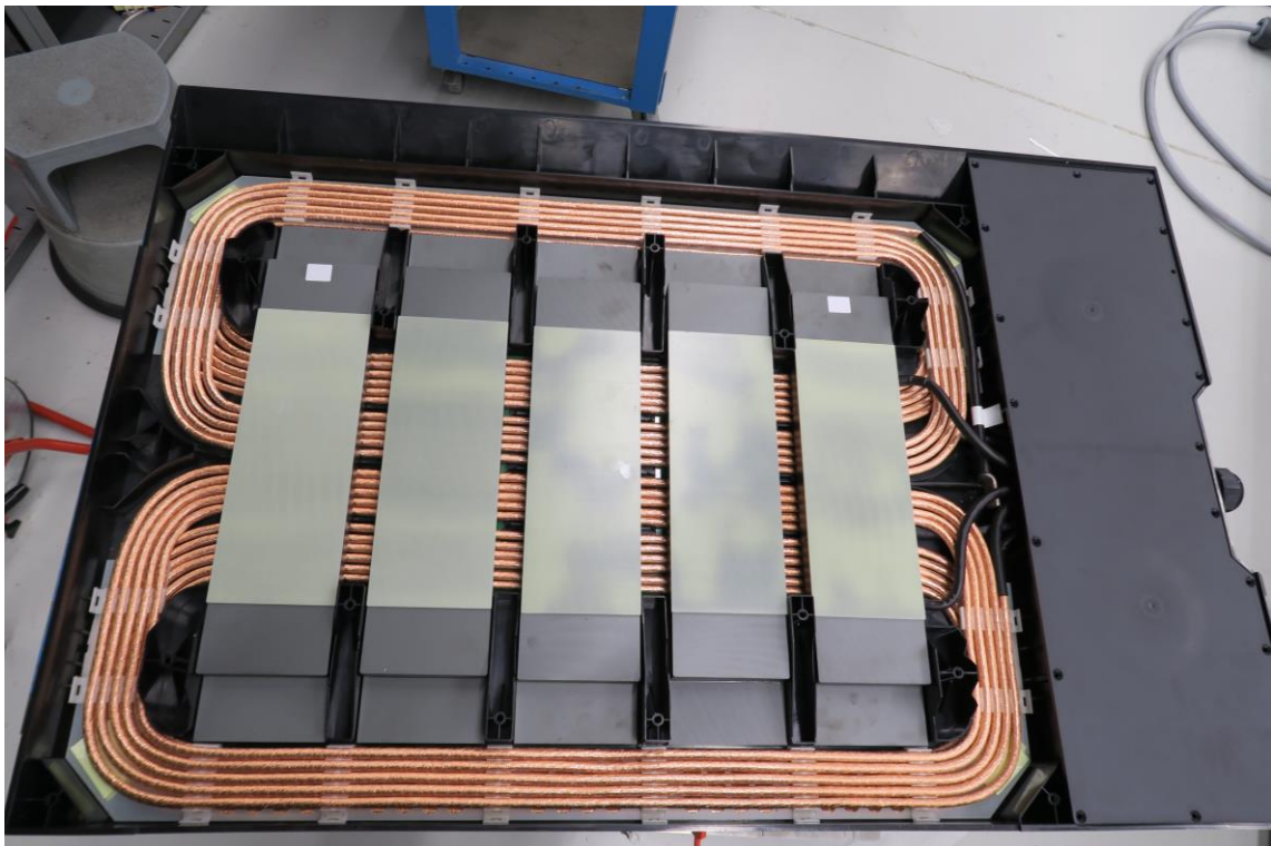
Figure 4: Primary Pad
