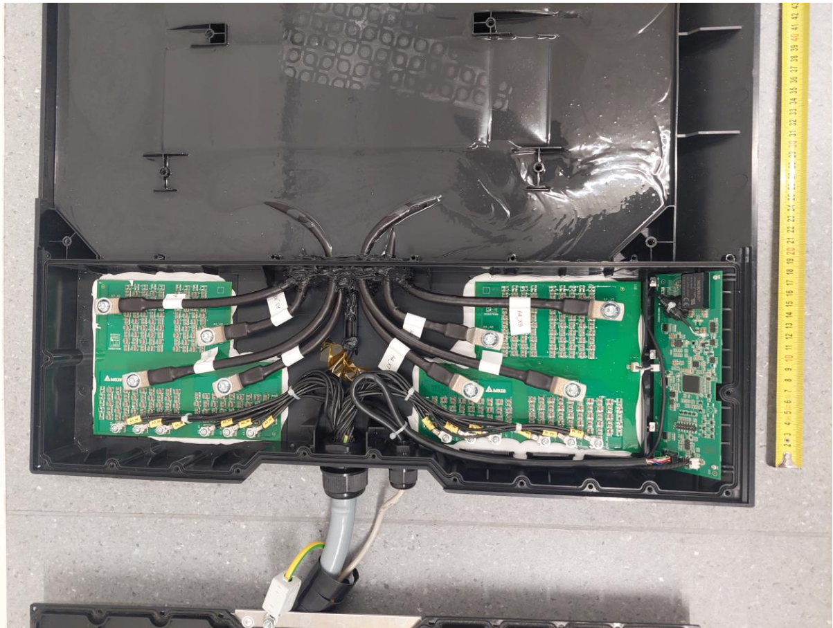
Figure 3: Primary Pad
