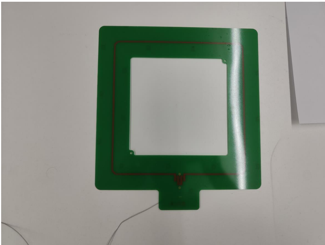
Figure 6: Antenna for primary pad
