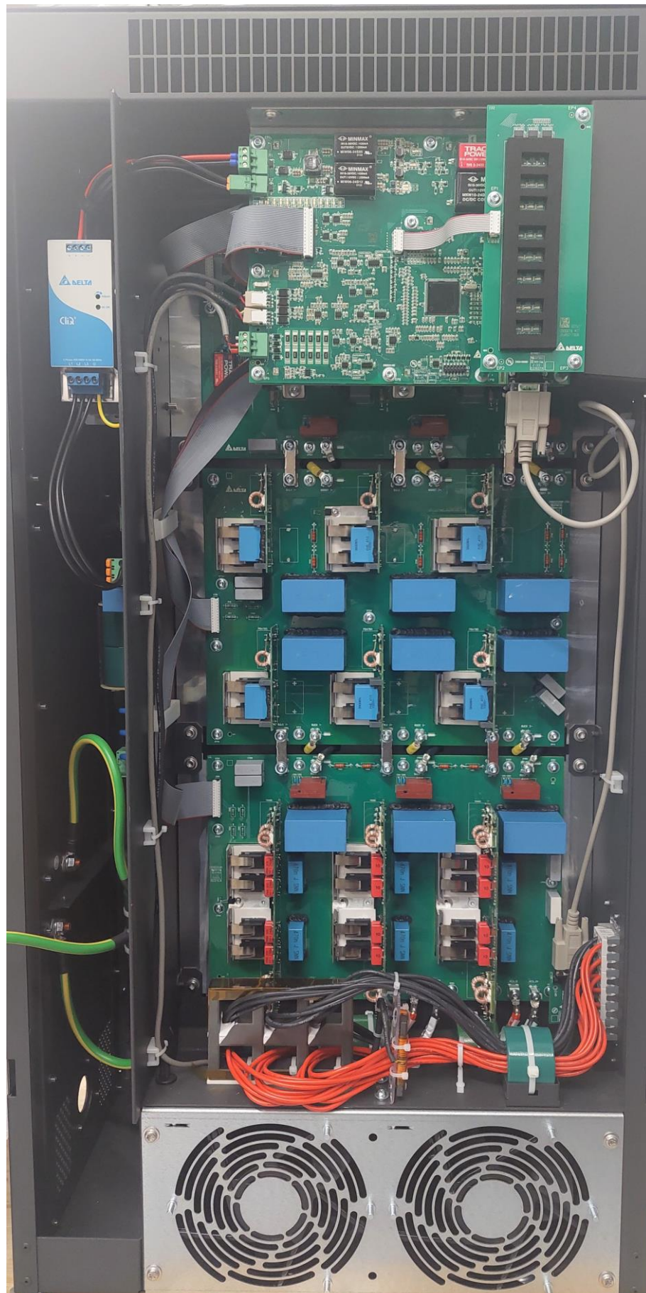
Figure 1: Primary Box
