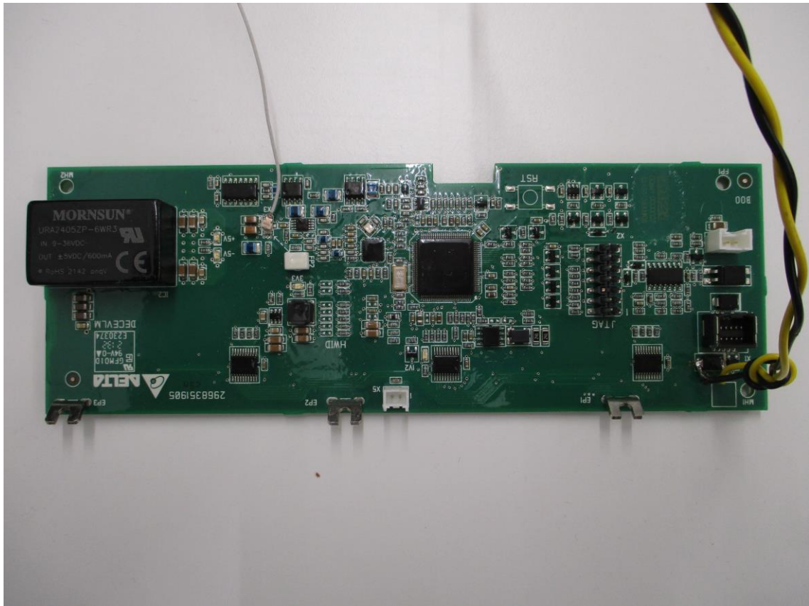
Figure 7: PCB with radio module
