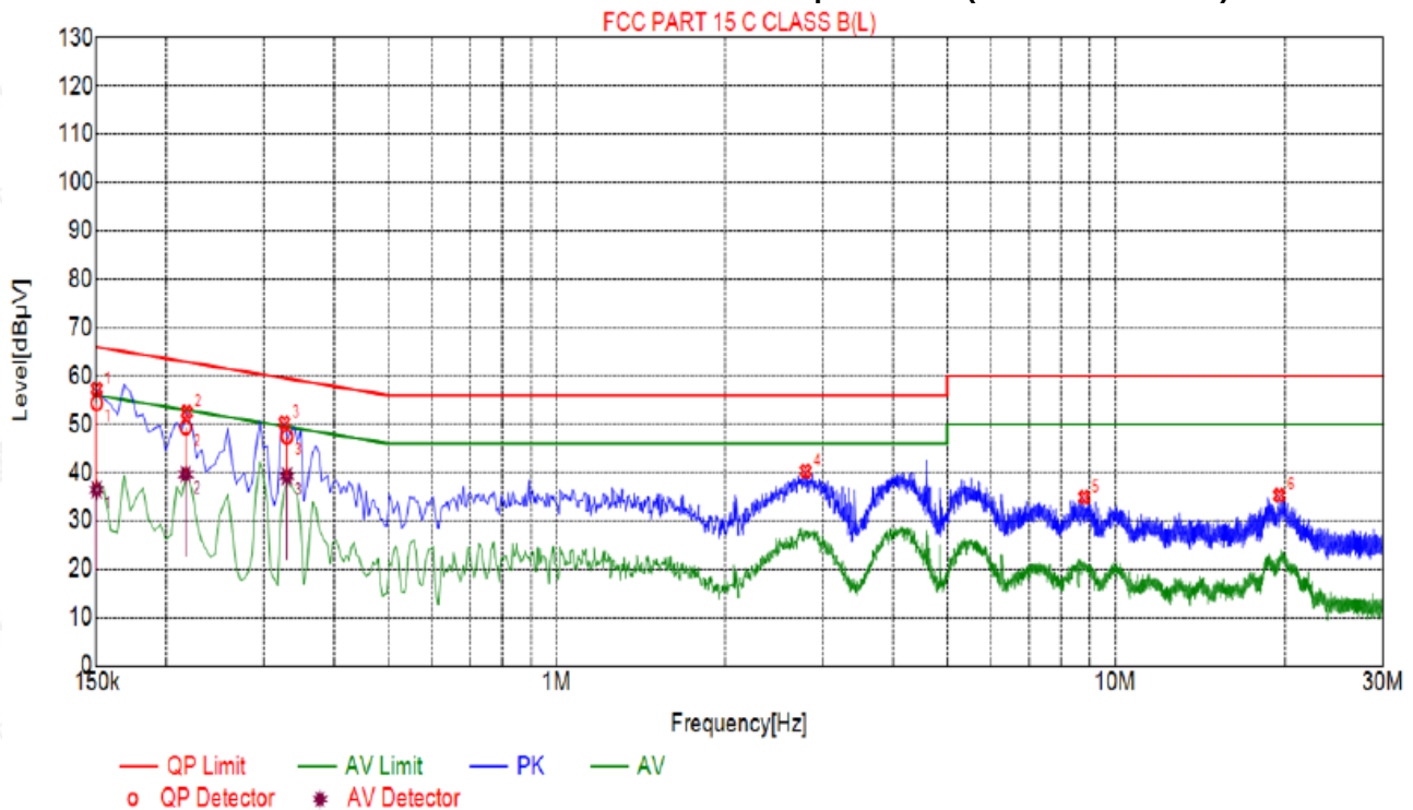
Conducted Emission on Line Terminal of the power line (150 kHz to 30MHz)
