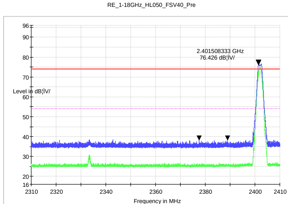
Figure 24: Radiated Band-Edge, TM1, V
