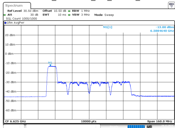
802.11ax80_6625MHz_RU_106/53_Chain 2
