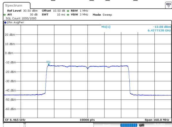
802.11ax80_6465MHz_RU_996/67_Chain 1
