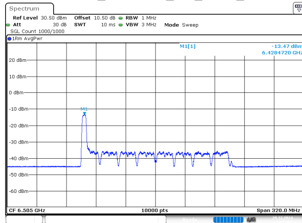
802.11ax160_6505MHz_RU_52/37_Chain 2
