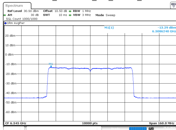
802.11ax80_6545MHz_RU_996/67_Chain 2
