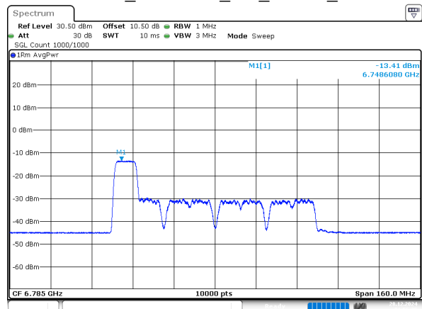
802.11ax80_6785MHz_RU_106/53_Chain 2
