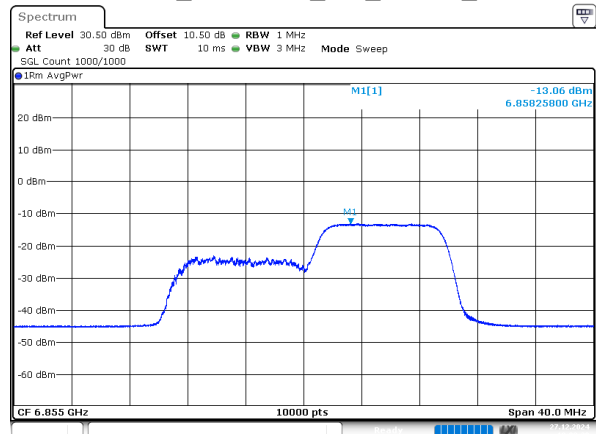
802.11ax20_6855MHz_RU_106/54_Chain 1
