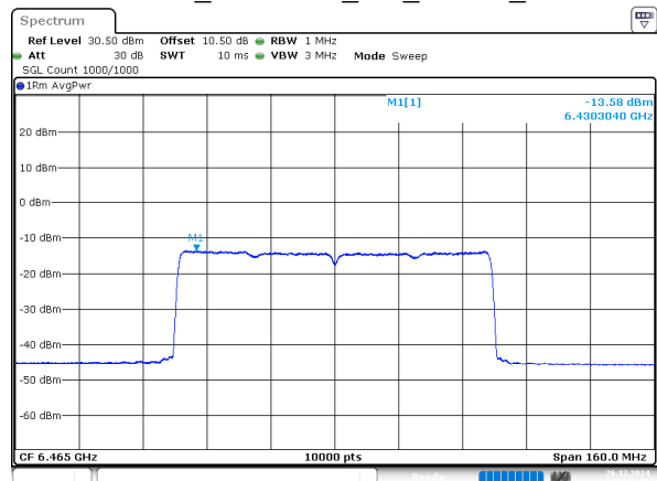
802.11ax80_6465MHz_RU_996/67_Chain 3
