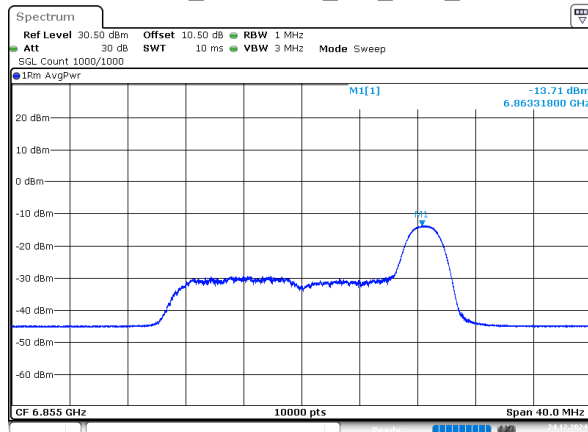
802.11ax20_6855MHz_RU_26/8_Chain 0
