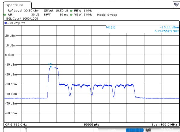
802.11ax80_6785MHz_RU_106/53_Chain 1
