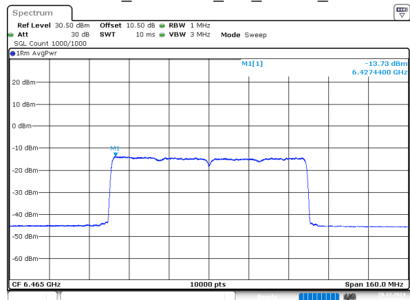
802.11ax80_6465MHz_RU_996/67_Chain 2
