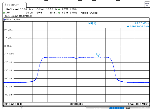
802.11ax20_6695MHz_RU_242/61_Chain 0
