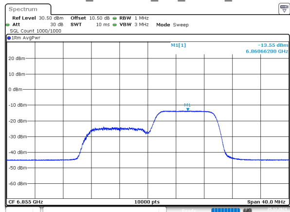
802.11ax20_6855MHz_RU_106/54_Chain 3
