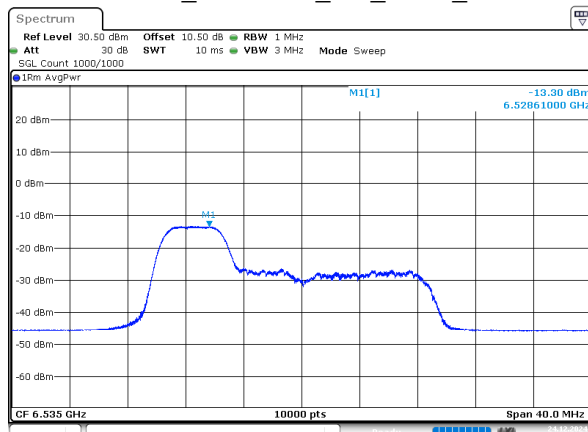
802.11ax20_6535MHz_RU_52/37_Chain 0
