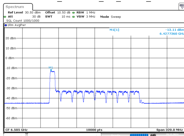
802.11ax160_6505MHz_RU_106/53_Chain 2
