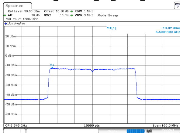
802.11ax80_6545MHz_RU_996/67_Chain 1
