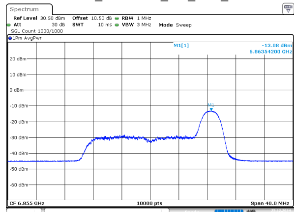
802.11ax20_6855MHz_RU_26/8_Chain 3
