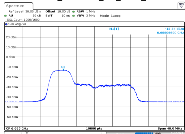
802.11ax20_6695MHz_RU_52/37_Chain 0
