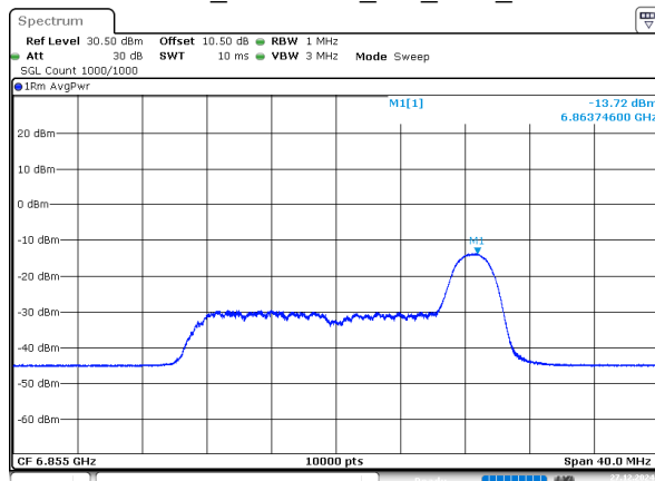
802.11ax20_6855MHz_RU_26/8_Chain 2
