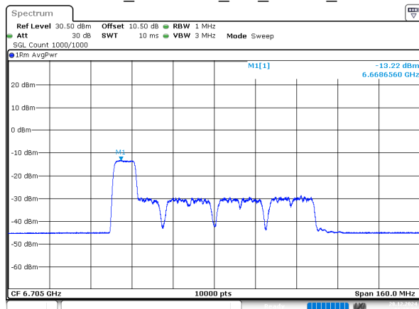
802.11ax80_6705MHz_RU_106/53_Chain 2
