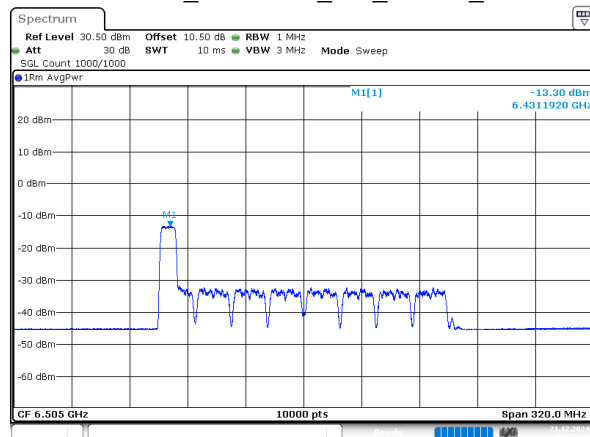
802.11ax160_6505MHz_RU_106/53_Chain 0
