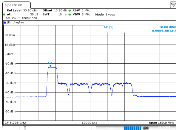
802.11ax80_6705MHz_RU_106/53_Chain 1
