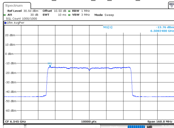
802.11ax80_6545MHz_RU_996/67_Chain 3
