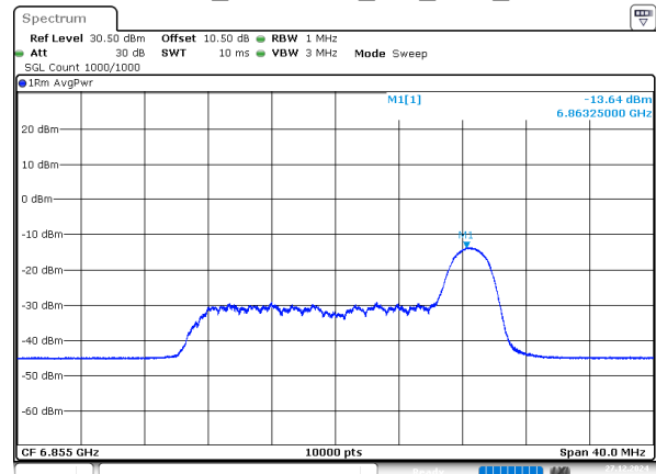
802.11ax20_6855MHz_RU_26/8_Chain 1
