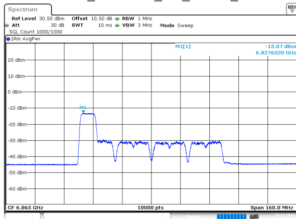
802.11ax80_6865MHz_RU_106/53_Chain 2
