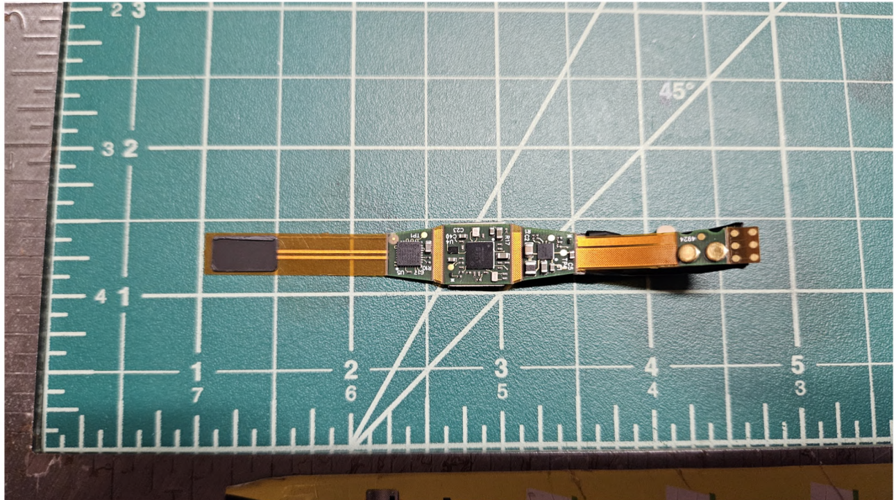
2 Figure 2 - TR3 PCBA Bottom Side
