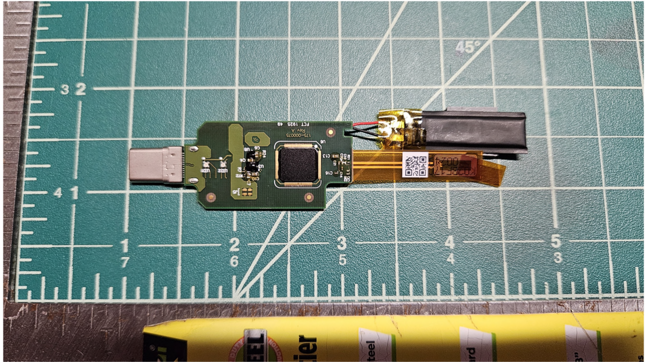
5 Figure 5 - TBK PCBA Top Side
