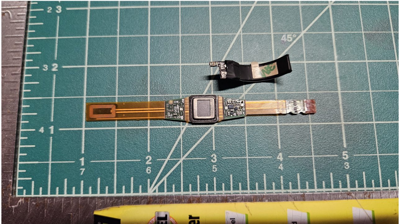
4 Figure 4 - TR3 PCBA Top Side With Battery Removed
