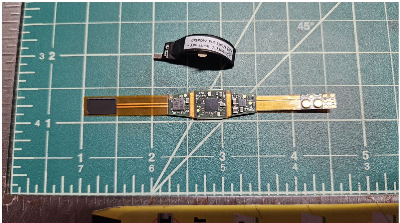
3 Figure 3 - TR3 PCBA Bottom Side With Battery Removed
