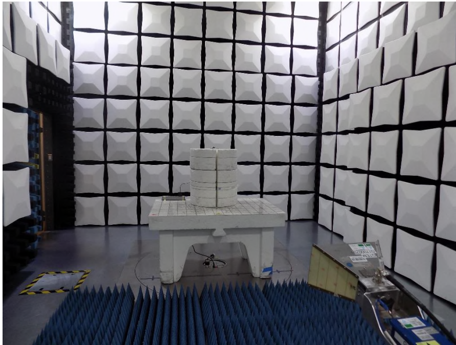
Figure 7 – Test Set Up Photo 1-18 GHz (Bandedge)
