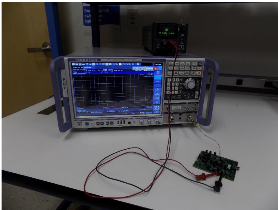
Figure 1 – Conducted Test Set Up (Dev Board)
