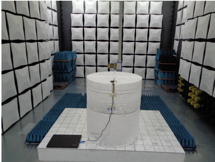
Figure 15– Test Set Up Photo 1-18 GHz
