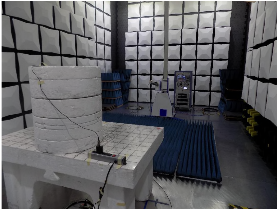
Figure 9– Test Set Up Photo 18-26.5 GHz
