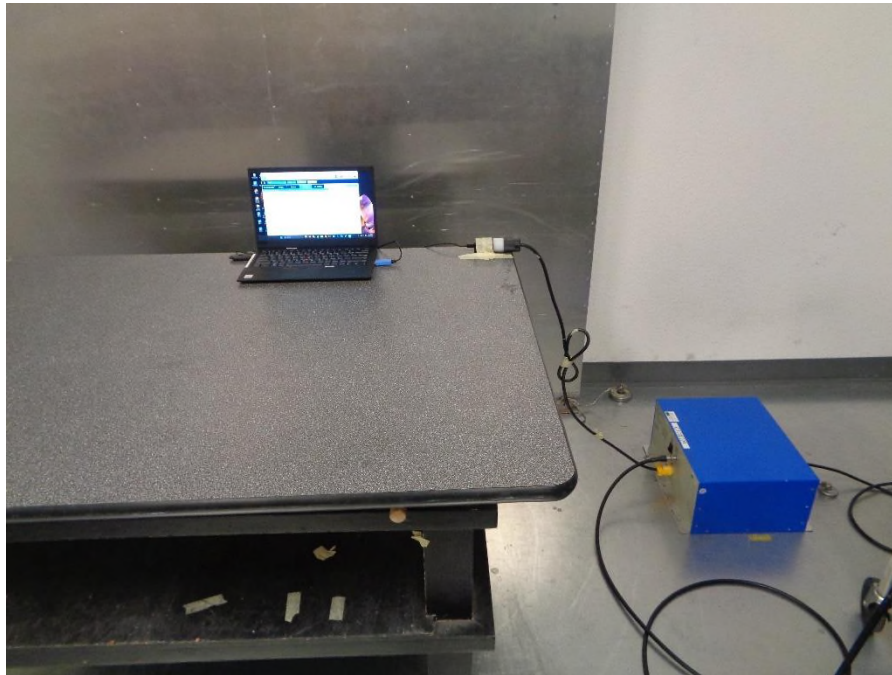
Figure 19— Test Set Up Photo Conducted Emissions
