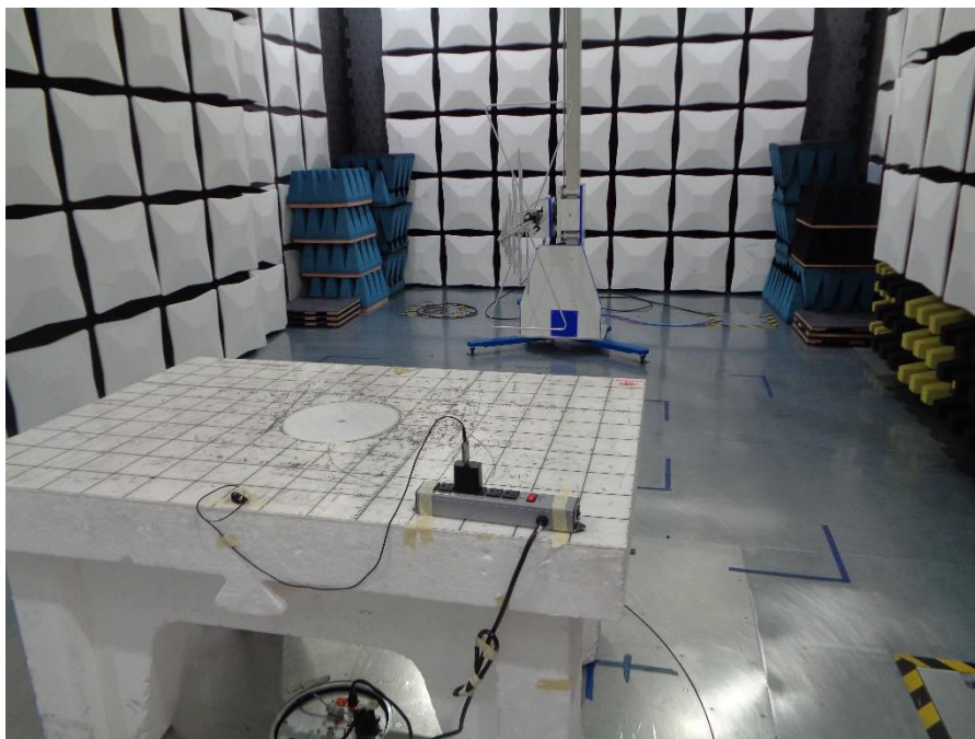
Figure 2– Test Set Up Photo 30-1000 MHz
