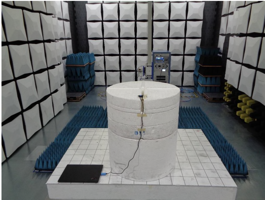
Figure 17– Test Set Up Photo 18-40 GHz
