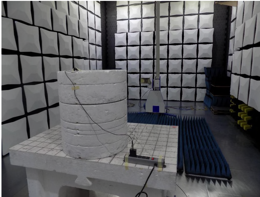
Figure 5 – Test Set Up Photo 1-18 GHz
