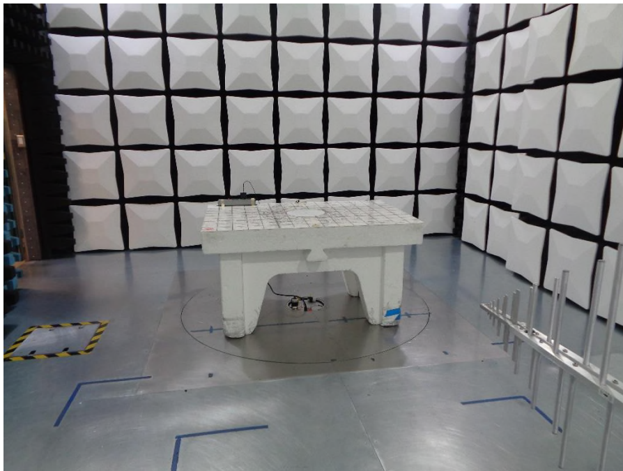
Figure 4 – Test Set Up Photo 30-1000 MHz
