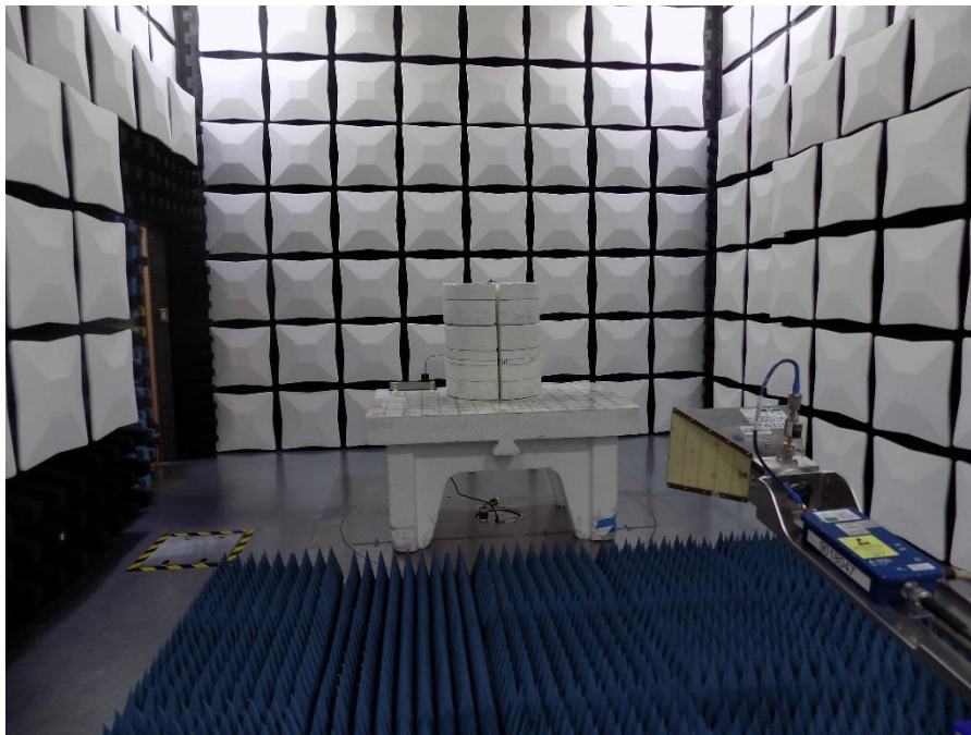
Figure 8– Test Set Up Photo 1-18 GHz
