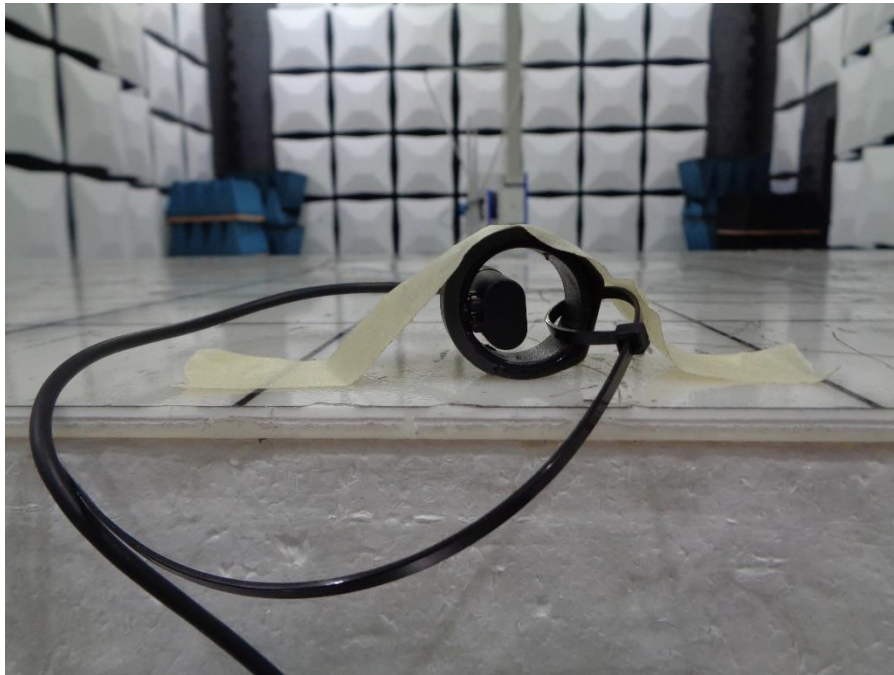
Figure 3– Test Set Up Photo 30-1000 MHz
