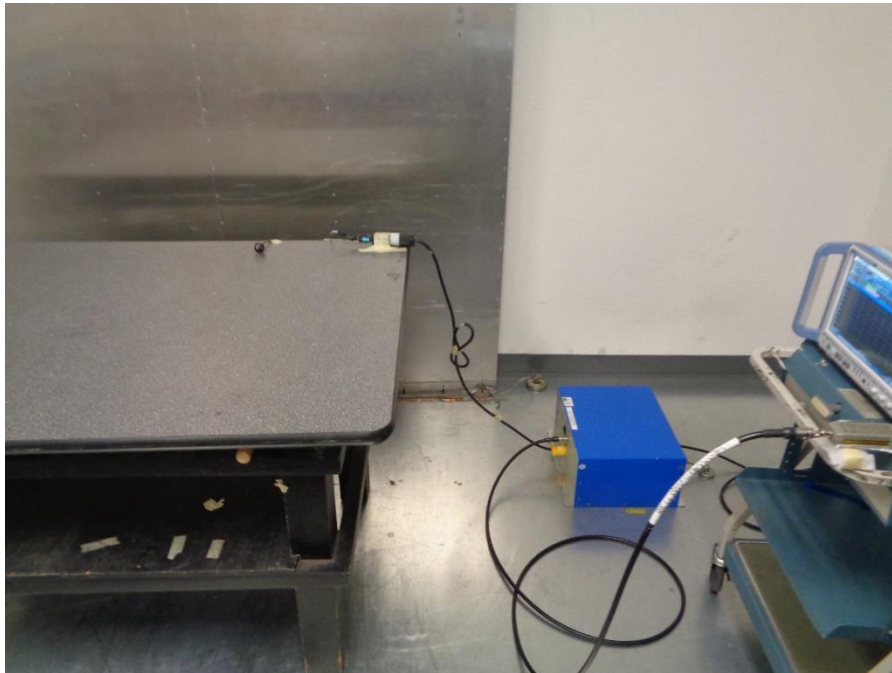
Figure 11– Test Set Up Photo Conducted Emissions
