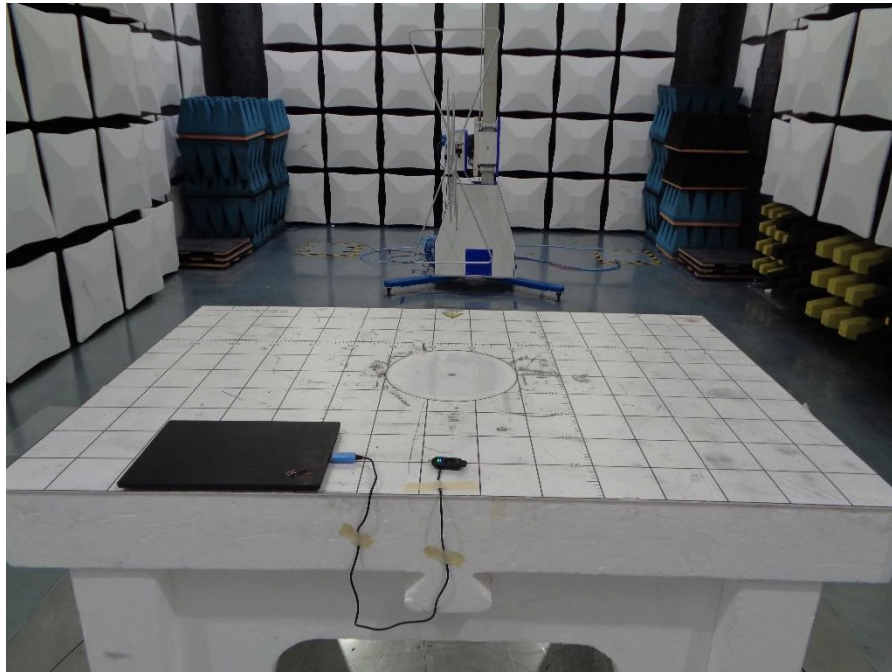
Figure 13– Test Set Up Photo 30-1000 MHz
