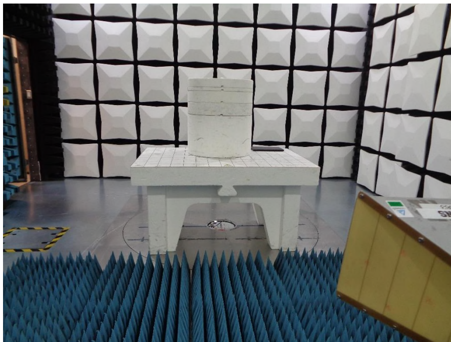
Figure 16– Test Set Up Photo 1-18 GHz
