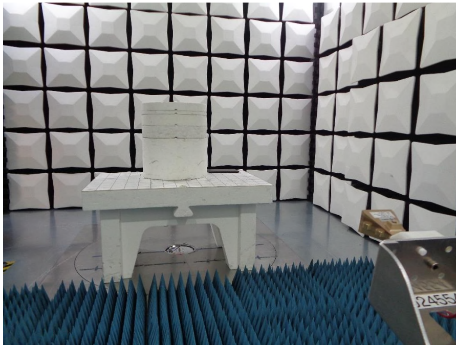
Figure 18– Test Set Up Photo 18-40 GHz
