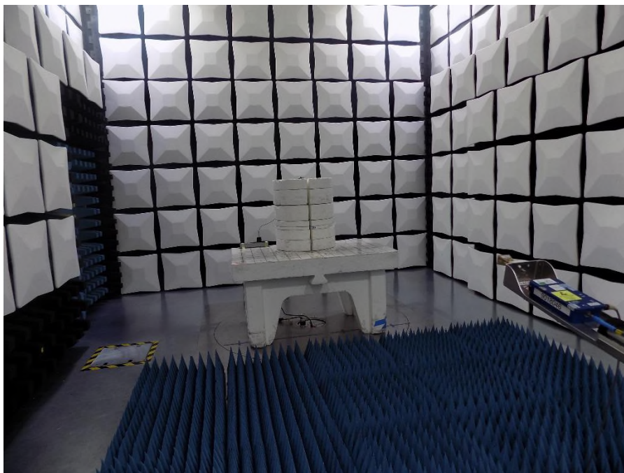
Figure 10– Test Set Up Photo 18-26.5 GHz
