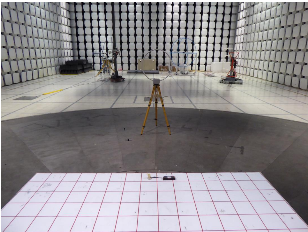
Figure 9 – 9k – 30MHz 3 meter Radiated Setup
