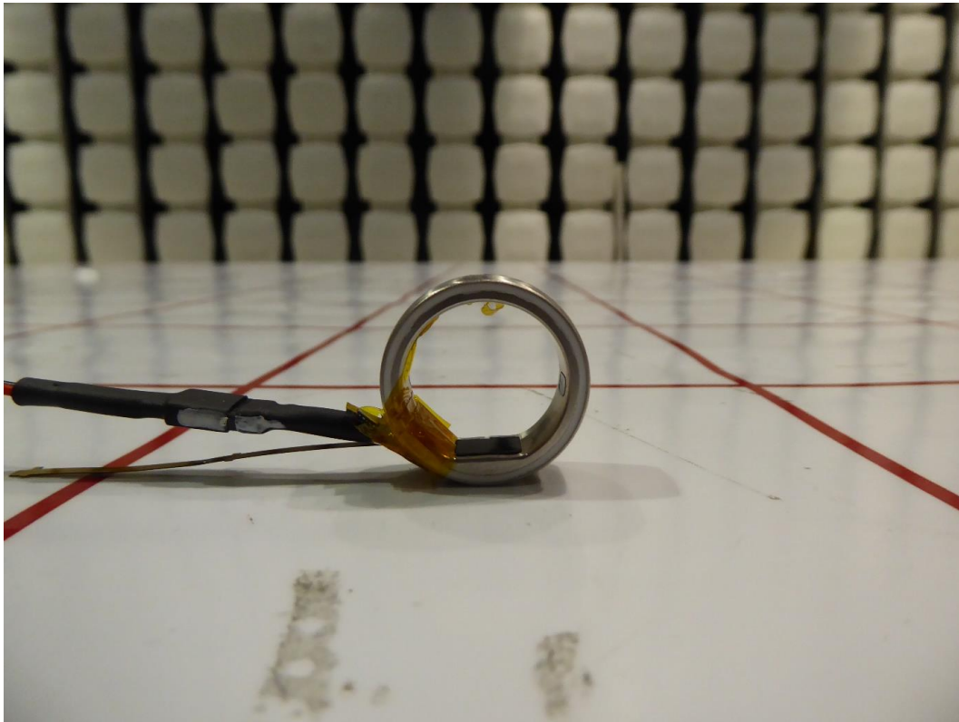
Figure 6 – External Photo of EUT (Radiated Sample 0001, X-axis)
