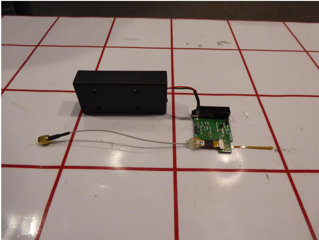
Figure 4 – Internal Photo of EUT (Conducted Sample 0002, Front)
