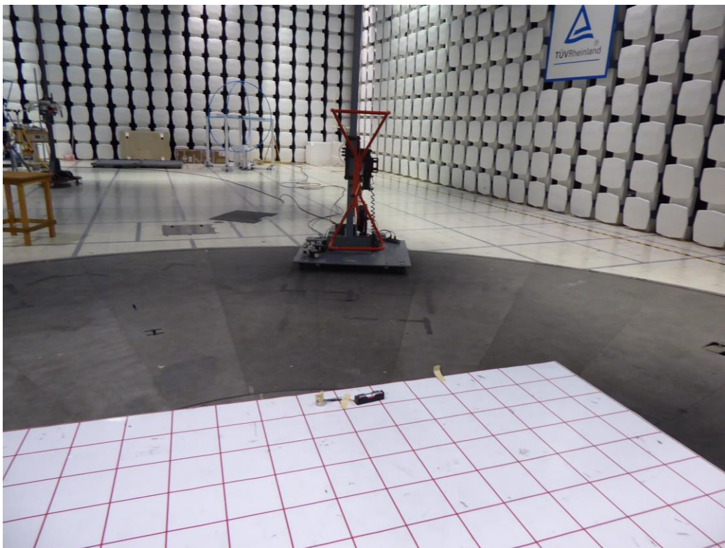
Figure 11 – 30 – 1000 MHz 3 meter Radiated Setup
