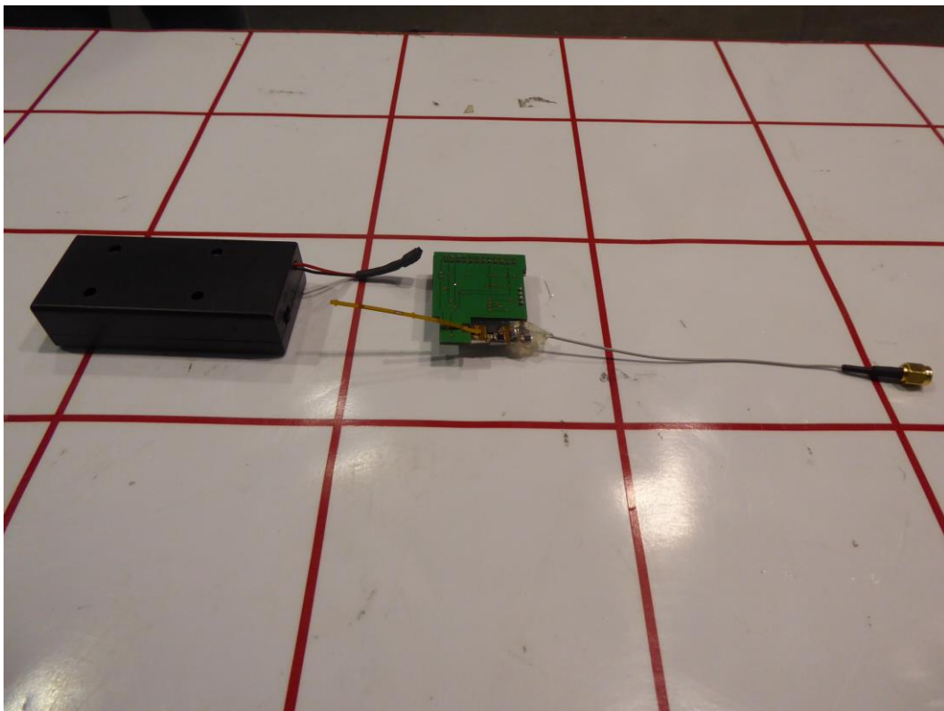
Figure 5 – Internal Photo of EUT (Conducted Sample 0002, Back)
