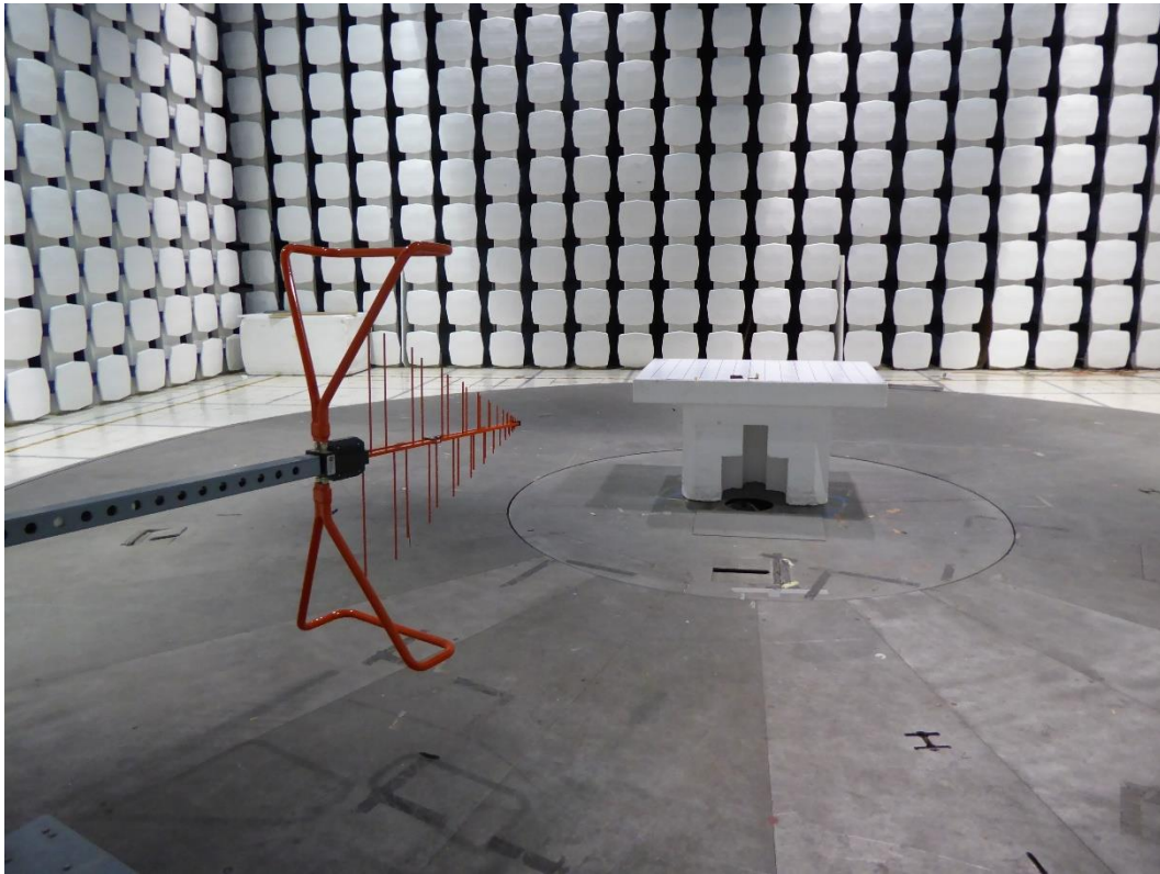
Figure 12 – 30 – 1000 MHz 3 meter Radiated Setup
