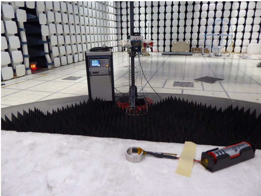
Figure 13 – 1 – 26.5 GHz 3 meter Radiated Setup
