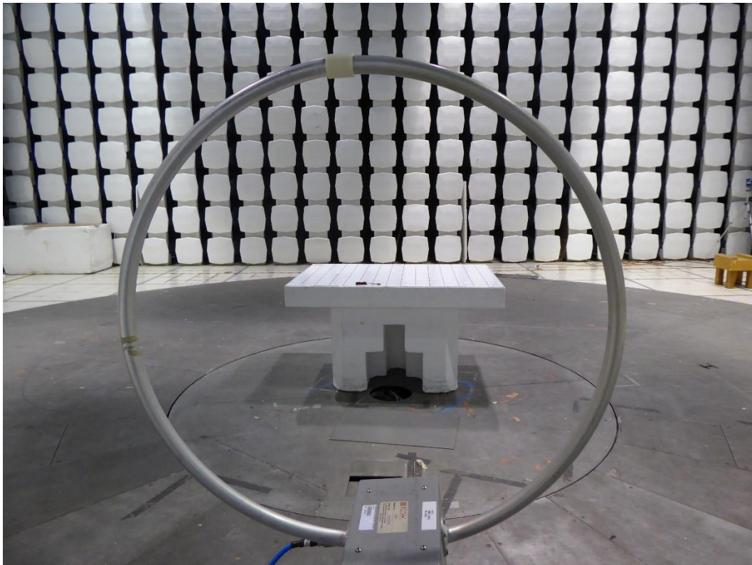
Figure 10 – 9k – 30MHz 3 meter Radiated Setup
