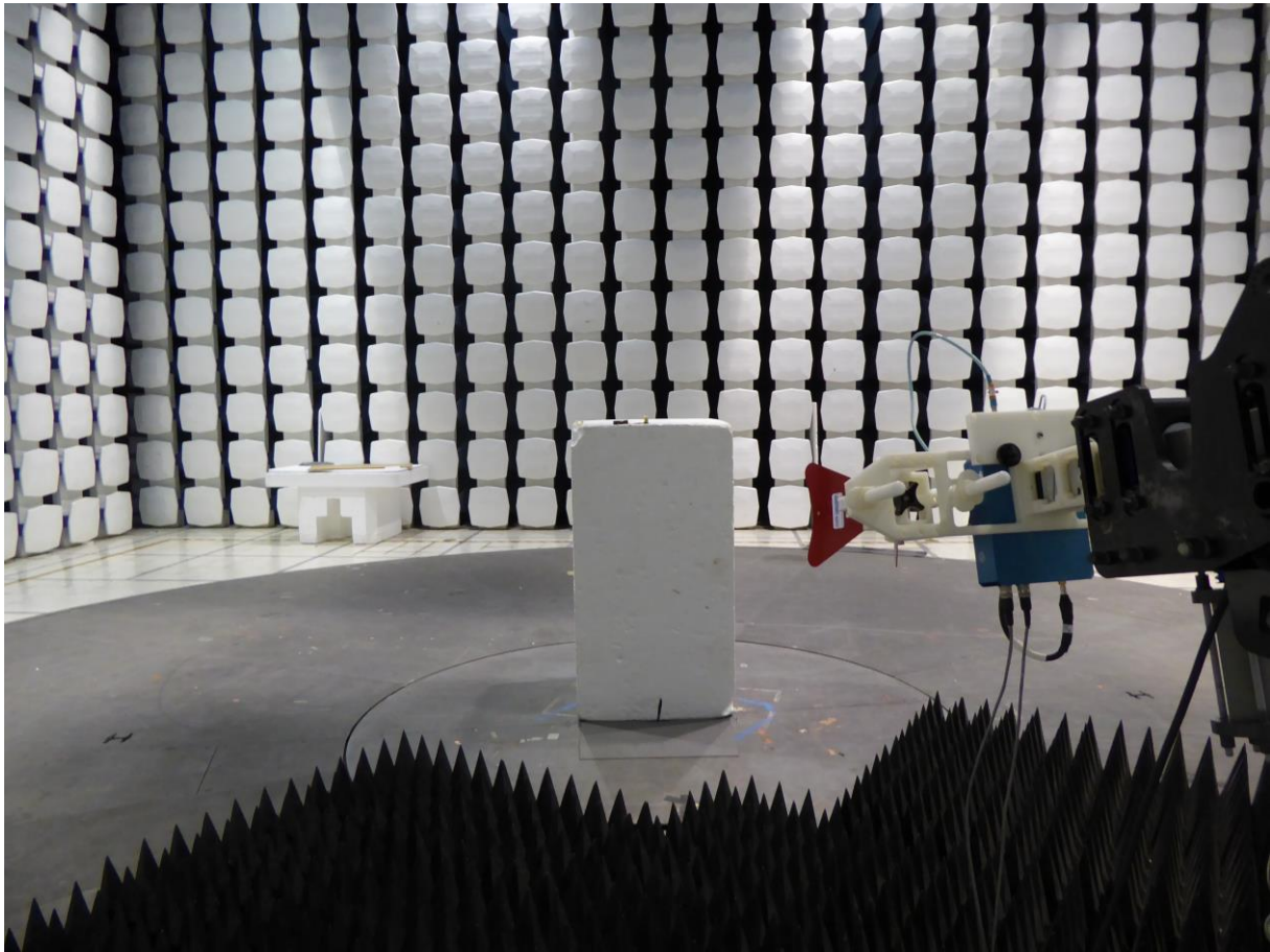
Figure 14 – 1 – 26.5 GHz 3 meter Radiated Test Setup
