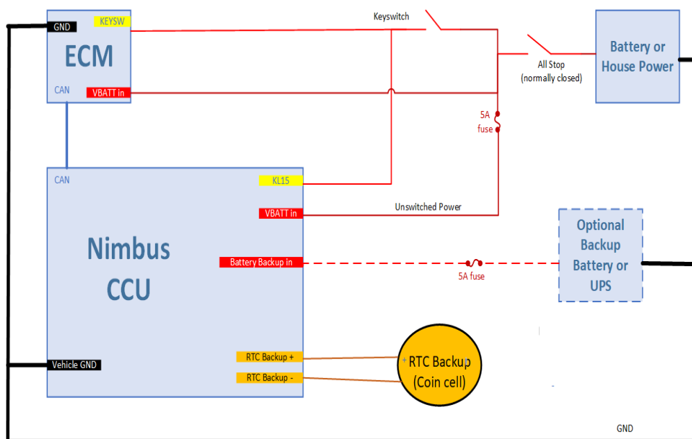
Figure 4 Grounding Scheme
