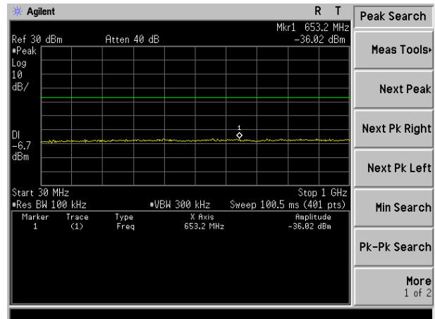
802.11n20-Middle Channel 2437MHz
