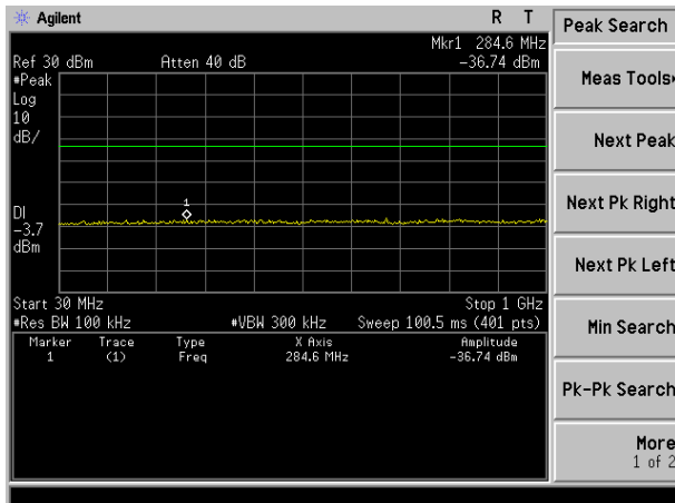
802.11b-High Channel 2462MHz
