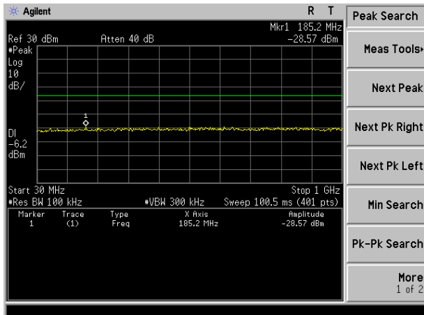
802.11n20-Low Channel 2412MHz
