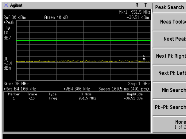
802.11b-Low Channel 2412MHz
