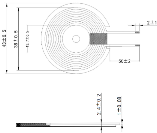
Mobile Phone coil:
