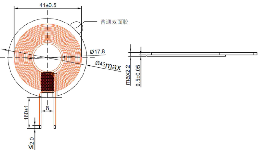
Apple Watch coil:
