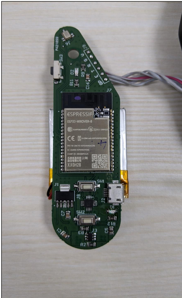
Photo 1: PCB Front view
