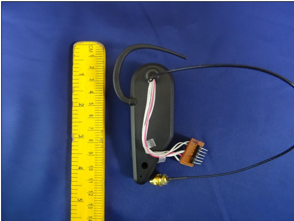
Photo3: EUT dimensional view
