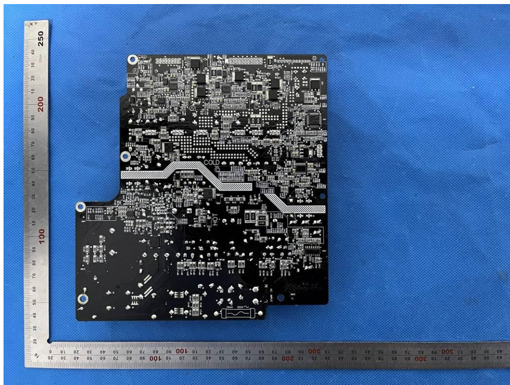
INTERNAL VIEW-2 OF EUT(power board: MPL_360-FM-3S)
