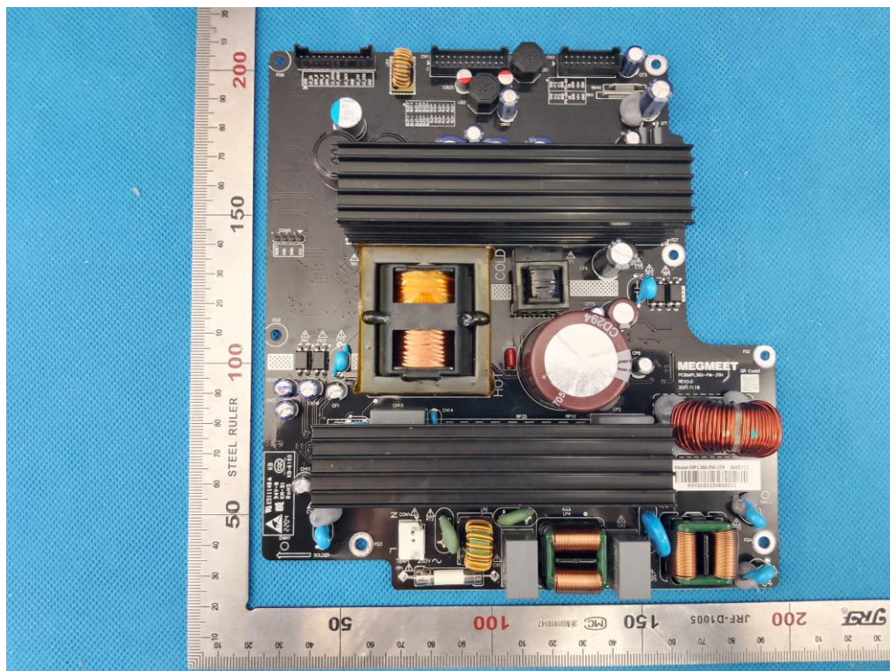
INTERNAL VIEW-4 OF EUT (power board: MPL_360-FM-3TH)
