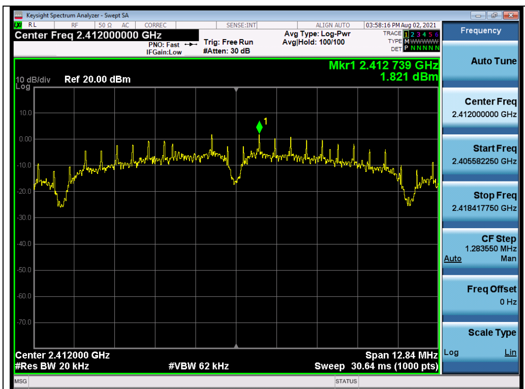
Test_Graph_802.11b_ANT2_2412_1Mbps_PSD
