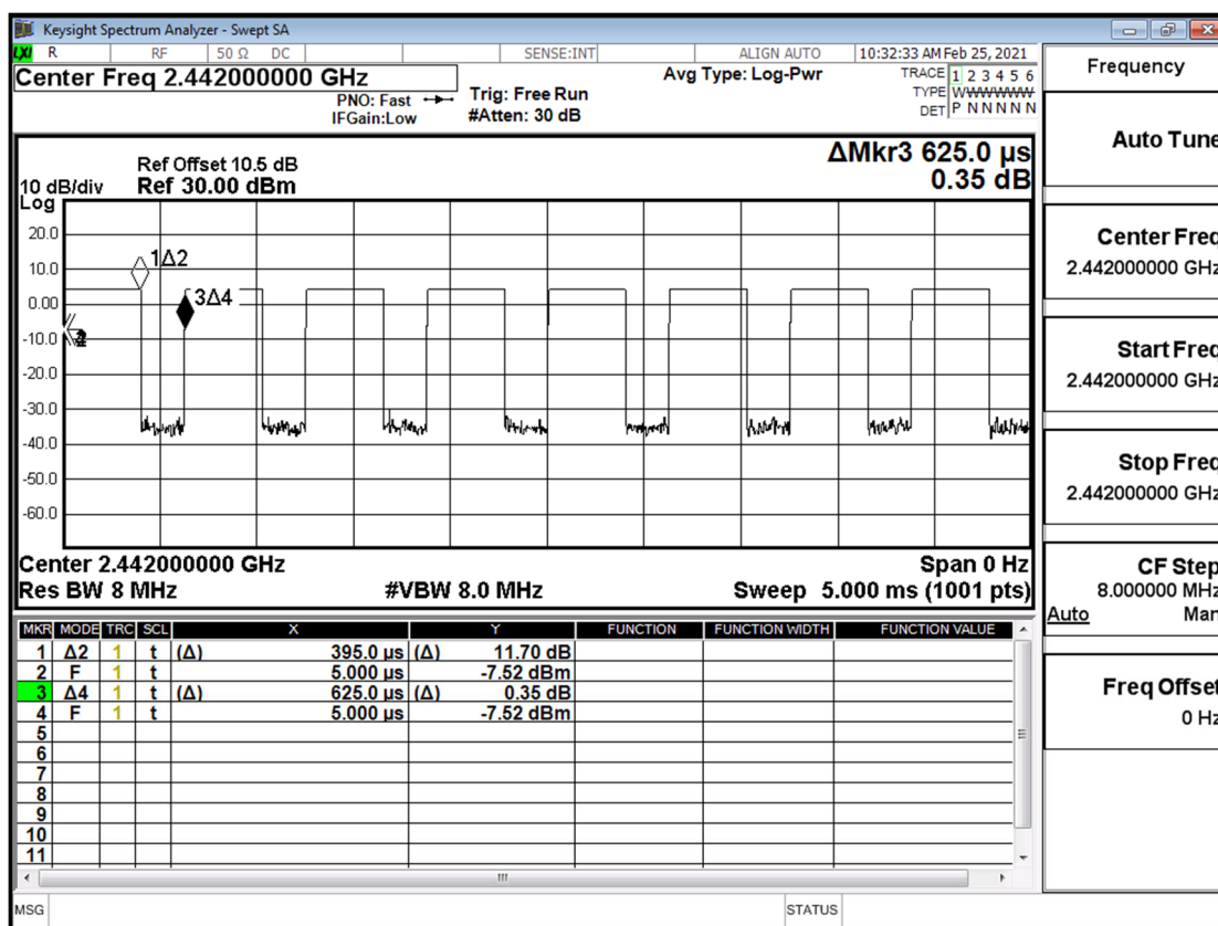
Duty Cycle_BLE_1M_MidCH20-2442
