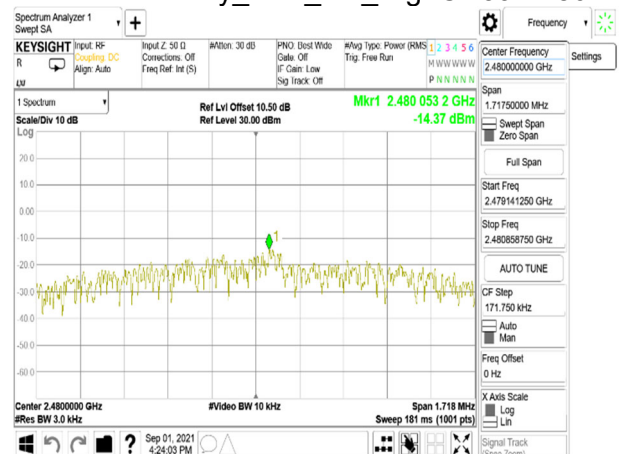
Power Density_BLE_2M_HighCH39-2480
