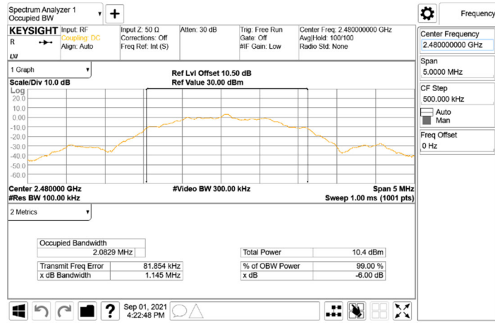
OBW 6dB_BLE_2M_HighCH39-2480
