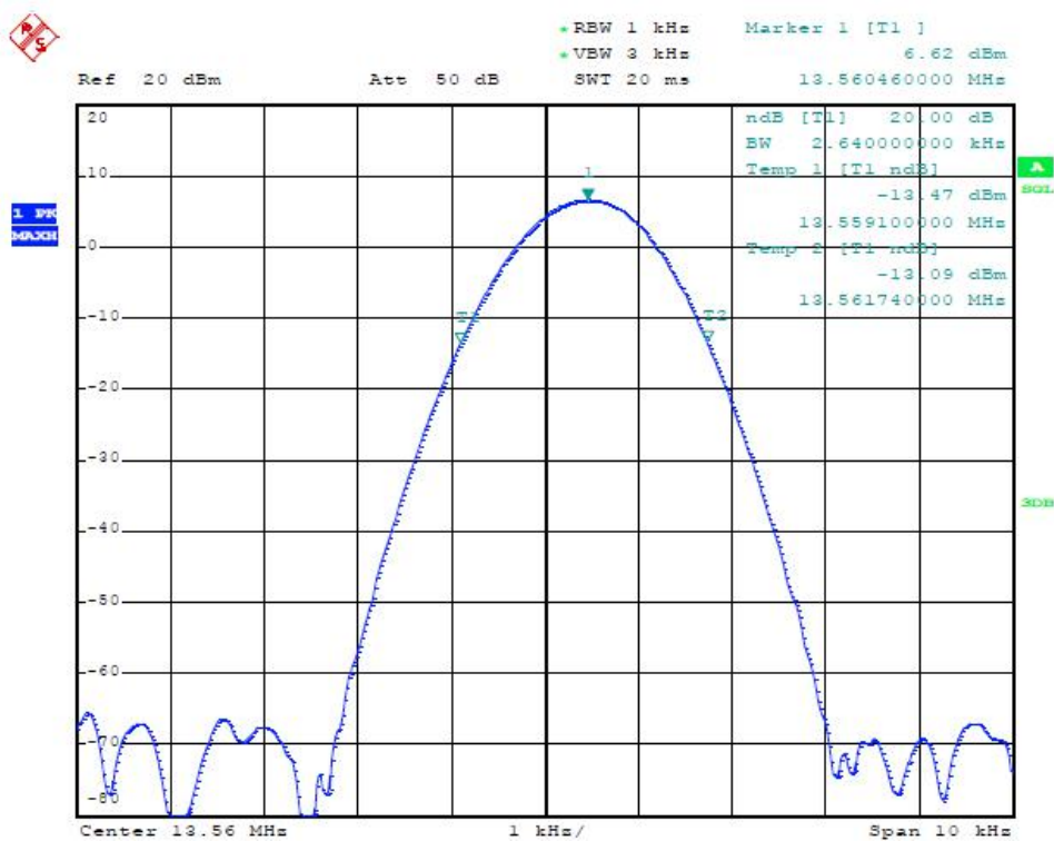
20dB Bandwidth
