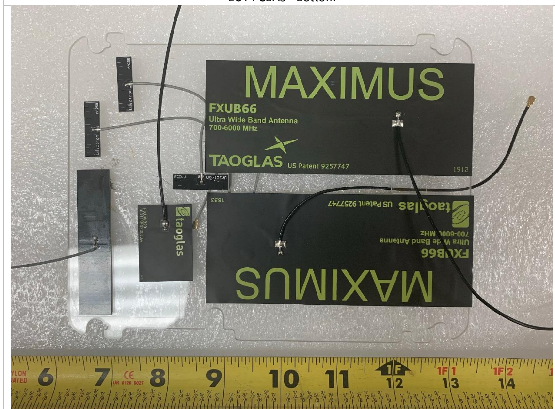
EUT Antenna (TX and RX) - Top
