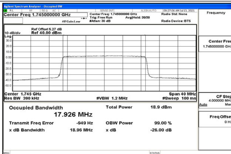
Band4-20MHz-16QAM-20300-100RB#0-17.926
