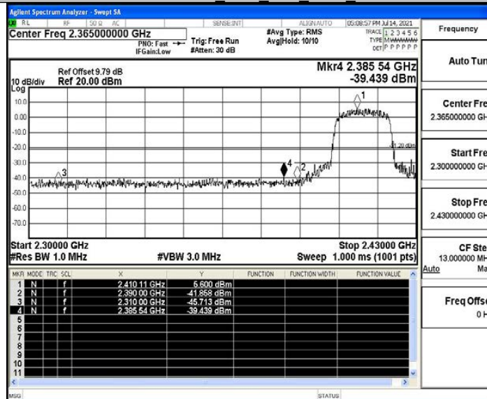
11N20SISO_Ant1_Low_2412_Peak
