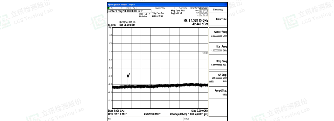
Band71_20MHz_16QAM_133222_1RB#0_1000~3000_1000~3000
