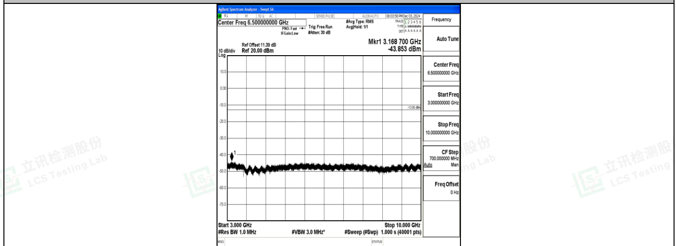
Band71_20MHz_QPSK_133372_1RB#0_3000~10000_3000~10000
