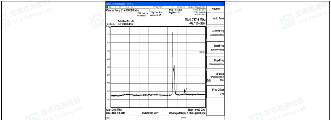
Band71_20MHz_QPSK_133222_1RB#0_30~1000_30~1000
