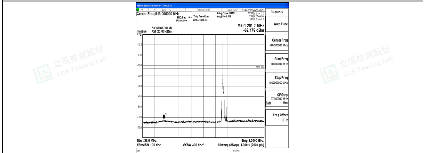
Band71_20MHz_16QAM_133222_1RB#0_30~1000_30~1000
