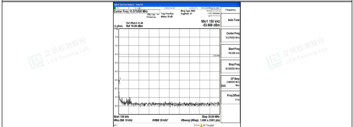
Band71_15MHz_QPSK_133197_1RB#0_0.15~30_0.15~30
