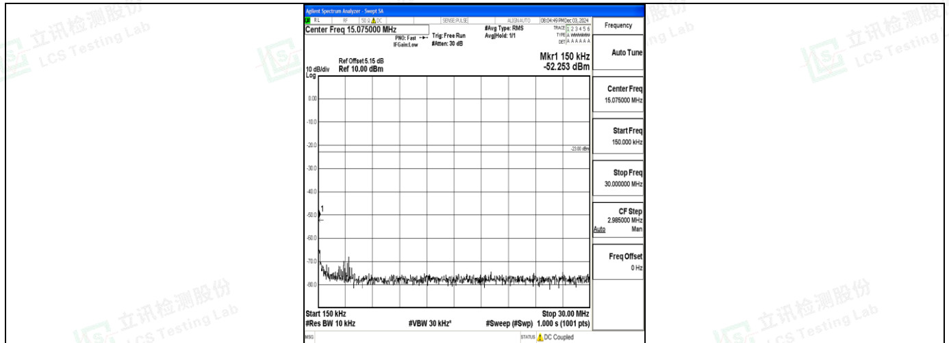
Band71_20MHz_16QAM_133372_1RB#0_0.15~30_0.15~30
