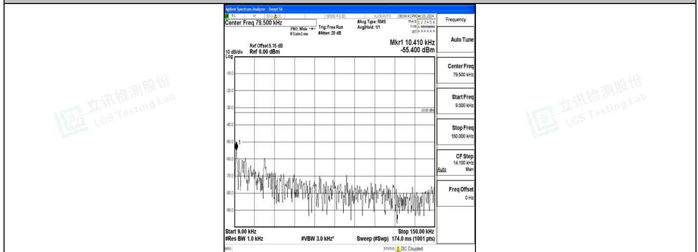
Band71_20MHz_16QAM_133372_1RB#0_0.009~0.15_0.009~0.15
