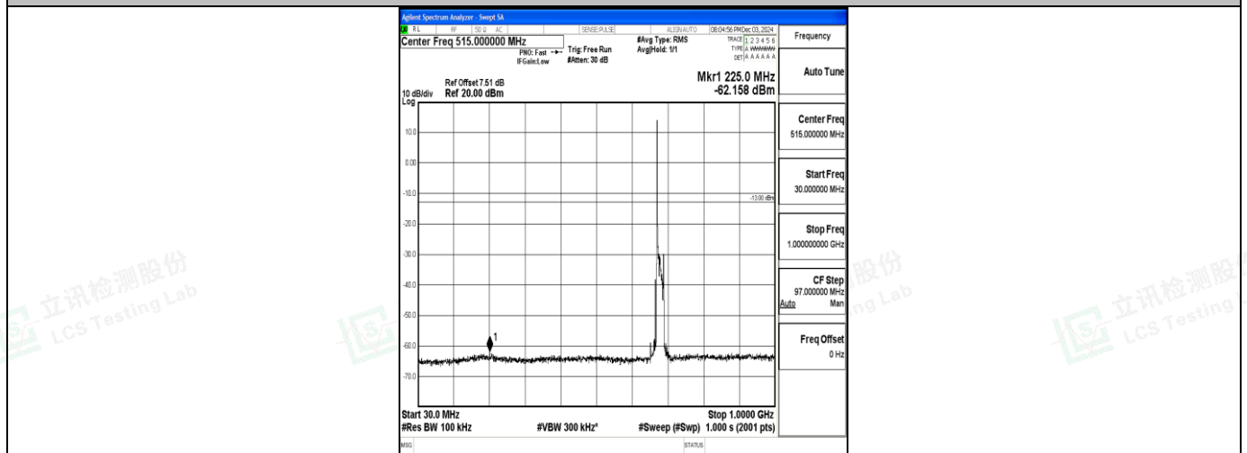
Band71_20MHz_16QAM_133372_1RB#0_30~1000_30~1000
