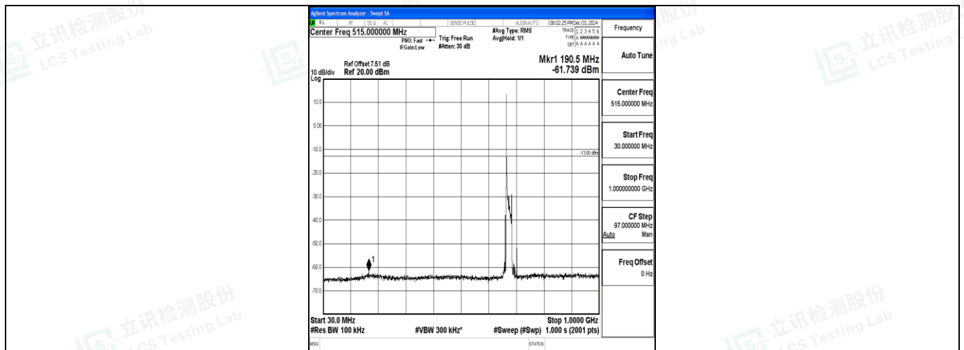
Band71_20MHz_16QAM_133322_1RB#0_30~1000_30~1000
