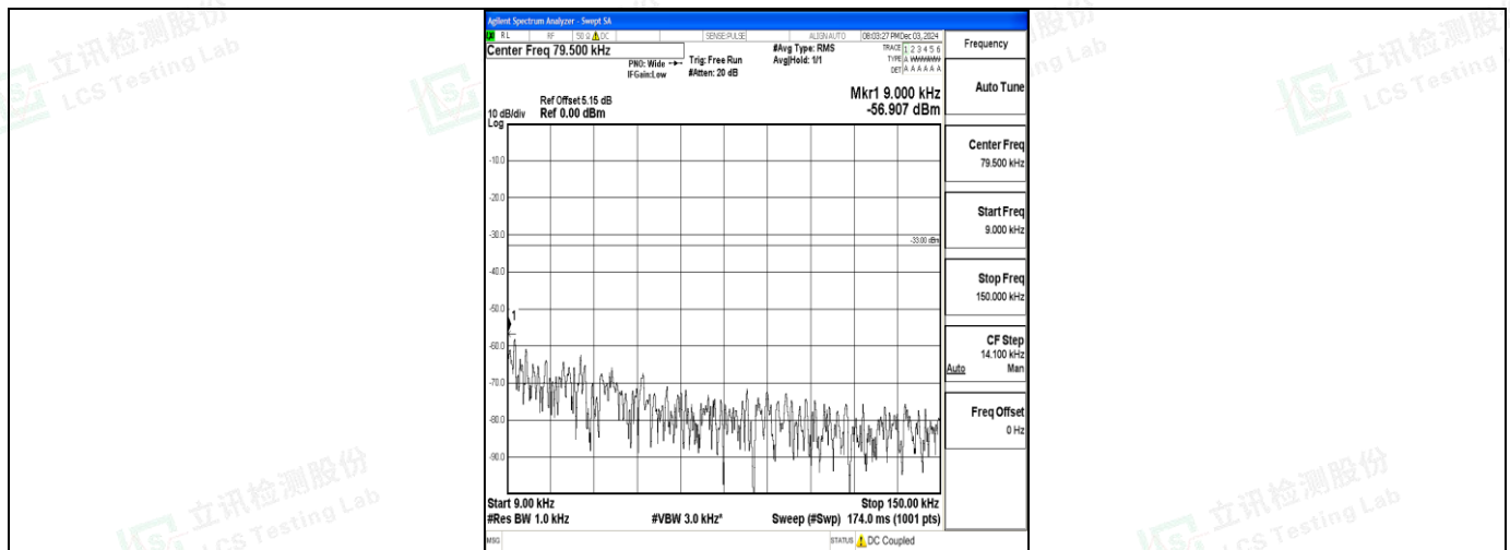
Band71_20MHz_QPSK_133372_1RB#0_0.009~0.15_0.009~0.15
