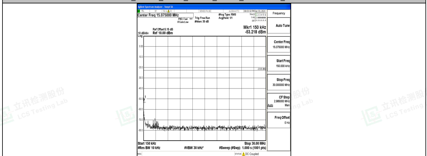
Band71_20MHz_QPSK_133372_1RB#0_0.15~30_0.15~30
