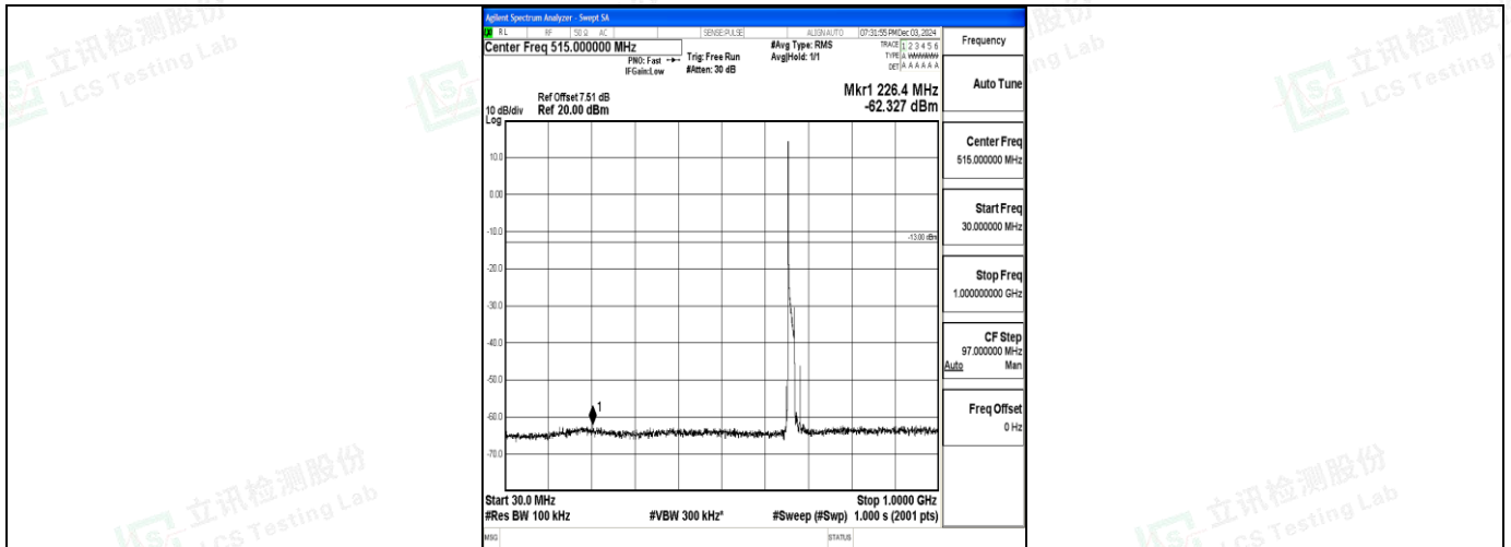
Band71_15MHz_QPSK_133197_1RB#0_30~1000_30~1000
