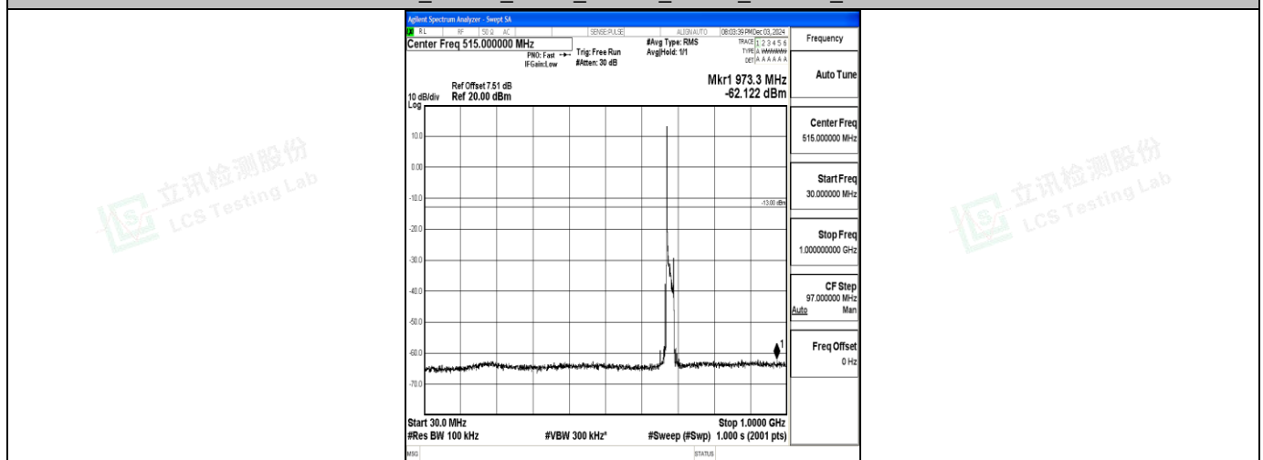
Band71_20MHz_QPSK_133372_1RB#0_30~1000_30~1000
