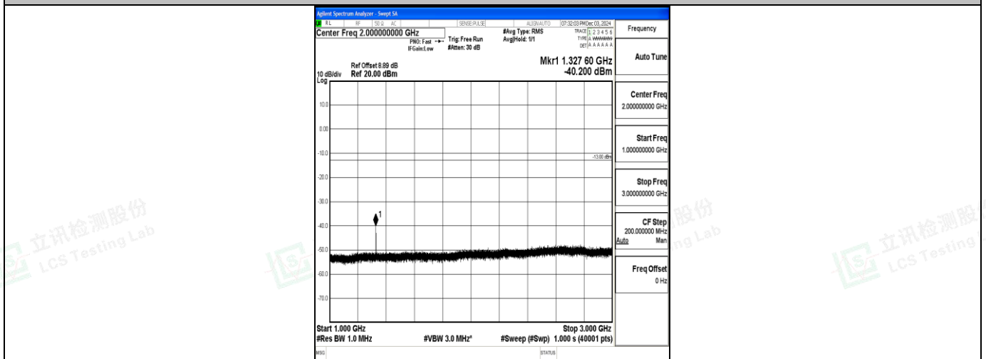
Band71_15MHz_QPSK_133197_1RB#0_1000~3000_1000~3000
