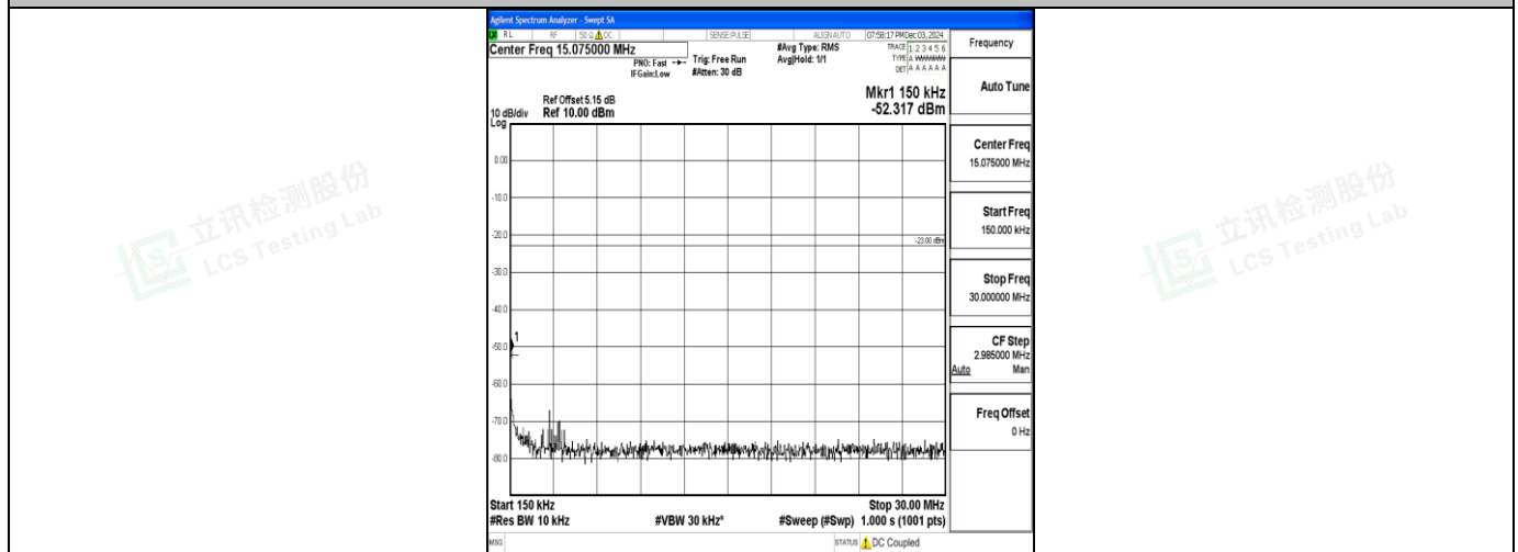
Band71_20MHz_QPSK_133222_1RB#0_0.15~30_0.15~30
