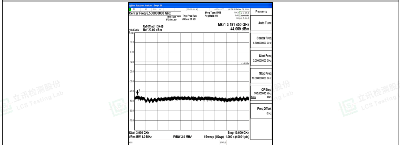
Band71_20MHz_16QAM_133222_1RB#0_3000~10000_3000~10000
