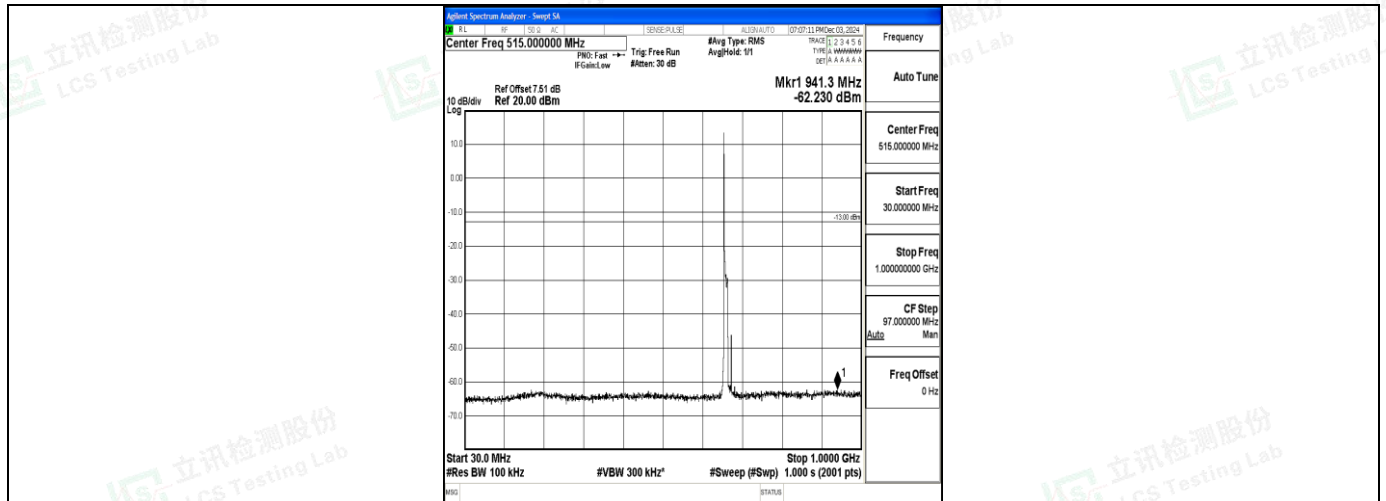
Band71_10MHz_QPSK_133172_1RB#0_30~1000_30~1000
