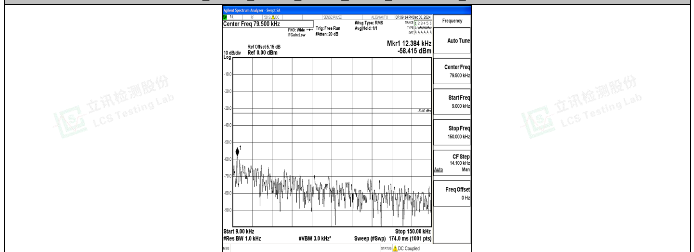
Band71_10MHz_QPSK_133297_1RB#0_0.009~0.15_0.009~0.15
