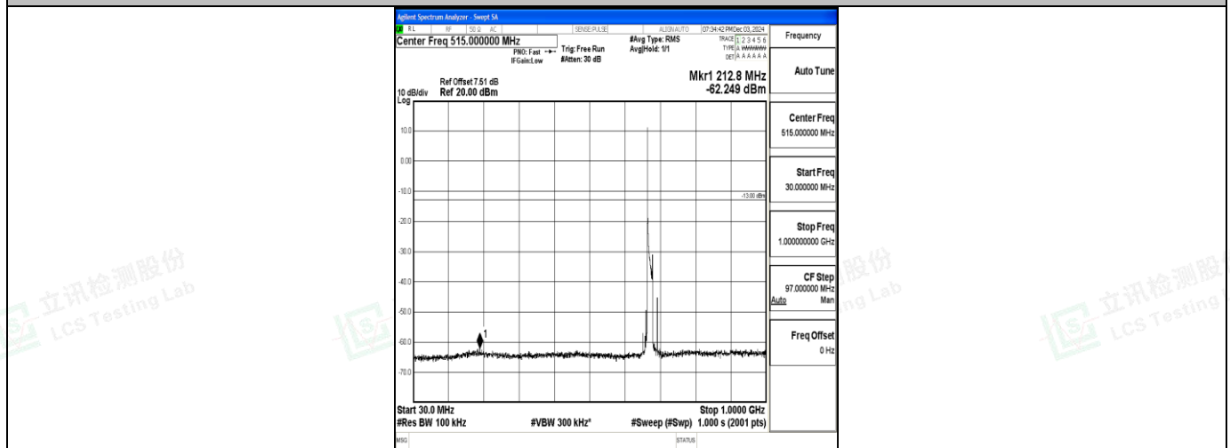
Band71_15MHz_QPSK_133297_1RB#0_30~1000_30~1000
