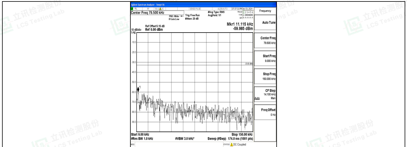
Band71_15MHz_QPSK_133397_1RB#0_0.009~0.15_0.009~0.15
