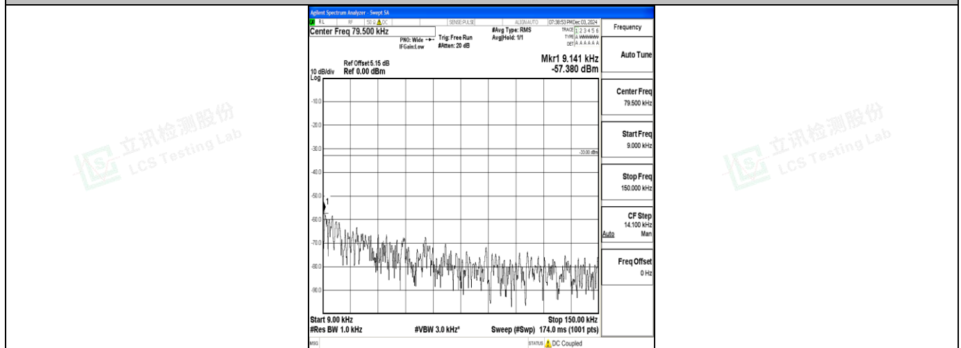
Band71_15MHz_16QAM_133397_1RB#0_0.009~0.15_0.009~0.15
