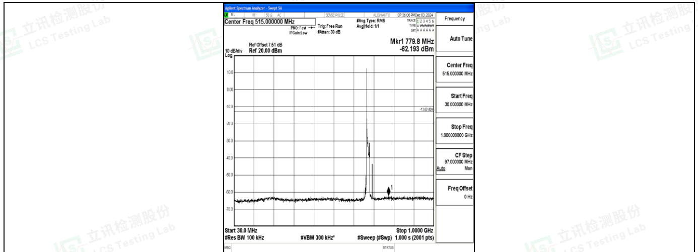
Band71_15MHz_16QAM_133297_1RB#0_30~1000_30~1000
