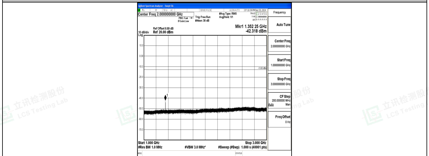
Band71_10MHz_16QAM_133297_1RB#0_1000~3000_1000~3000
