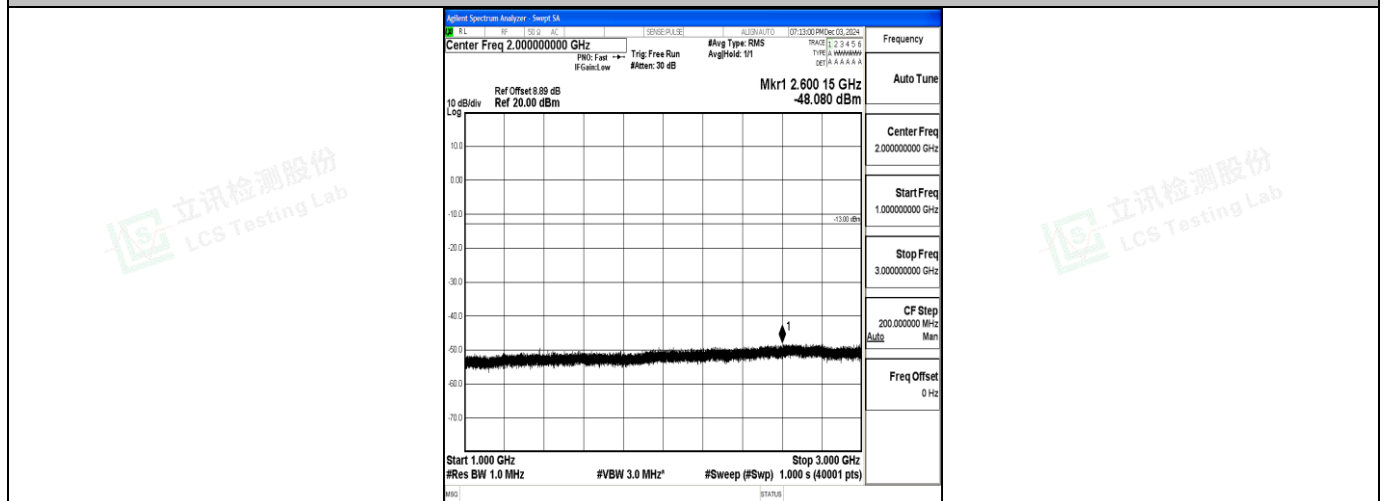
Band71_10MHz_16QAM_133422_1RB#0_1000~3000_1000~3000
