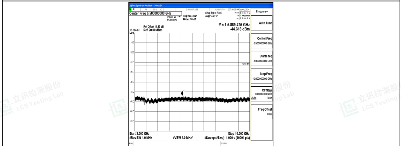
Band71_15MHz_QPSK_133397_1RB#0_3000~10000_3000~10000
