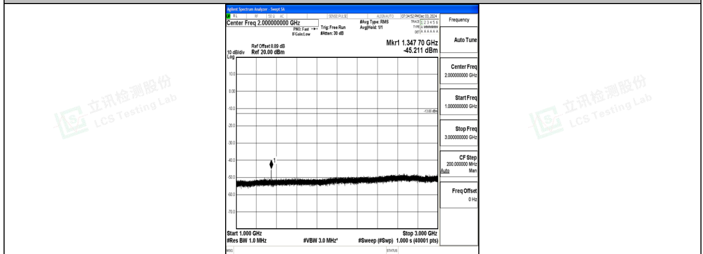
Band71_15MHz_QPSK_133297_1RB#0_1000~3000_1000~3000
