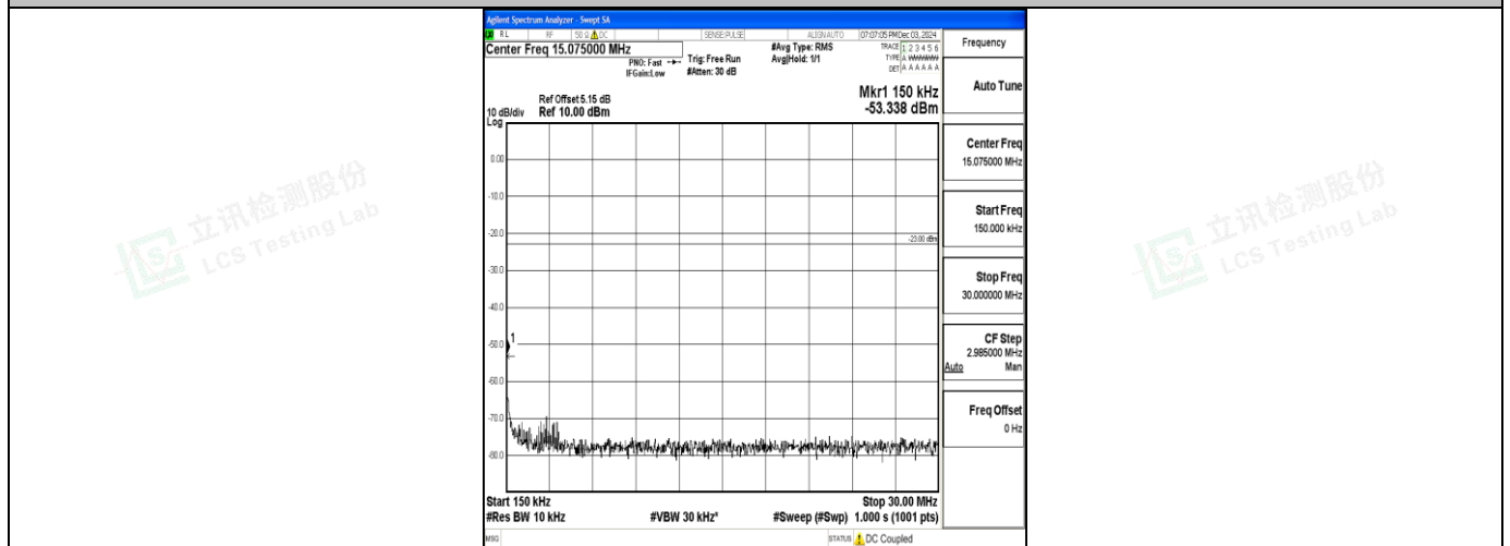
Band71_10MHz_QPSK_133172_1RB#0_0.15~30_0.15~30
