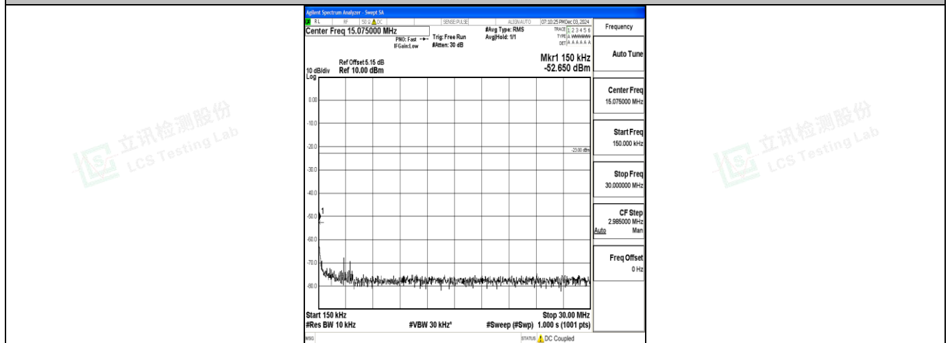
Band71_10MHz_16QAM_133297_1RB#0_0.15~30_0.15~30
