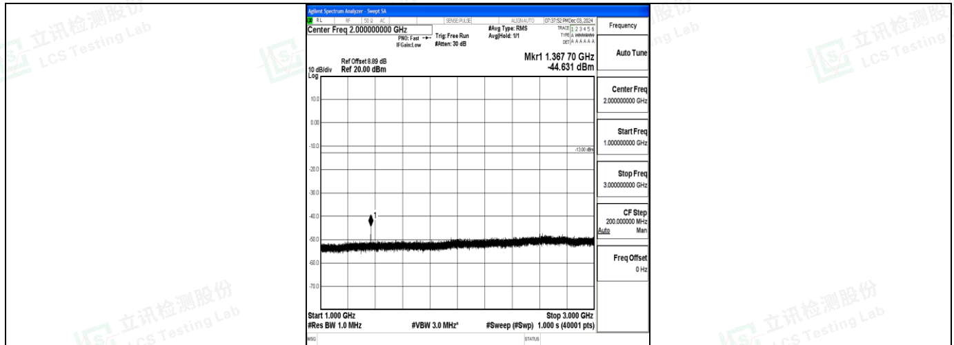
Band71_15MHz_QPSK_133397_1RB#0_1000~3000_1000~3000
