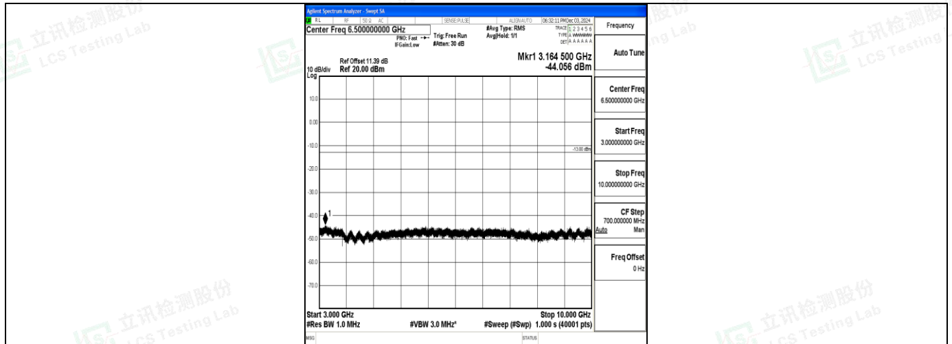
Band71_5MHz_QPSK_133297_1RB#0_3000~10000_3000~10000
