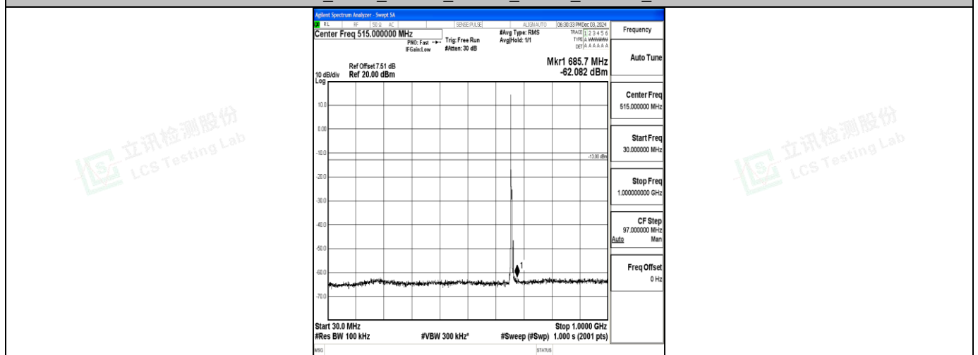
Band71_5MHz_16QAM_133147_1RB#0_30~1000_30~1000
