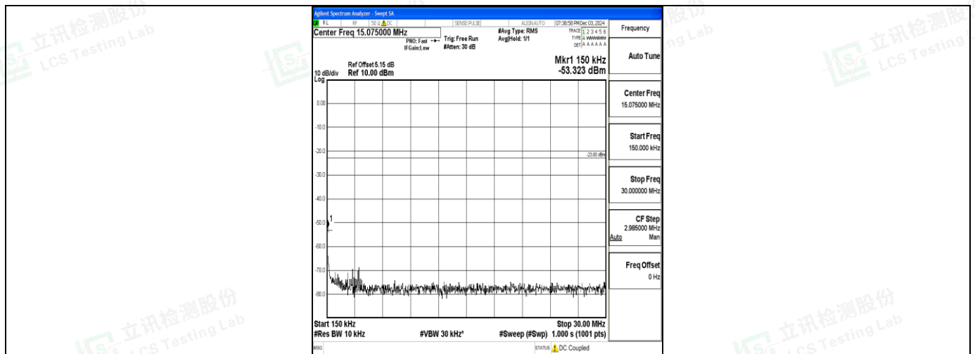
Band71_15MHz_16QAM_133397_1RB#0_0.15~30_0.15~30
