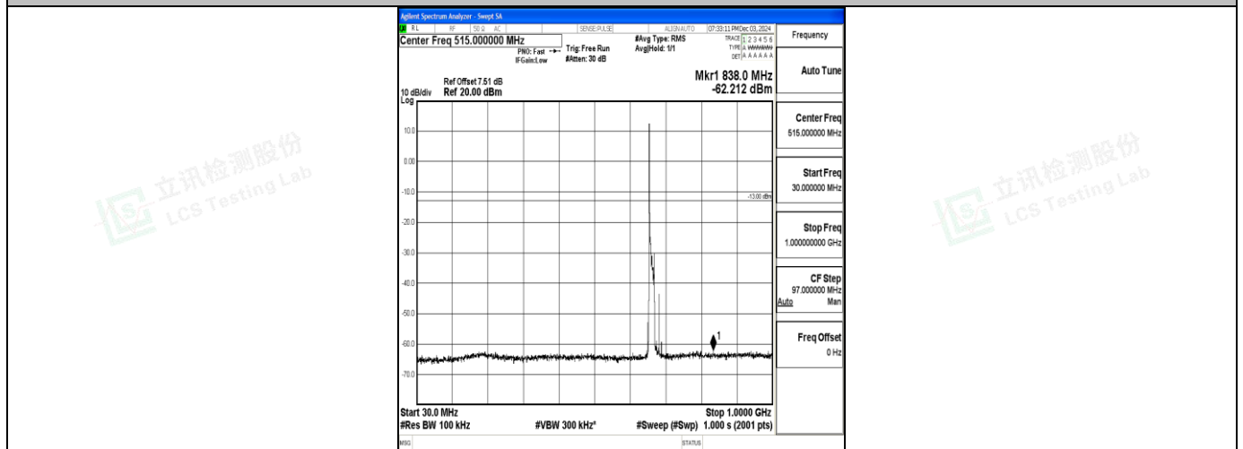
Band71_15MHz_16QAM_133197_1RB#0_30~1000_30~1000
