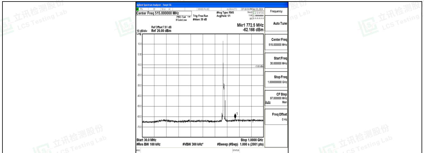
Band71_10MHz_16QAM_133297_1RB#0_30~1000_30~1000
