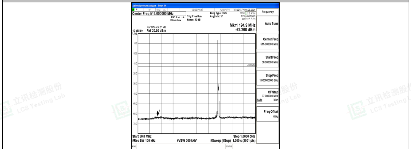
Band71_10MHz_16QAM_133422_1RB#0_30~1000_30~1000
