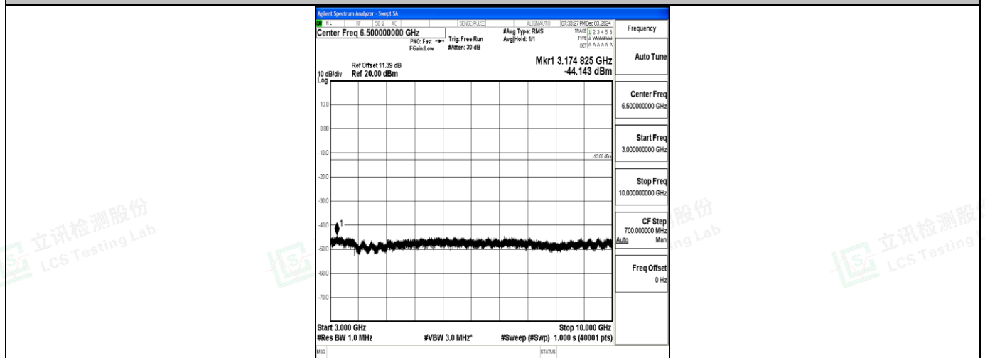
Band71_15MHz_16QAM_133197_1RB#0_3000~10000_3000~10000
