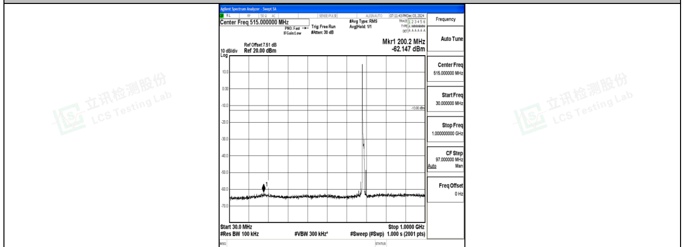
Band71_10MHz_QPSK_133422_1RB#0_30~1000_30~1000
