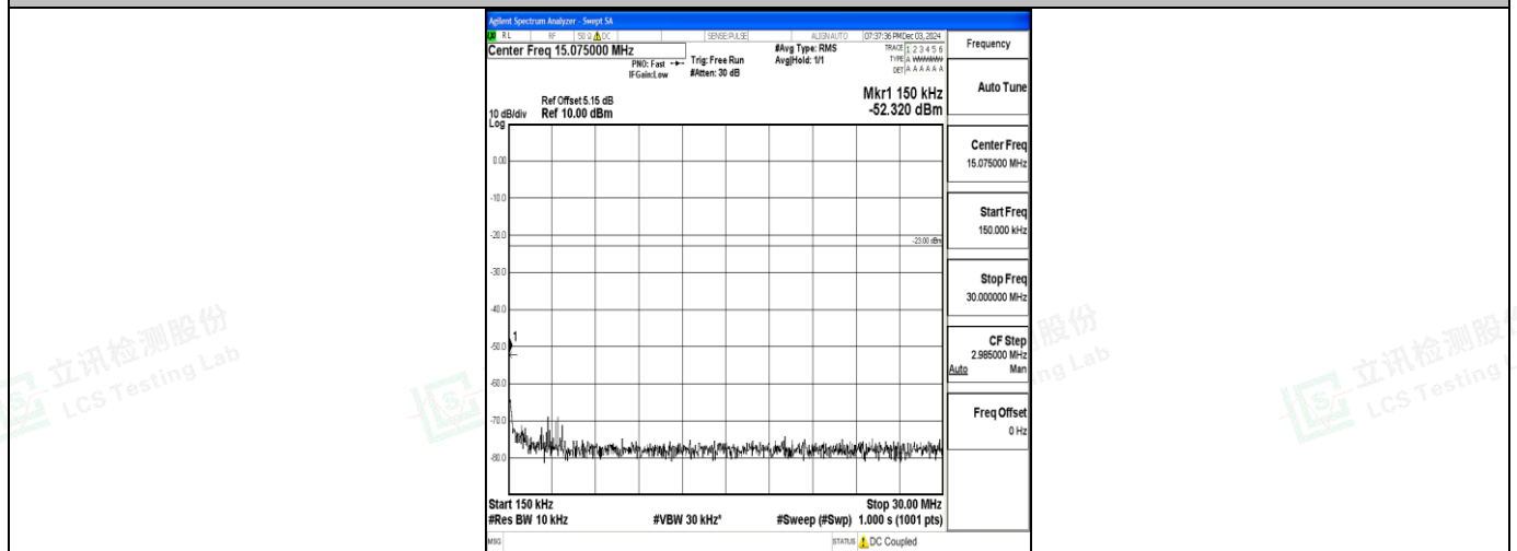
Band71_15MHz_QPSK_133397_1RB#0_0.15~30_0.15~30
