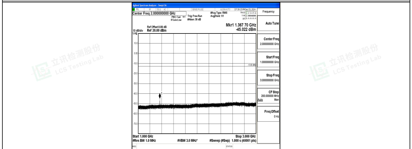
Band71_15MHz_16QAM_133397_1RB#0_1000~3000_1000~3000
