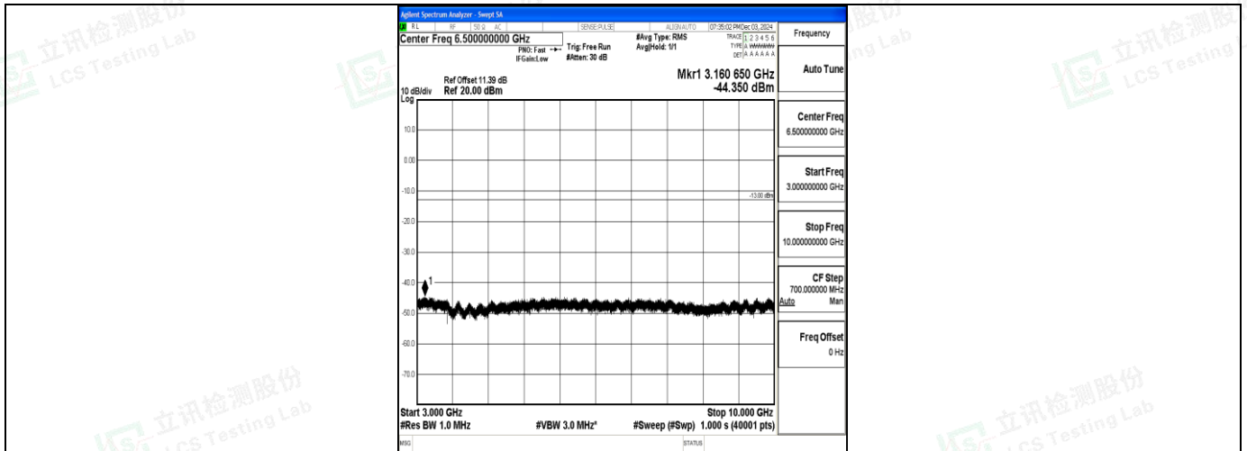
Band71_15MHz_QPSK_133297_1RB#0_3000~10000_3000~10000
