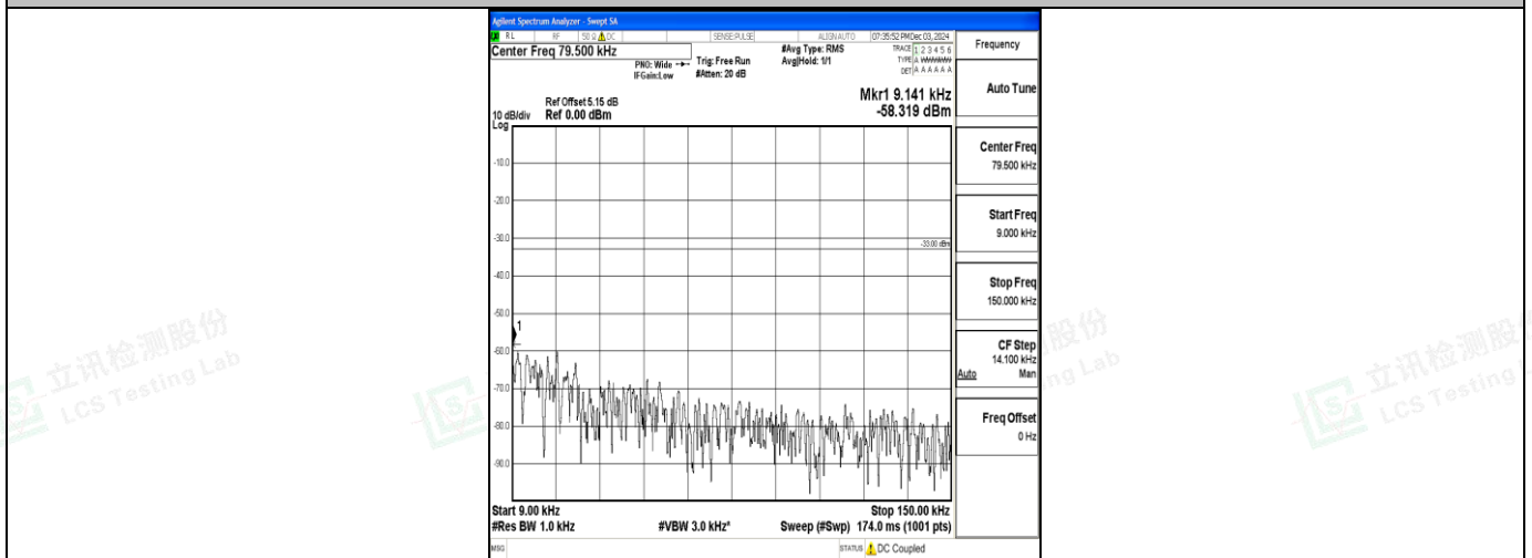
Band71_15MHz_16QAM_133297_1RB#0_0.009~0.15_0.009~0.15
