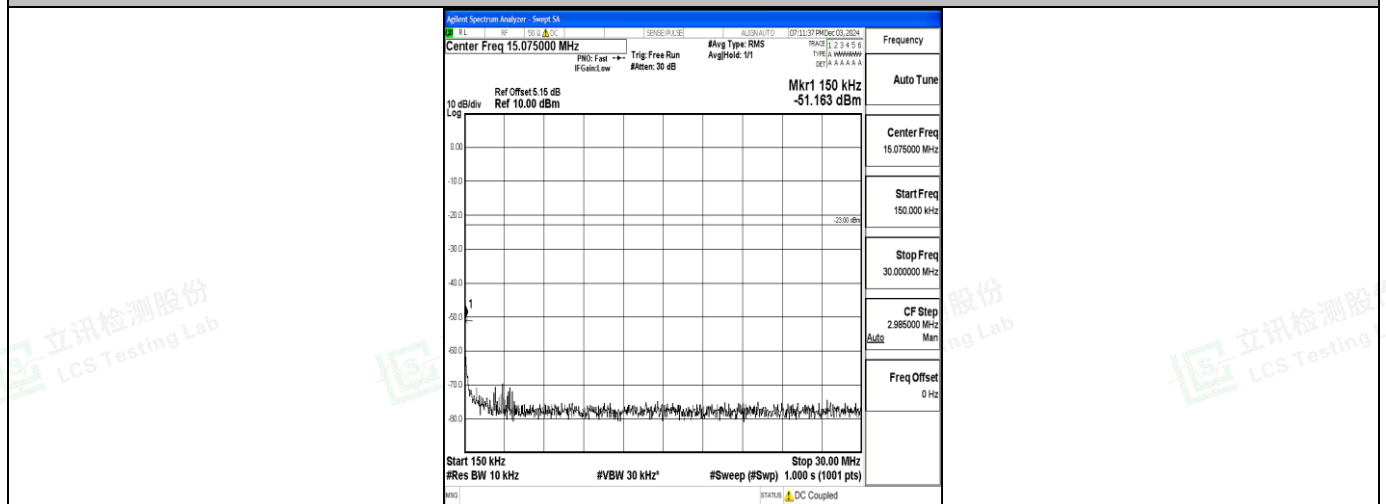
Band71_10MHz_QPSK_133422_1RB#0_0.15~30_0.15~30
