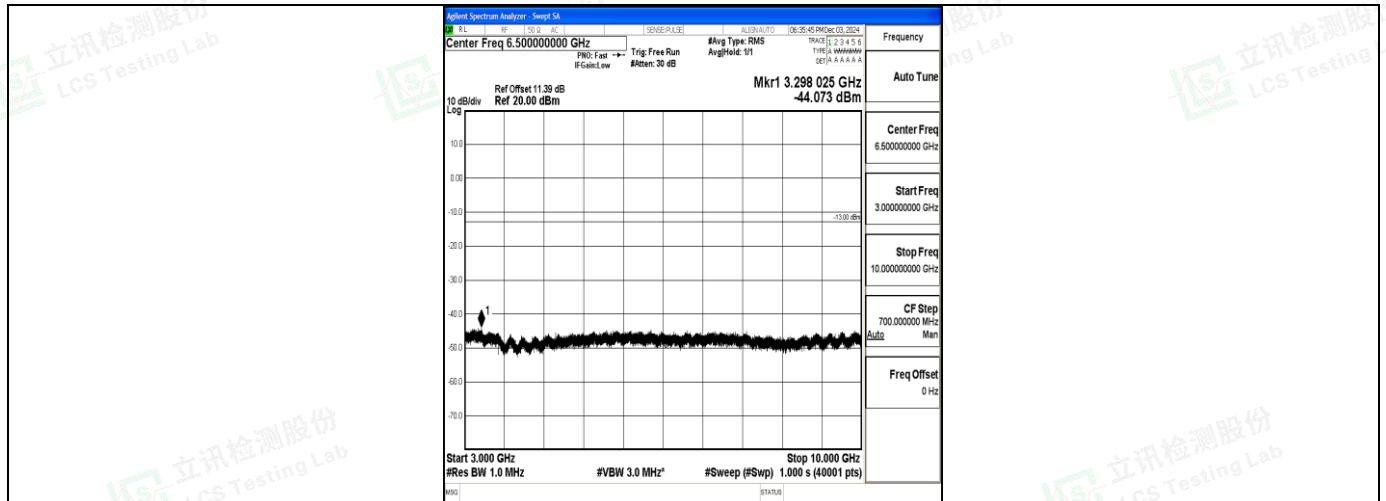
Band71_5MHz_16QAM_133447_1RB#0_3000~10000_3000~10000
