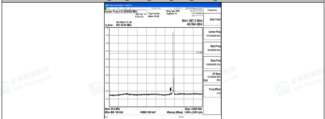
Band71_5MHz_16QAM_133447_1RB#0_30~1000_30~1000
