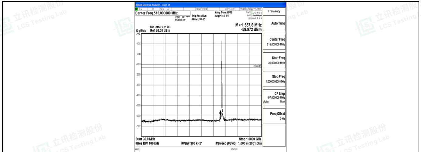
Band71_5MHz_16QAM_133297_1RB#0_30~1000_30~1000
