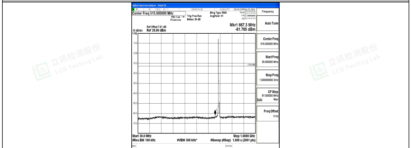
Band71_5MHz_QPSK_133447_1RB#0_30~1000_30~1000
