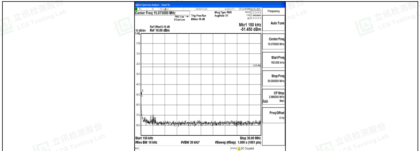
Band71_10MHz_16QAM_133422_1RB#0_0.15~30_0.15~30
