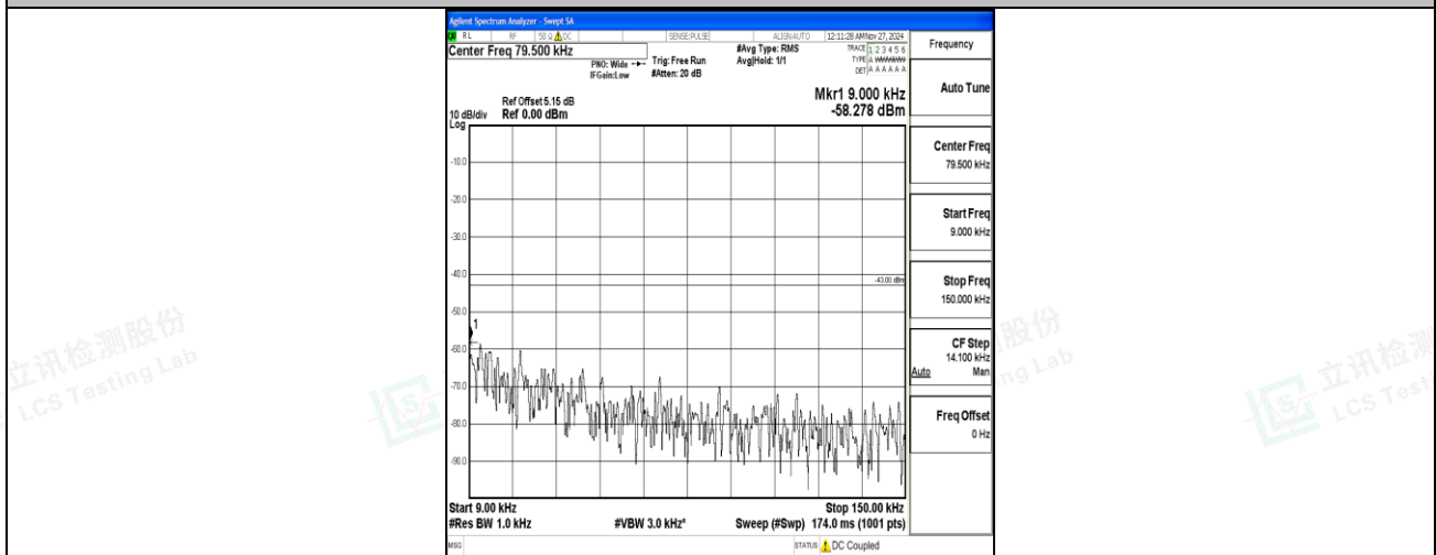
Band66_3MHz_16QAM_131987_1RB#0_0.009~0.15_0.009~0.15
