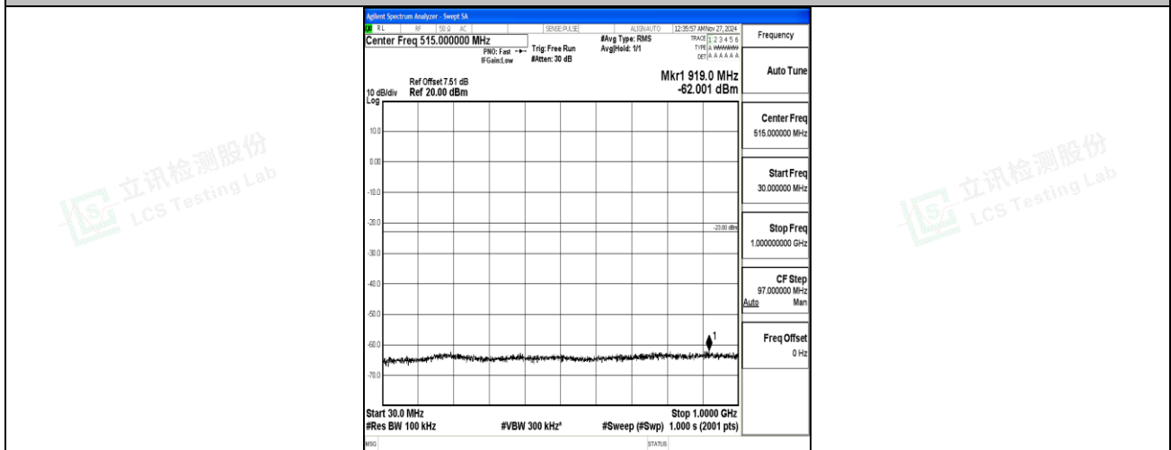
Band66_5MHz_QPSK_132322_1RB#0_30~1000_30~1000
