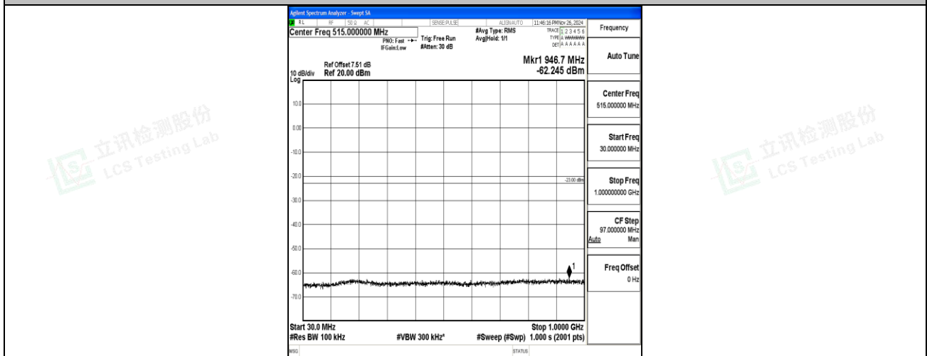
Band66_1.4MHz_16QAM_132665_1RB#0_30~1000_30~1000
