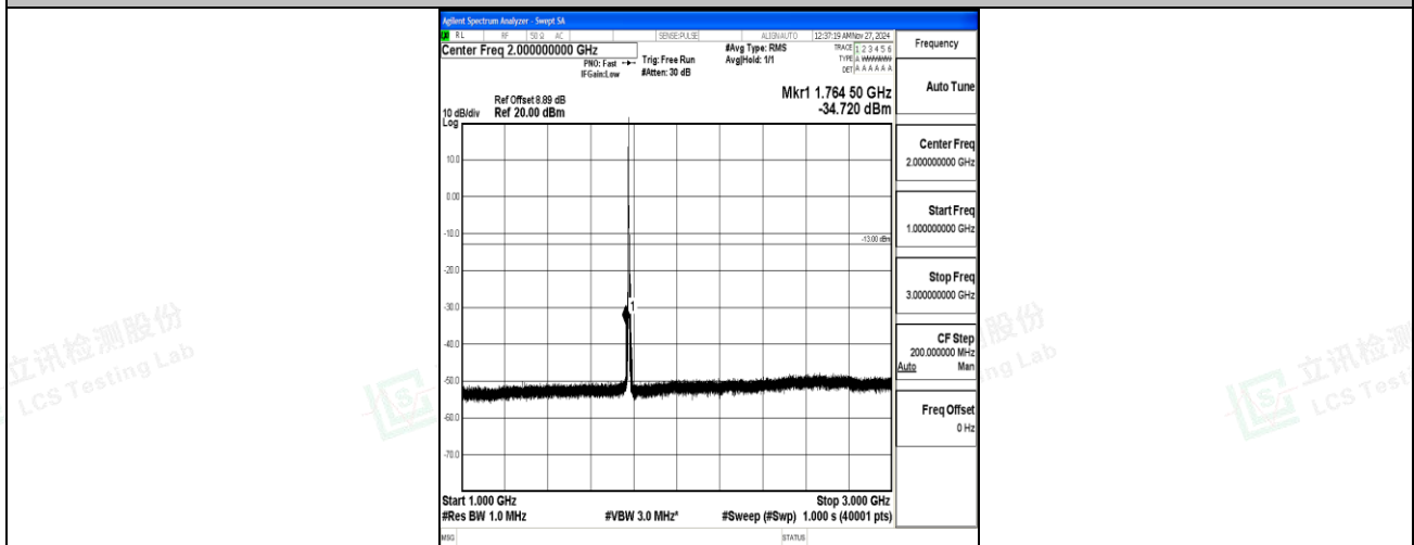
Band66_5MHz_QPSK_132647_1RB#0_1000~3000_1000~3000
