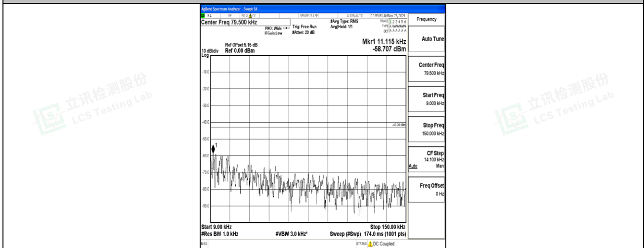
Band66_10MHz_16QAM_132322_1RB#0_0.009~0.15_0.009~0.15
