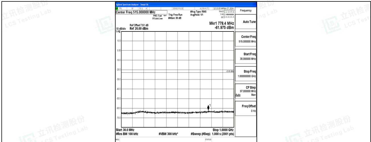
Band66_3MHz_QPSK_132657_1RB#0_30~1000_30~1000
