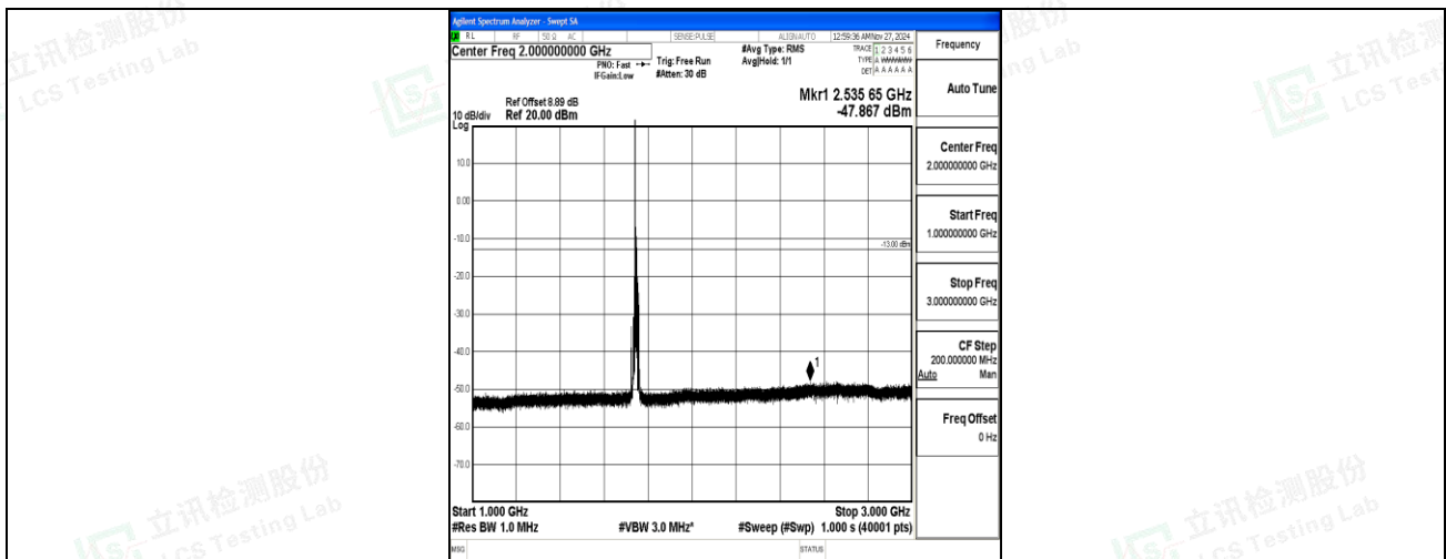
Band66_10MHz_QPSK_132322_1RB#0_1000~3000_1000~3000
