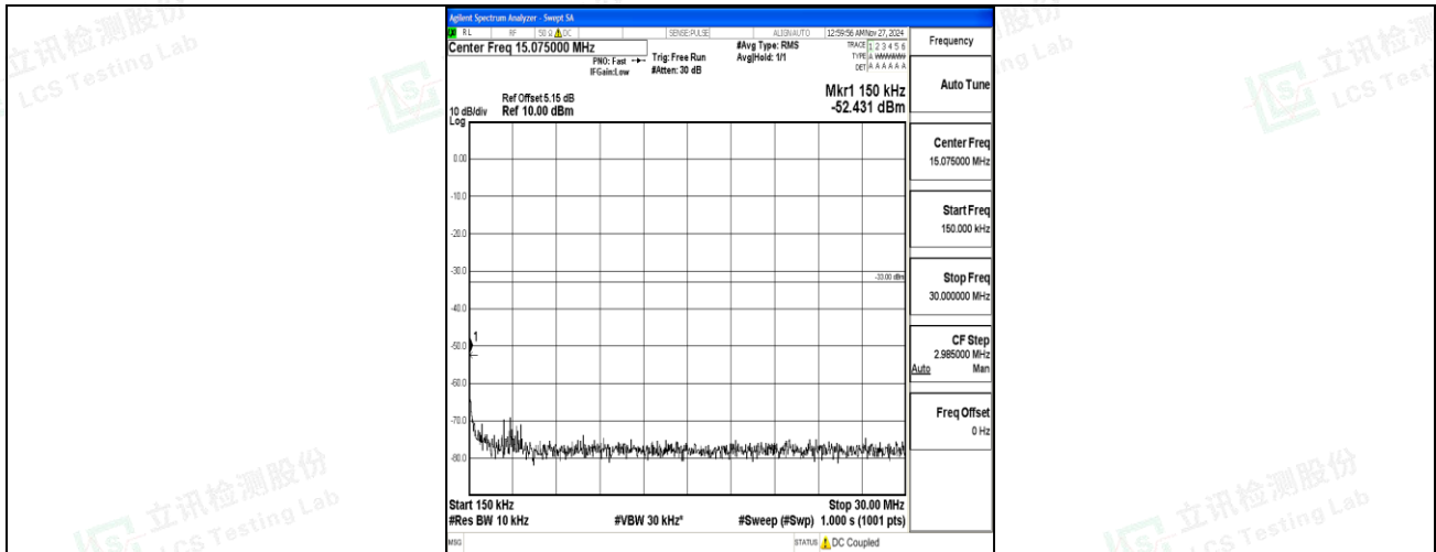
Band66_10MHz_16QAM_132322_1RB#0_0.15~30_0.15~30
