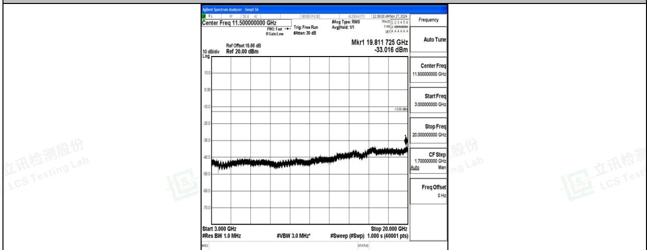
Band66_5MHz_16QAM_132647_1RB#0_3000~20000_3000~20000
