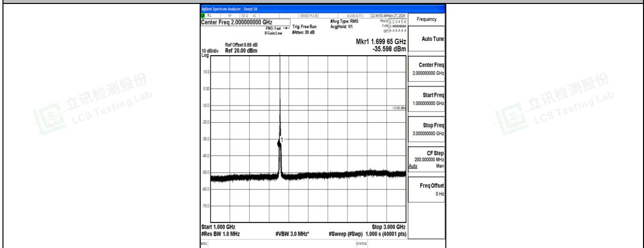
Band66_5MHz_QPSK_131997_1RB#0_1000~3000_1000~3000
