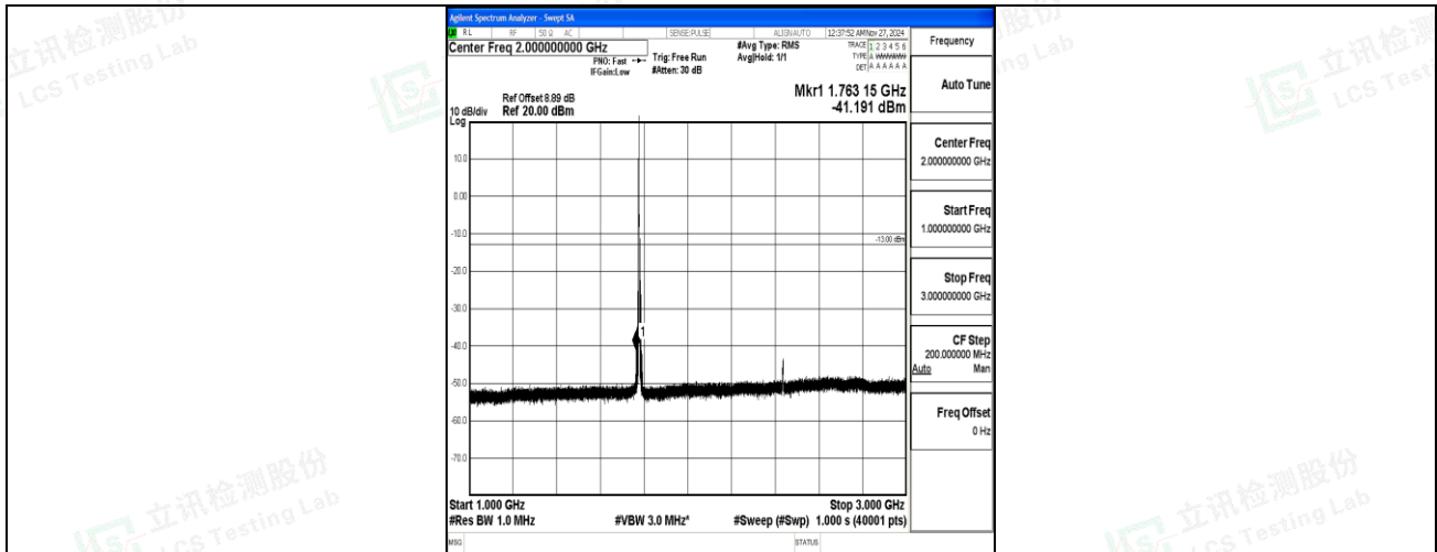
Band66_5MHz_16QAM_132647_1RB#0_1000~3000_1000~3000
