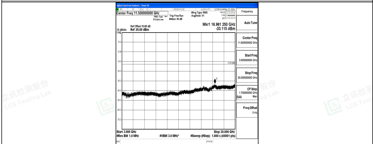
Band66_10MHz_QPSK_132322_1RB#0_3000~20000_3000~20000
