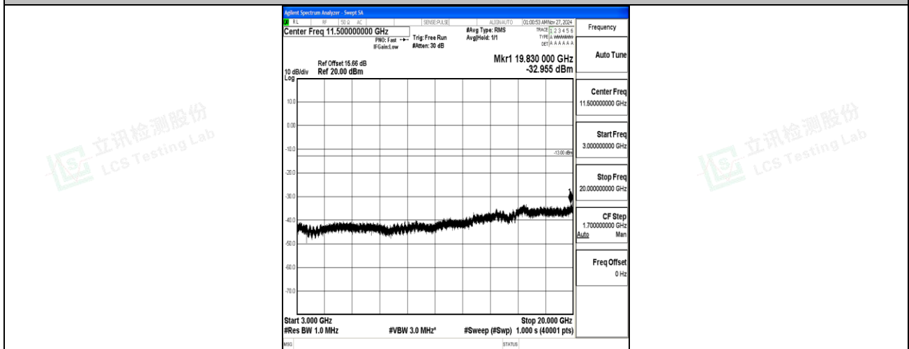
Band66_10MHz_QPSK_132622_1RB#0_3000~20000_3000~20000
