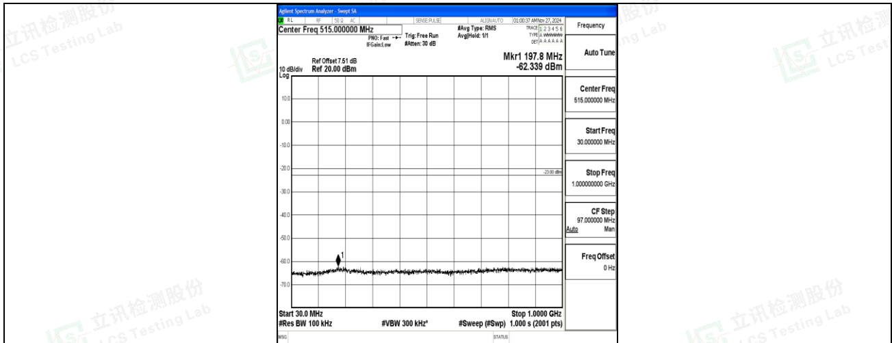
Band66_10MHz_QPSK_132622_1RB#0_30~1000_30~1000
