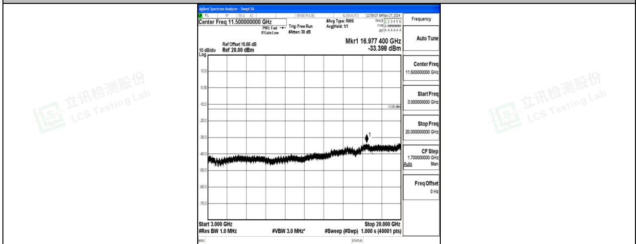
Band66_10MHz_16QAM_132022_1RB#0_3000~20000_3000~20000
