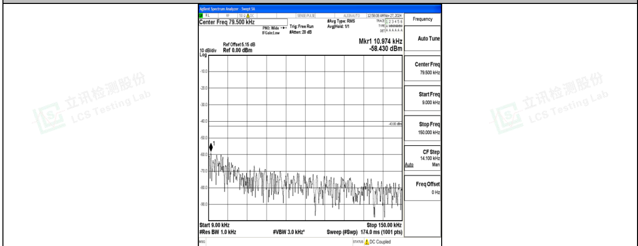
Band66_10MHz_QPSK_132022_1RB#0_0.009~0.15_0.009~0.15
