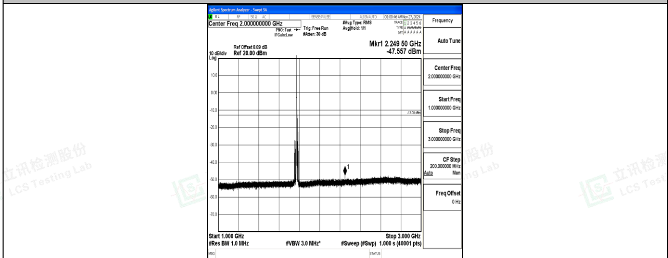
Band66_10MHz_QPSK_132622_1RB#0_1000~3000_1000~3000
