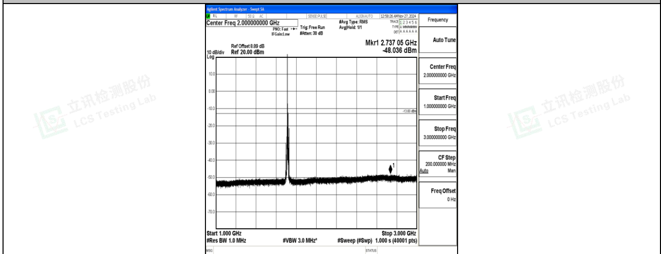
Band66_10MHz_QPSK_132022_1RB#0_1000~3000_1000~3000
