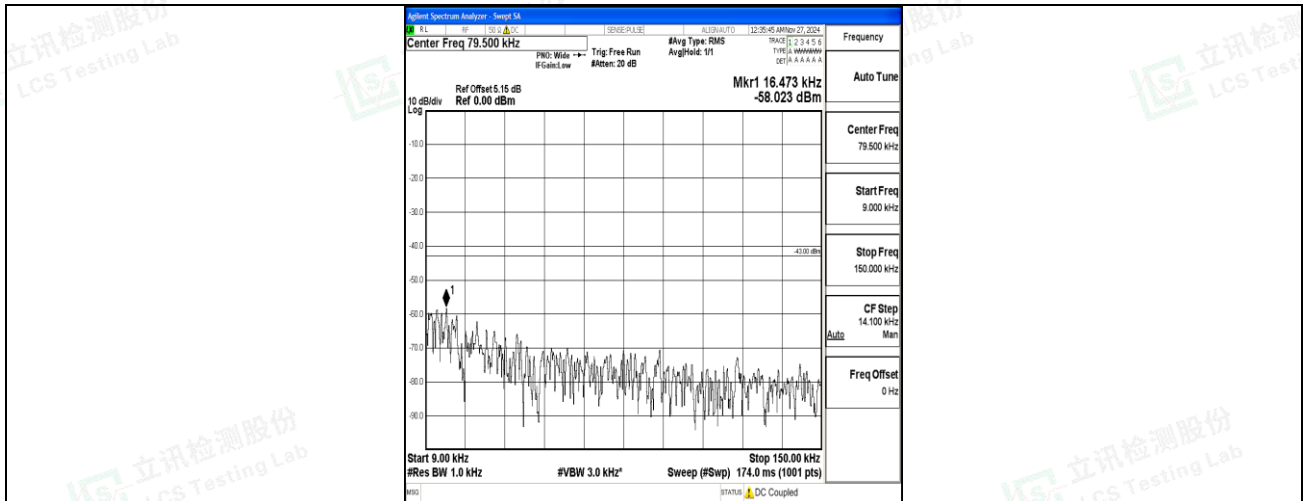
Band66_5MHz_QPSK_132322_1RB#0_0.009~0.15_0.009~0.15
