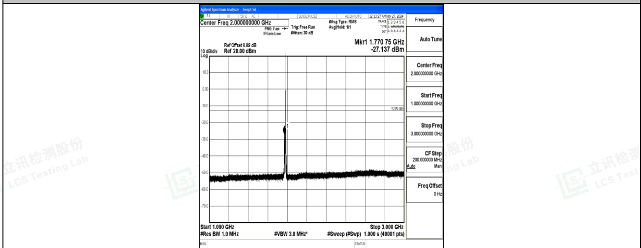
Band66_3MHz_QPSK_132657_1RB#0_1000~3000_1000~3000
