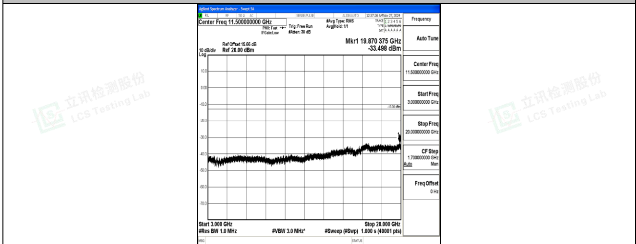
Band66_5MHz_QPSK_132647_1RB#0_3000~20000_3000~20000
