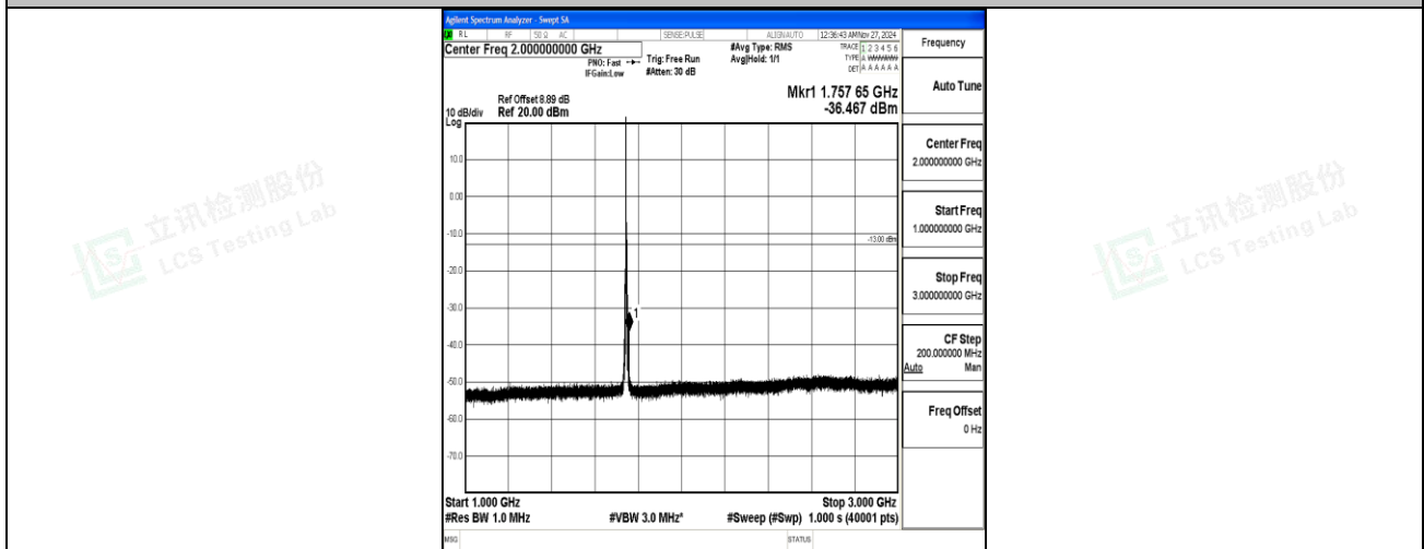
Band66_5MHz_16QAM_132322_1RB#0_1000~3000_1000~3000
