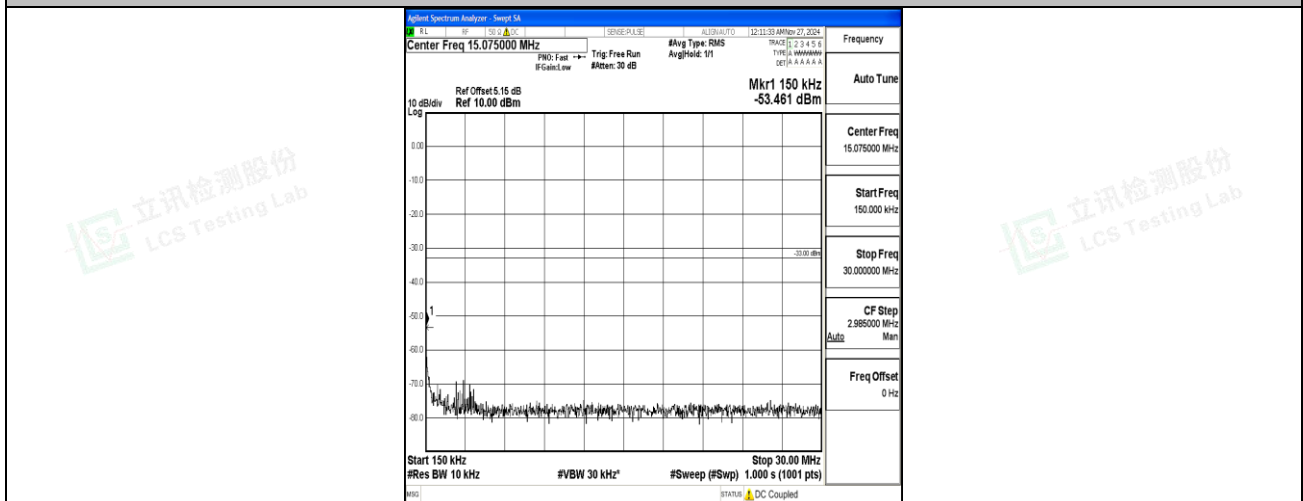
Band66_3MHz_16QAM_131987_1RB#0_0.15~30_0.15~30
