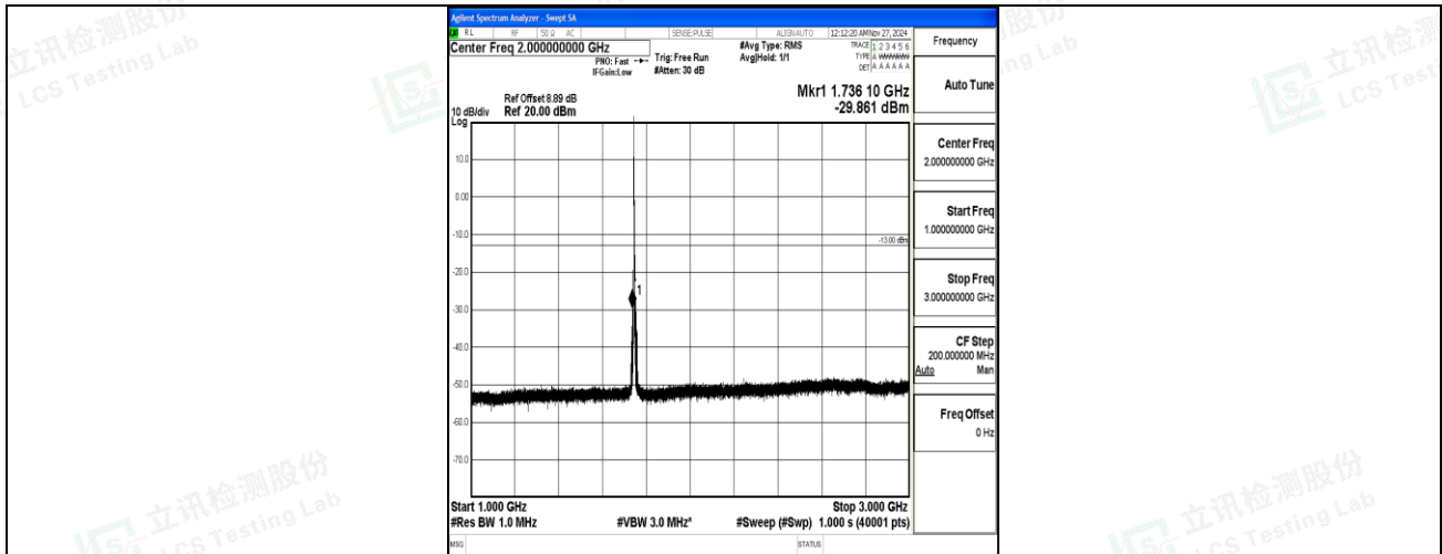
Band66_3MHz_QPSK_132322_1RB#0_1000~3000_1000~3000
