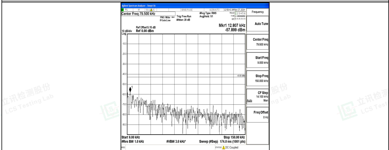
Band66_10MHz_16QAM_132022_1RB#0_0.009~0.15_0.009~0.15
