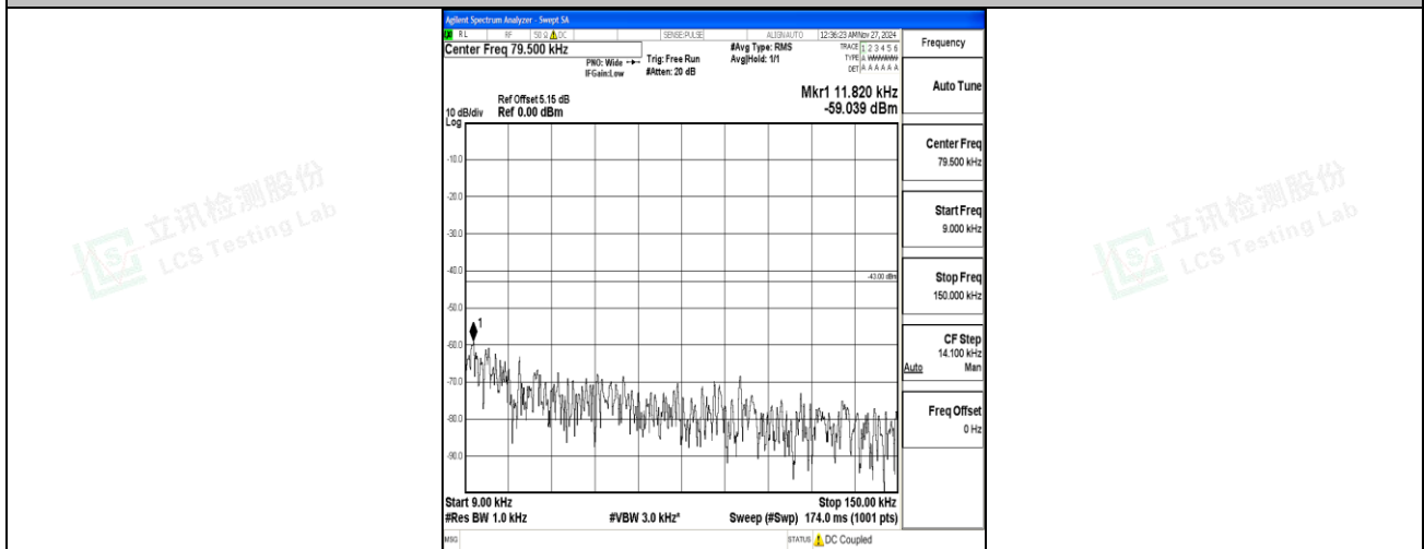
Band66_5MHz_16QAM_132322_1RB#0_0.009~0.15_0.009~0.15
