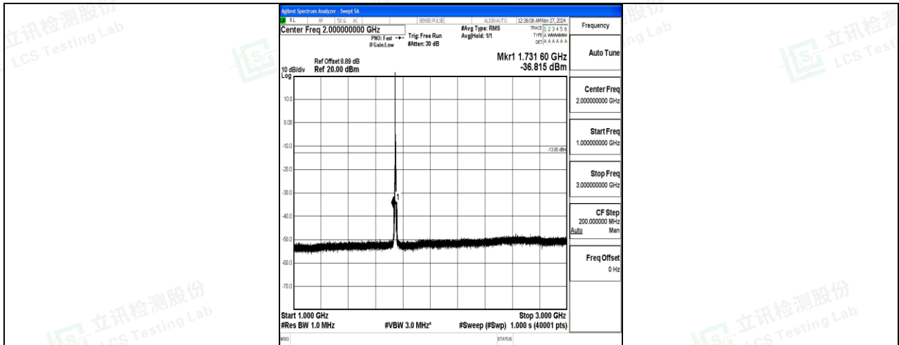
Band66_5MHz_QPSK_132322_1RB#0_1000~3000_1000~3000
