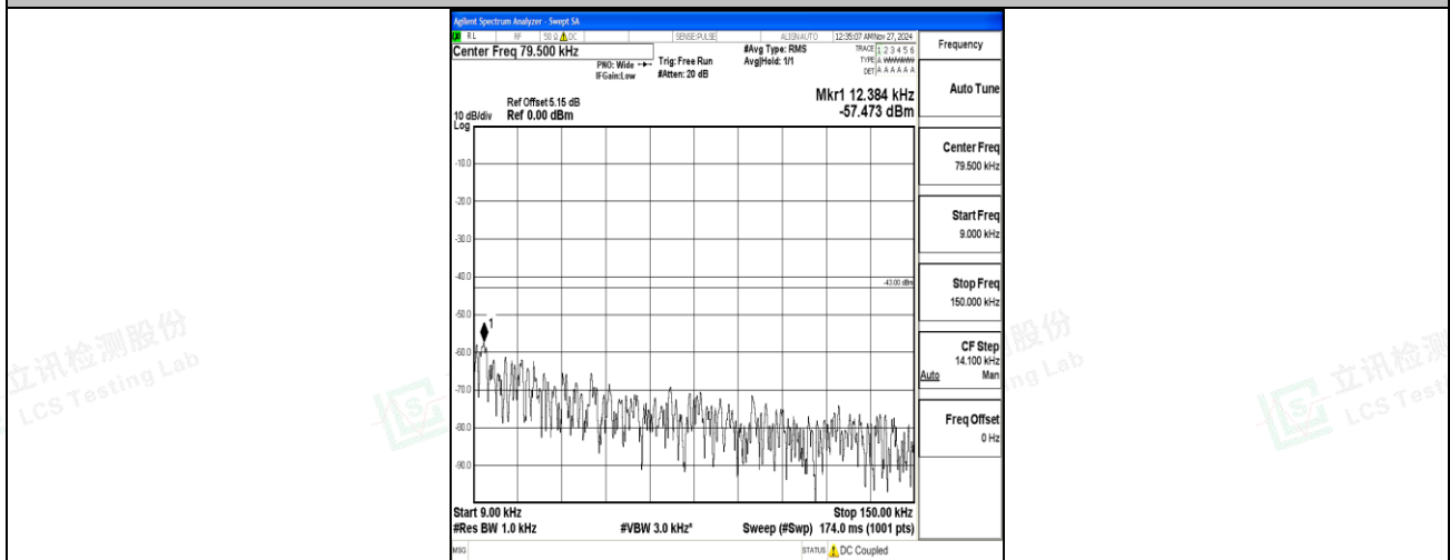
Band66_5MHz_16QAM_131997_1RB#0_0.009~0.15_0.009~0.15
