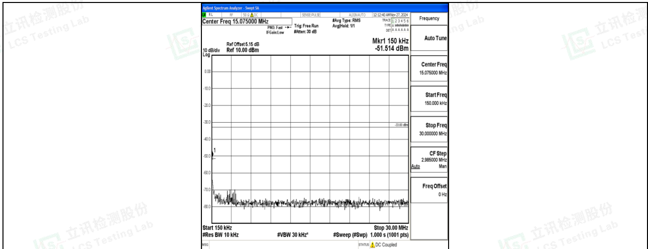
Band66_3MHz_16QAM_132322_1RB#0_0.15~30_0.15~30
