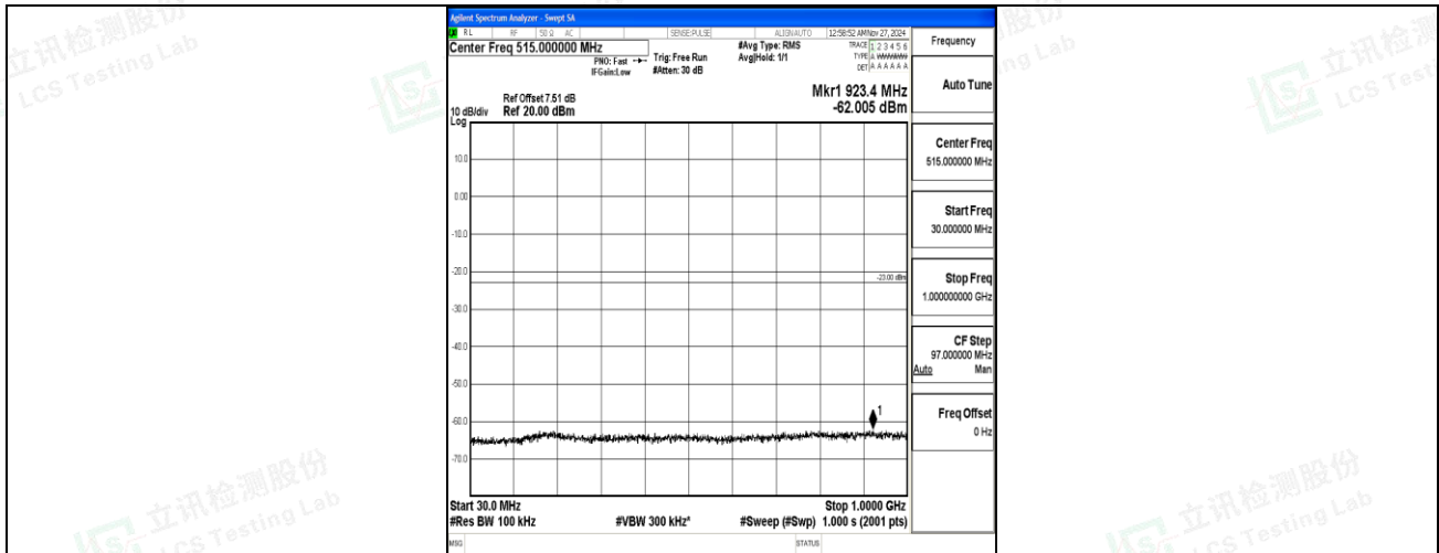
Band66_10MHz_16QAM_132022_1RB#0_30~1000_30~1000
