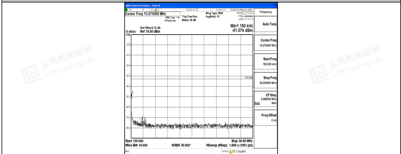
Band66_10MHz_QPSK_132622_1RB#0_0.15~30_0.15~30
