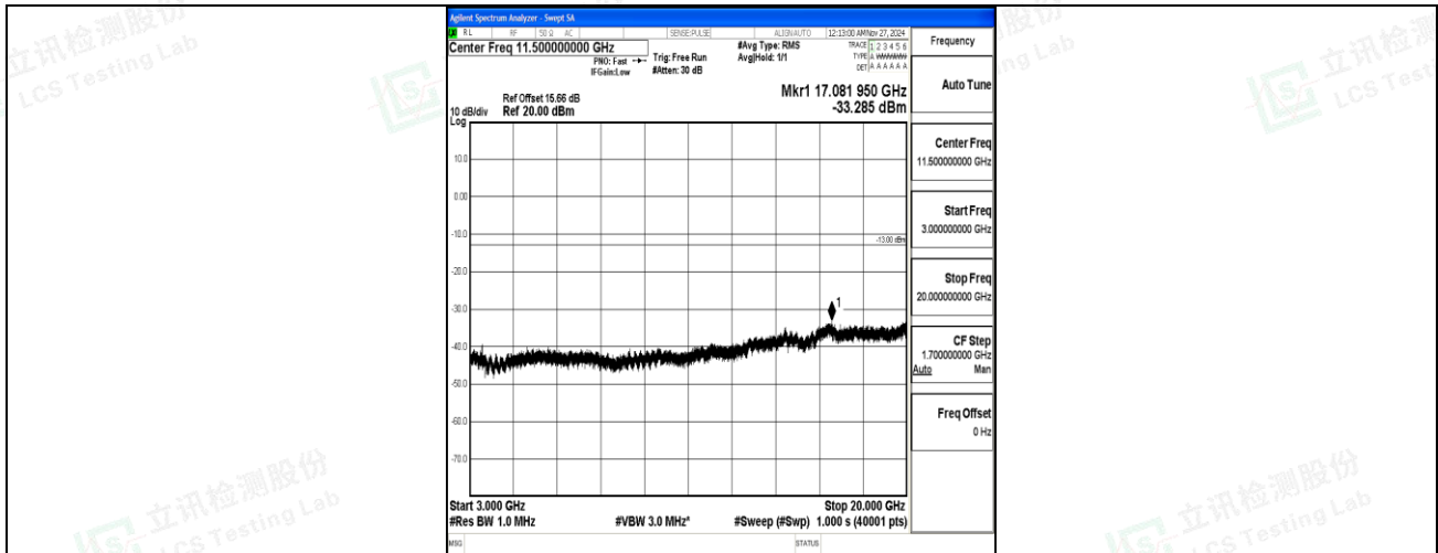
Band66_3MHz_16QAM_132322_1RB#0_3000~20000_3000~20000
