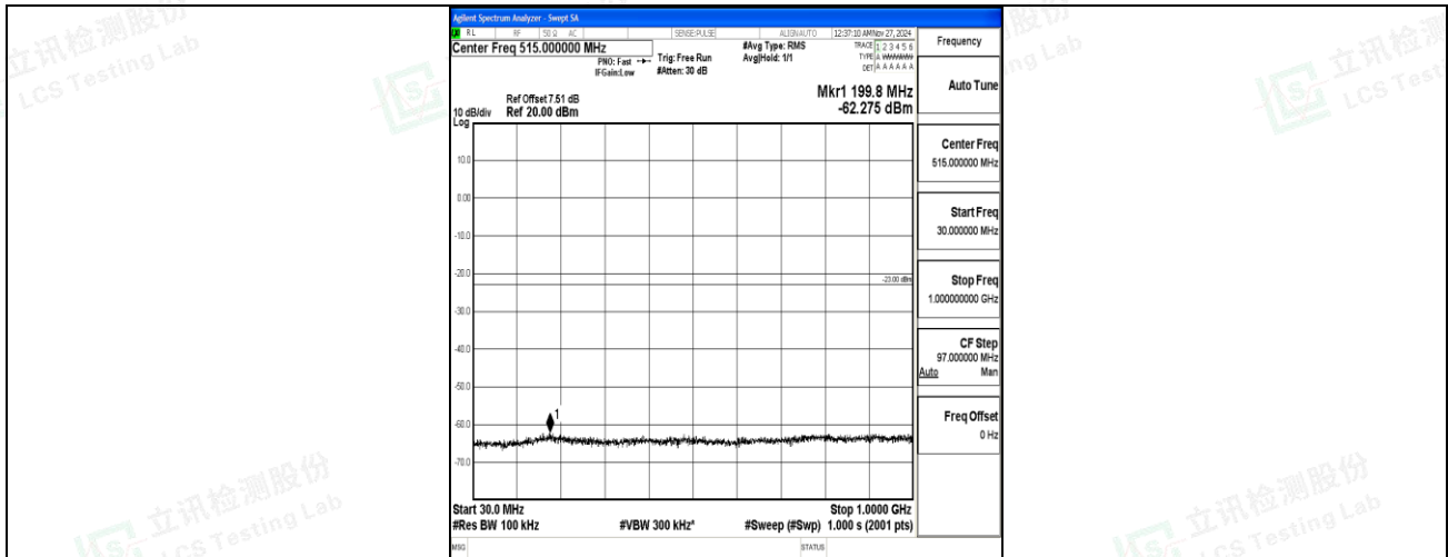
Band66_5MHz_QPSK_132647_1RB#0_30~1000_30~1000
