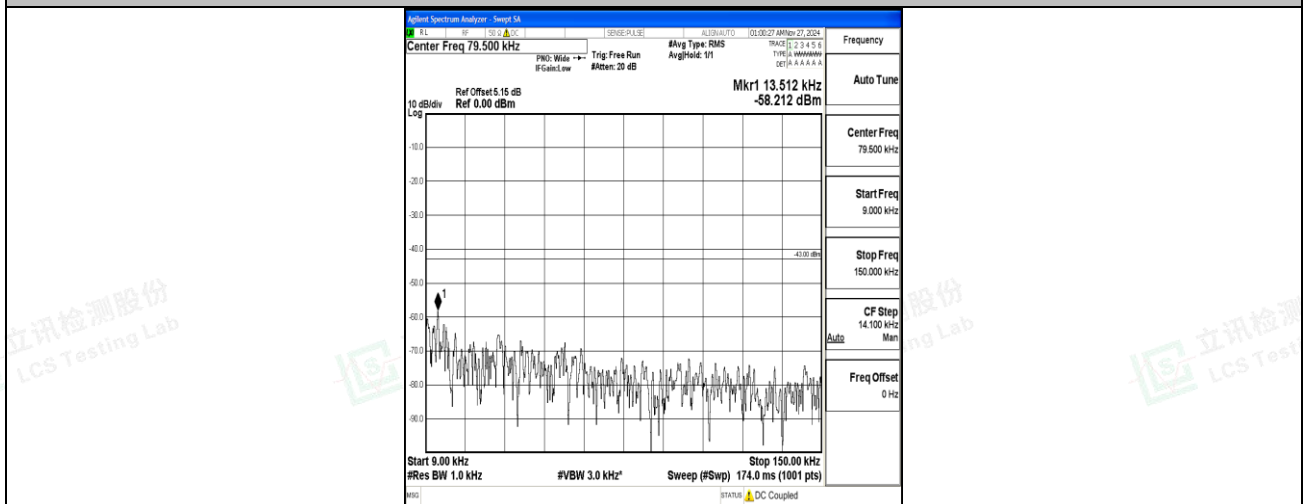
Band66_10MHz_QPSK_132622_1RB#0_0.009~0.15_0.009~0.15
