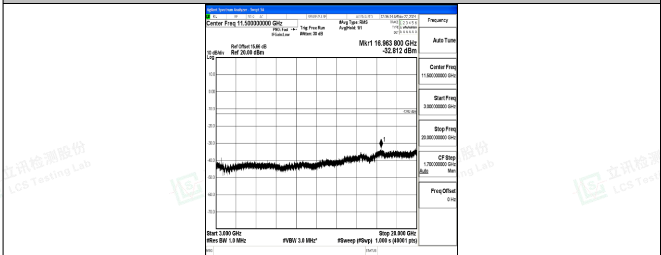
Band66_5MHz_QPSK_132322_1RB#0_3000~20000_3000~20000
