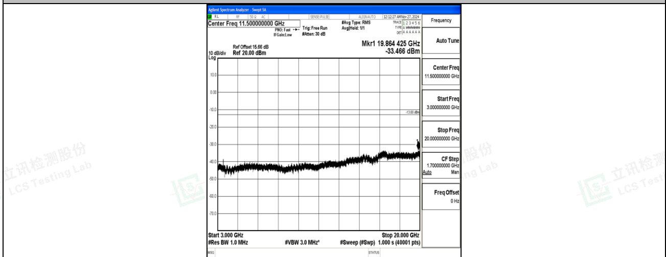
Band66_3MHz_QPSK_132322_1RB#0_3000~20000_3000~20000
