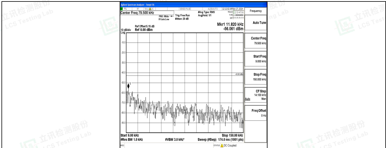
Band66_3MHz_QPSK_132322_1RB#0_0.009~0.15_0.009~0.15
