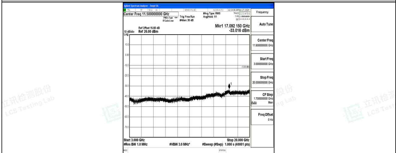
Band66_3MHz_16QAM_132657_1RB#0_3000~20000_3000~20000
