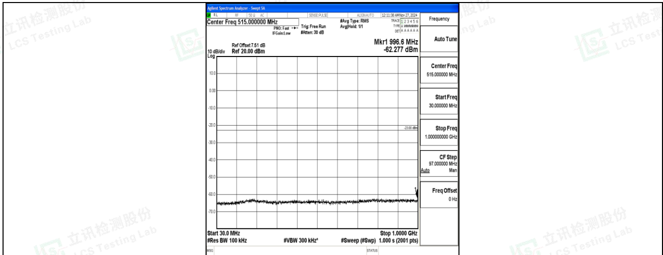
Band66_3MHz_16QAM_131987_1RB#0_30~1000_30~1000
