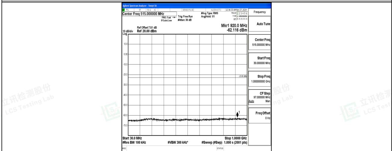
Band66_5MHz_16QAM_132322_1RB#0_30~1000_30~1000
