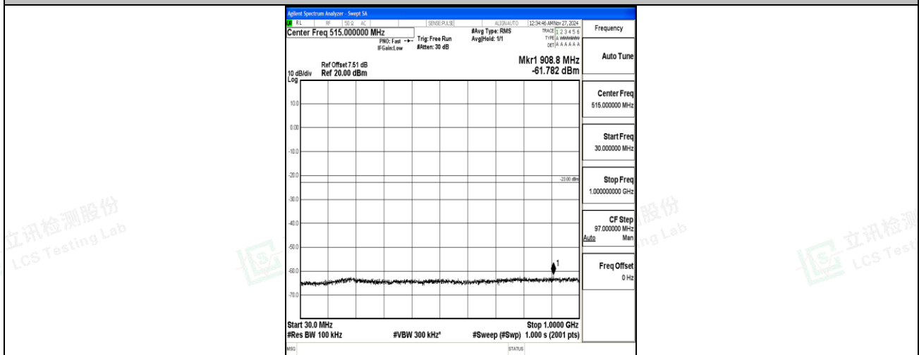
Band66_5MHz_QPSK_131997_1RB#0_30~1000_30~1000
