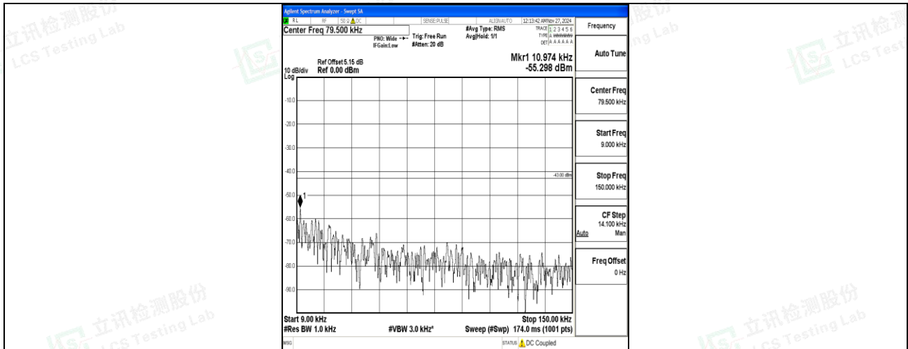
Band66_3MHz_16QAM_132657_1RB#0_0.009~0.15_0.009~0.15
