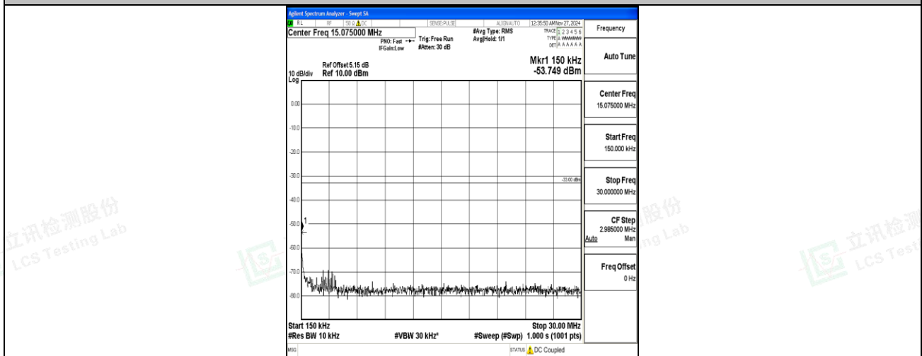
Band66_5MHz_QPSK_132322_1RB#0_0.15~30_0.15~30
