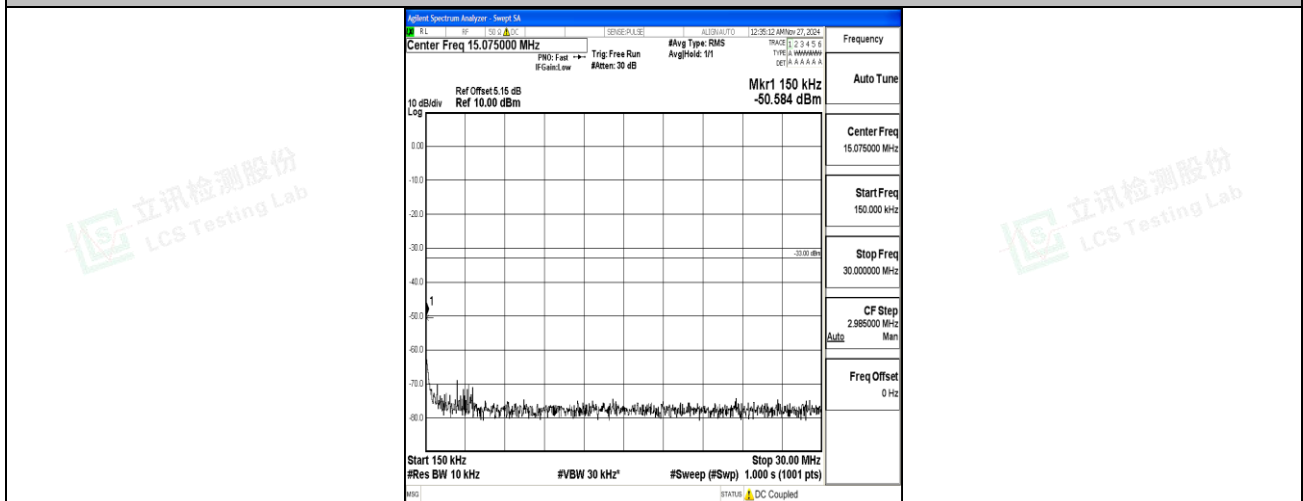
Band66_5MHz_16QAM_131997_1RB#0_0.15~30_0.15~30
