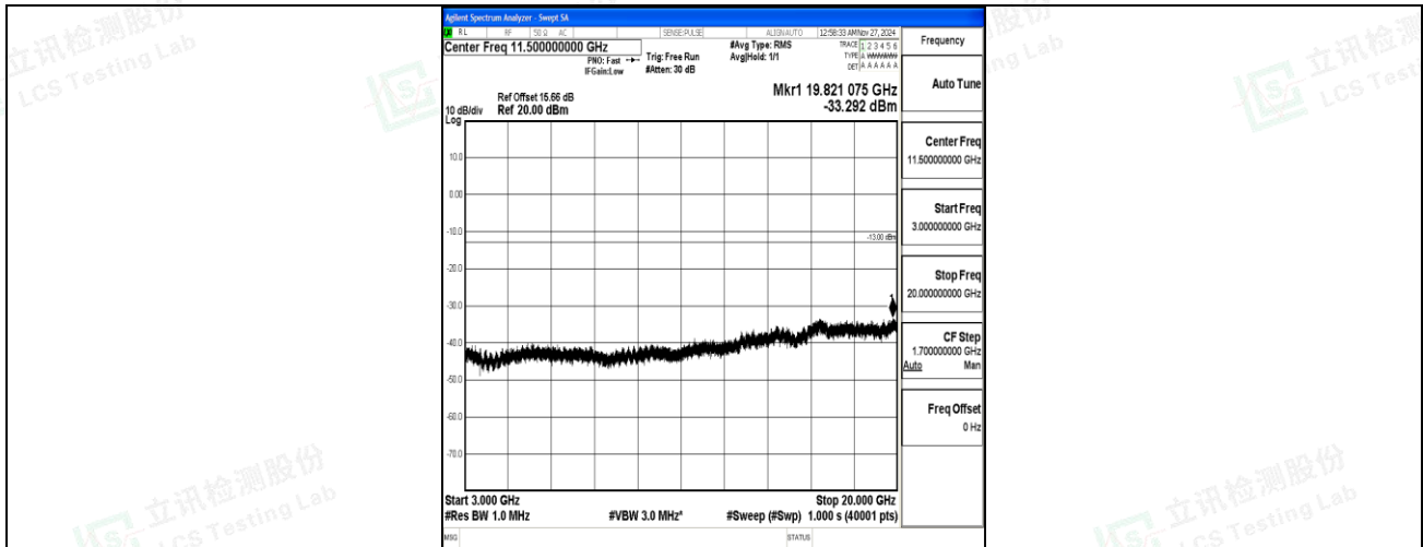
Band66_10MHz_QPSK_132022_1RB#0_3000~20000_3000~20000
