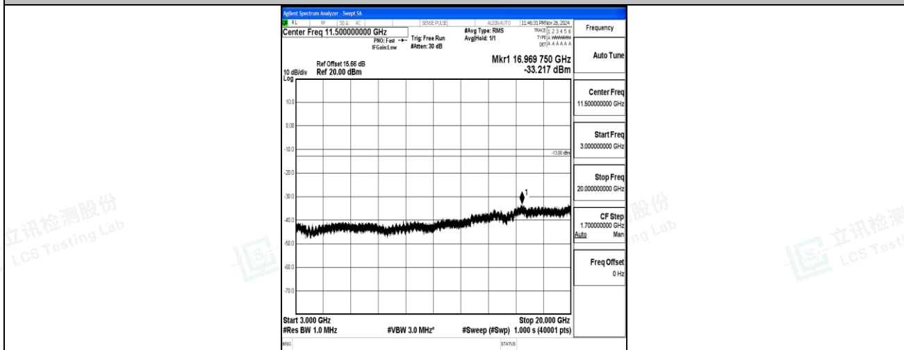
Band66_1.4MHz_16QAM_132665_1RB#0_3000~20000_3000~20000
