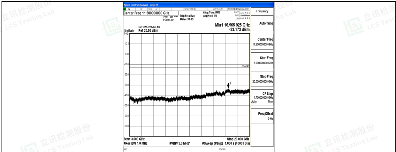
Band66_5MHz_QPSK_131997_1RB#0_3000~20000_3000~20000
