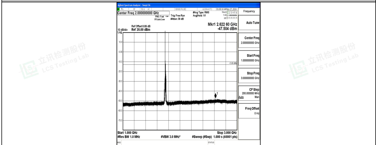
Band66_10MHz_16QAM_132322_1RB#0_1000~3000_1000~3000
