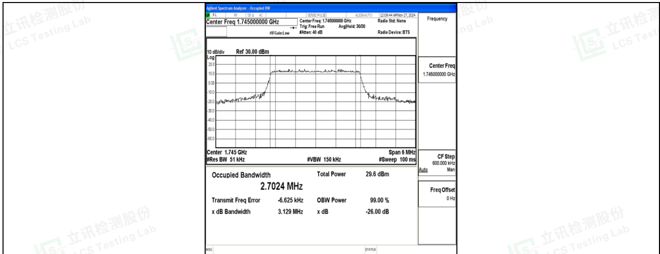
Band66-3MHz-16QAM-132322-15RB#0-PASS
