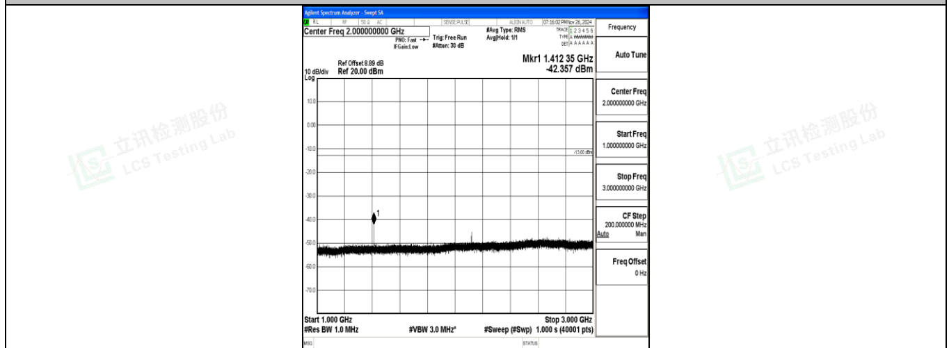
Band12_3MHz_QPSK_23095_1RB#0_1000~3000_1000~3000
