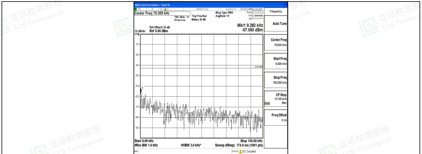
Band12_3MHz_16QAM_23025_1RB#0_0.009~0.15_0.009~0.15
