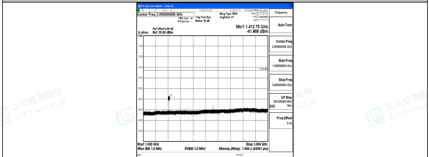
Band12_3MHz_16QAM_23095_1RB#0_1000~3000_1000~3000
