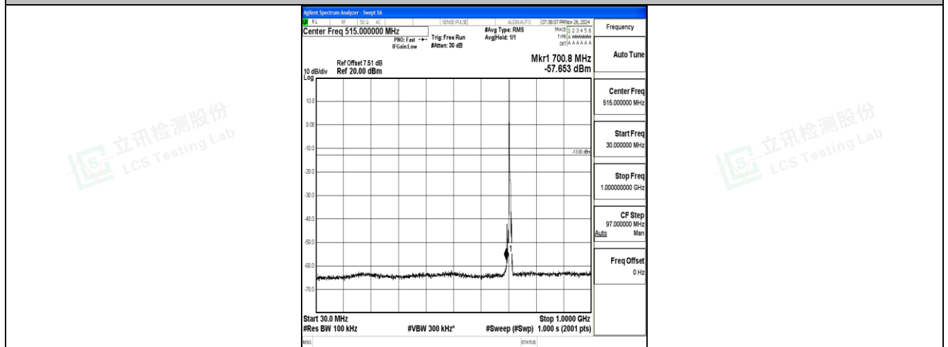
Band12_5MHz_QPSK_23155_1RB#0_30~1000_30~1000
