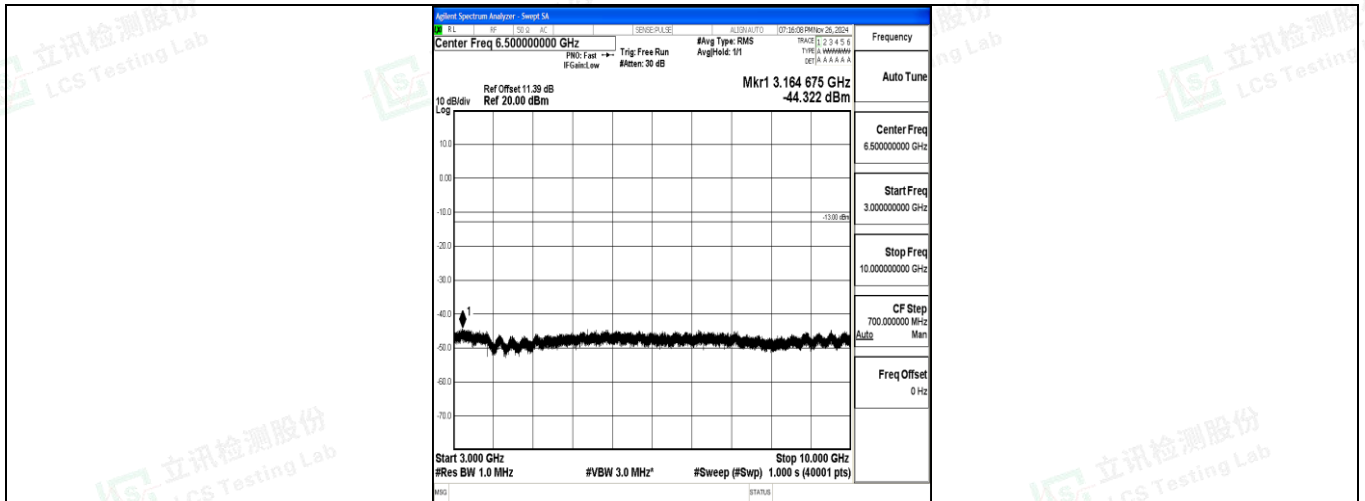
Band12_3MHz_QPSK_23095_1RB#0_3000~10000_3000~10000
