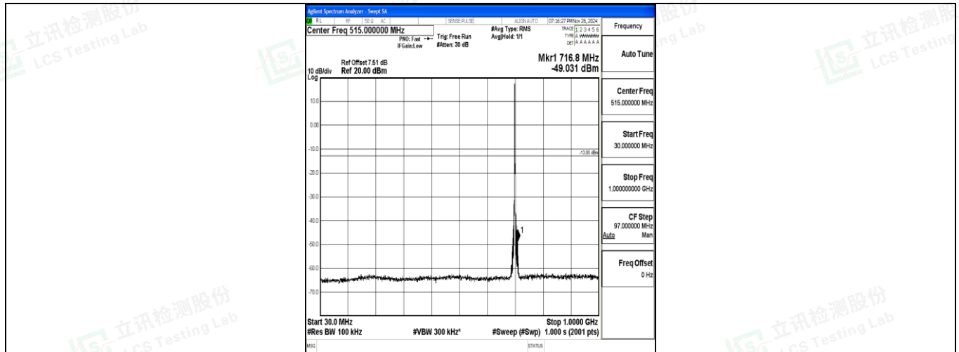
Band12_3MHz_16QAM_23095_1RB#0_30~1000_30~1000
