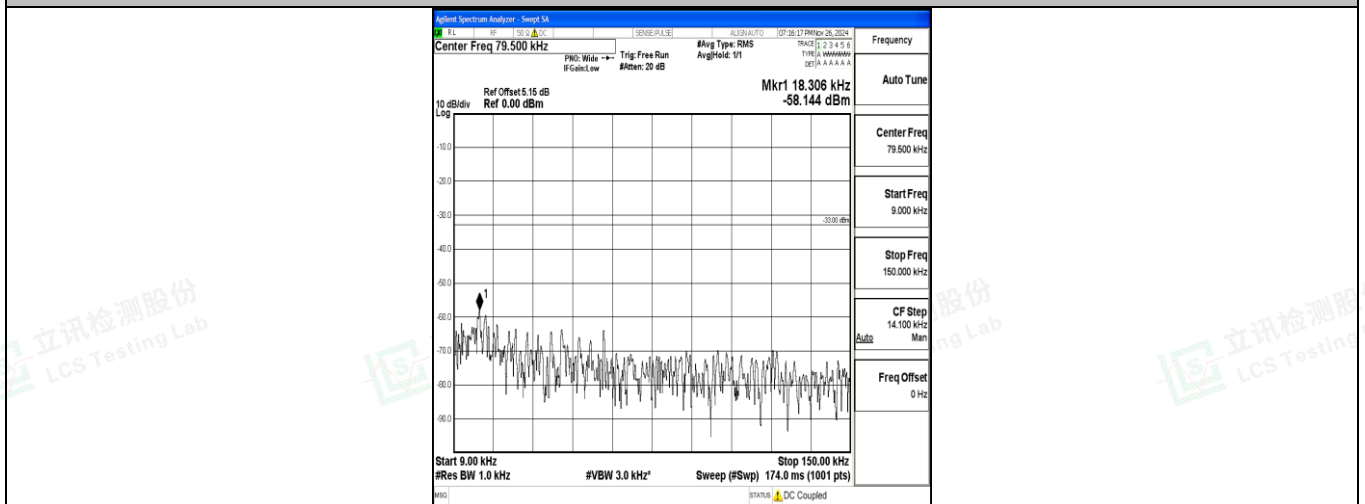
Band12_3MHz_16QAM_23095_1RB#0_0.009~0.15_0.009~0.15
