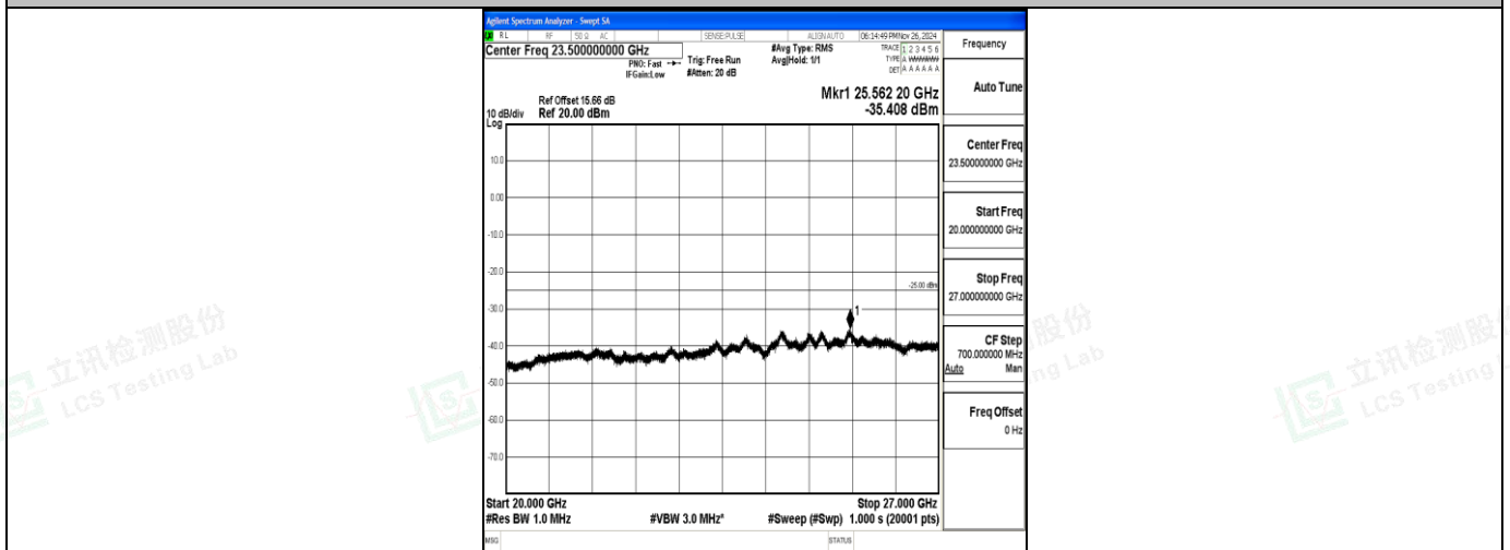
Band7_15MHz_QPSK_21375_1RB#0_20000~27000_20000~27000
