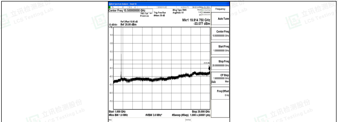
Band7_20MHz_QPSK_21350_1RB#0_1000~20000_1000~20000
