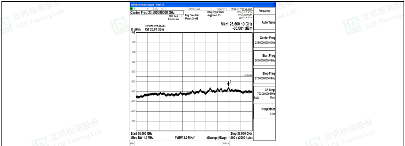
Band7_15MHz_16QAM_21375_1RB#0_20000~27000_20000~27000
