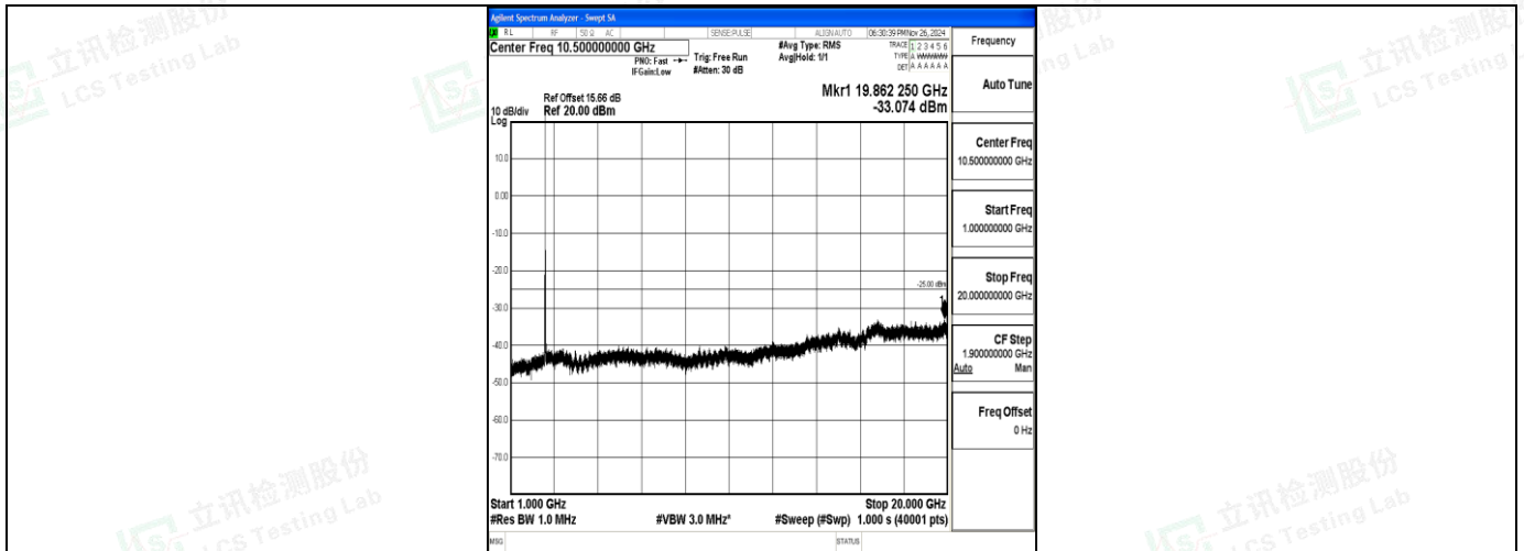
Band7_20MHz_16QAM_20850_1RB#0_1000~20000_1000~20000
