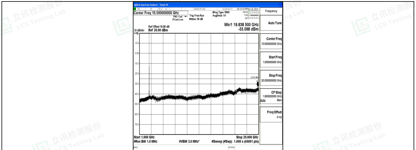
Band7_15MHz_QPSK_21375_1RB#0_1000~20000_1000~20000
