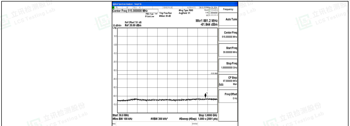
Band7_20MHz_16QAM_21100_1RB#0_30~1000_30~1000
