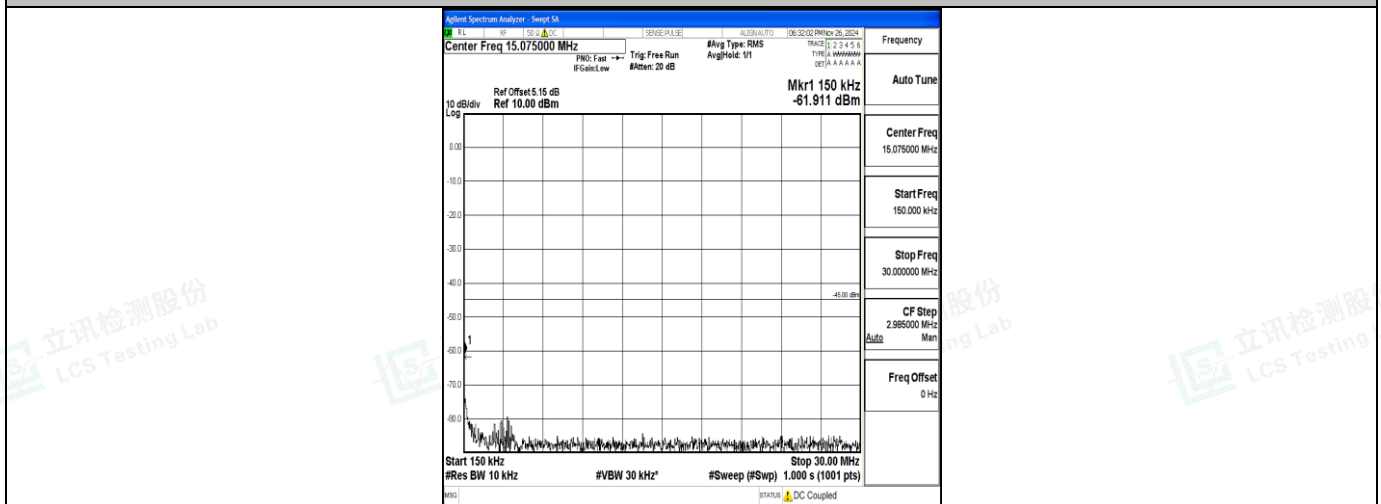
Band7_20MHz_QPSK_21350_1RB#0_0.15~30_0.15~30
