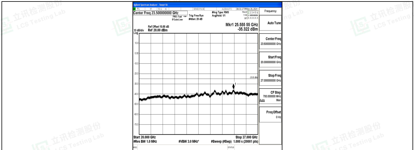
Band7_20MHz_QPSK_21100_1RB#0_20000~27000_20000~27000
