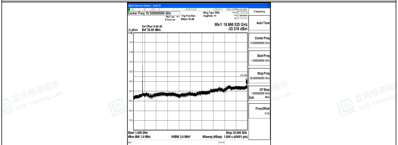
Band7_20MHz_16QAM_21100_1RB#0_1000~20000_1000~20000
