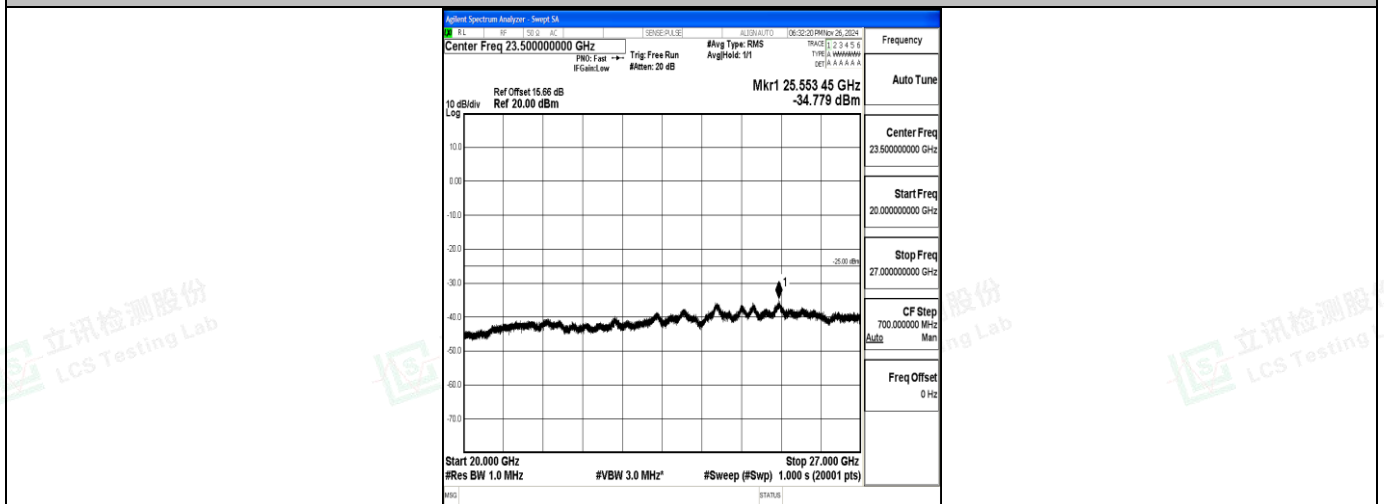
Band7_20MHz_QPSK_21350_1RB#0_20000~27000_20000~27000
