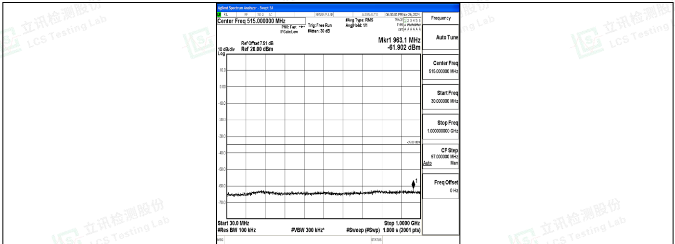
Band7_20MHz_QPSK_20850_1RB#0_30~1000_30~1000
