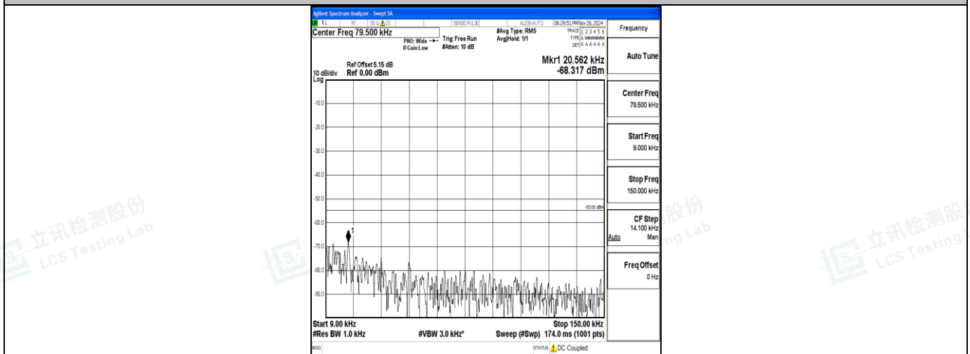
Band7_20MHz_QPSK_20850_1RB#0_0.009~0.15_0.009~0.15
