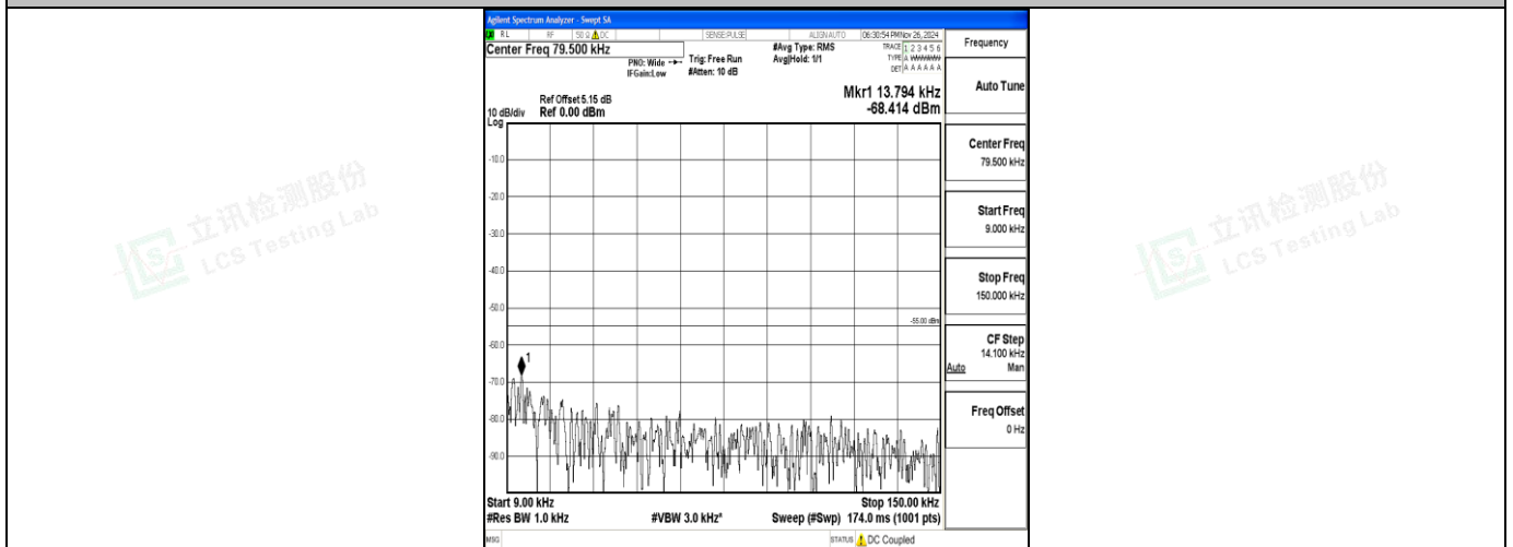
Band7_20MHz_QPSK_21100_1RB#0_0.009~0.15_0.009~0.15
