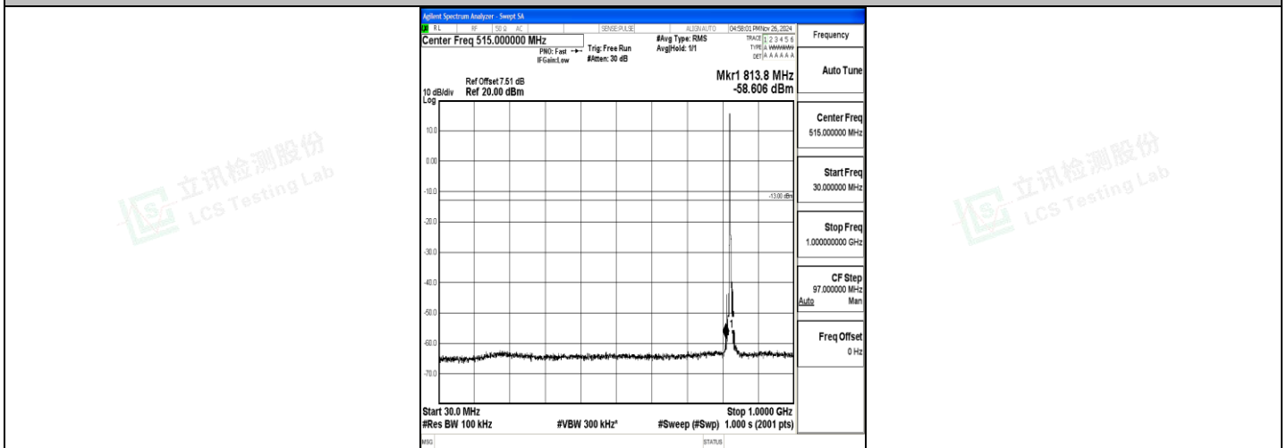
Band5_5MHz_16QAM_20425_1RB#0_30~1000_30~1000
