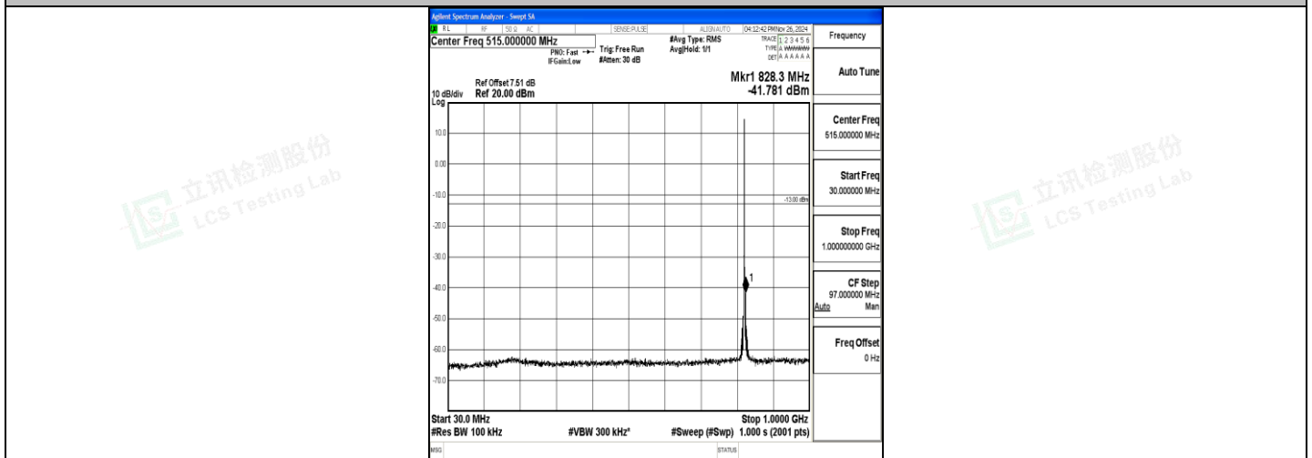
Band5_1.4MHz_16QAM_20407_1RB#0_30~1000_30~1000
