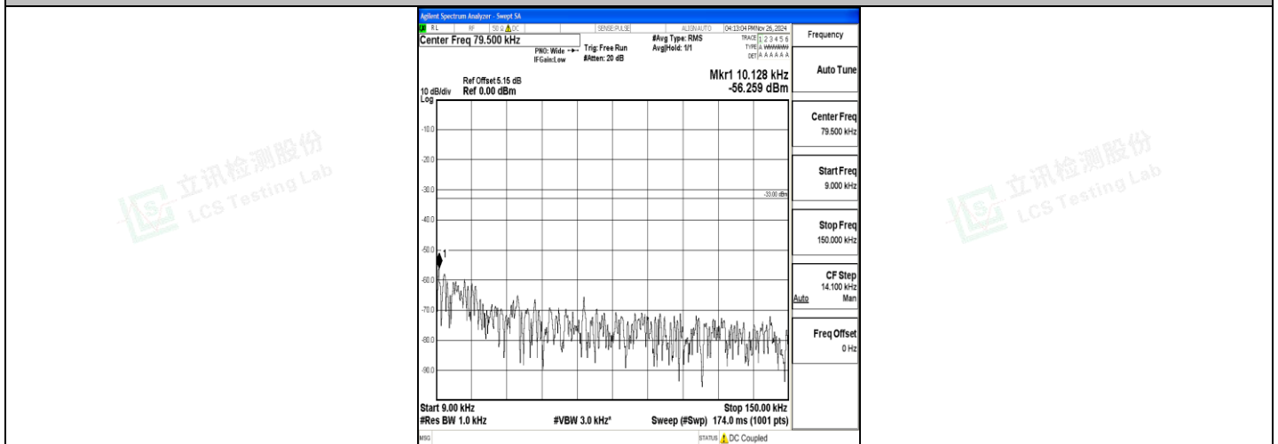
Band5_1.4MHz_QPSK_20525_1RB#0_0.009~0.15_0.009~0.15
