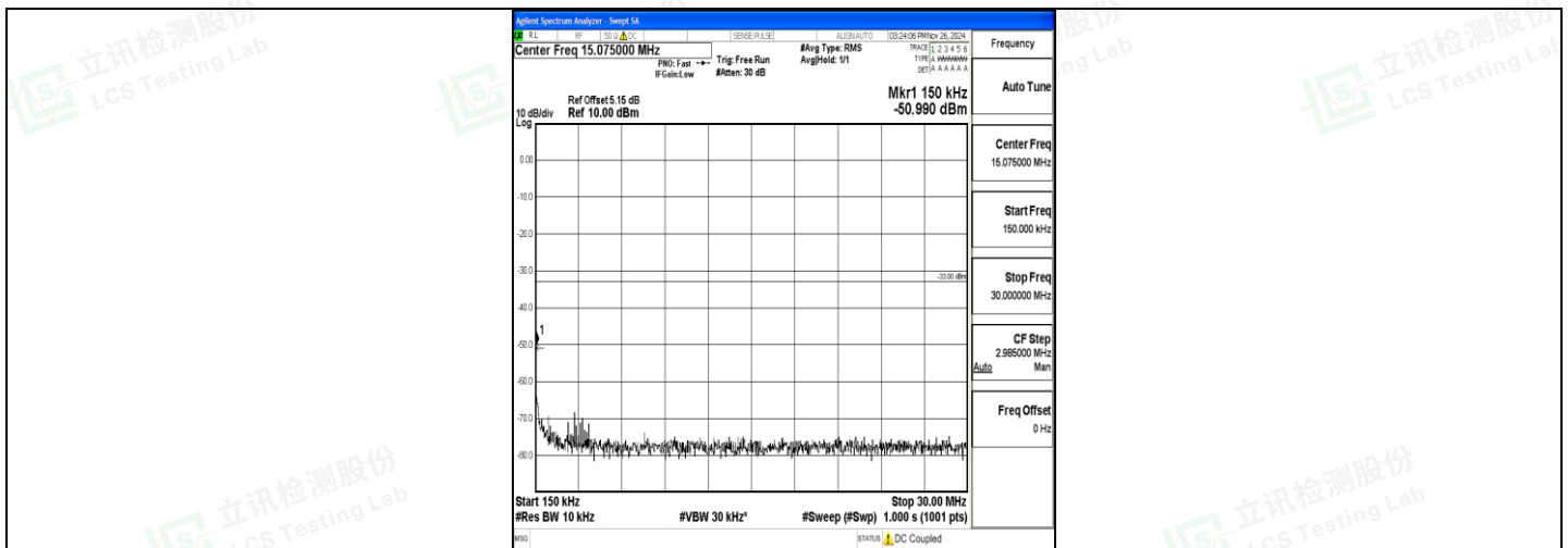
Band4_10MHz_QPSK_20000_1RB#0_0.15~30_0.15~30
