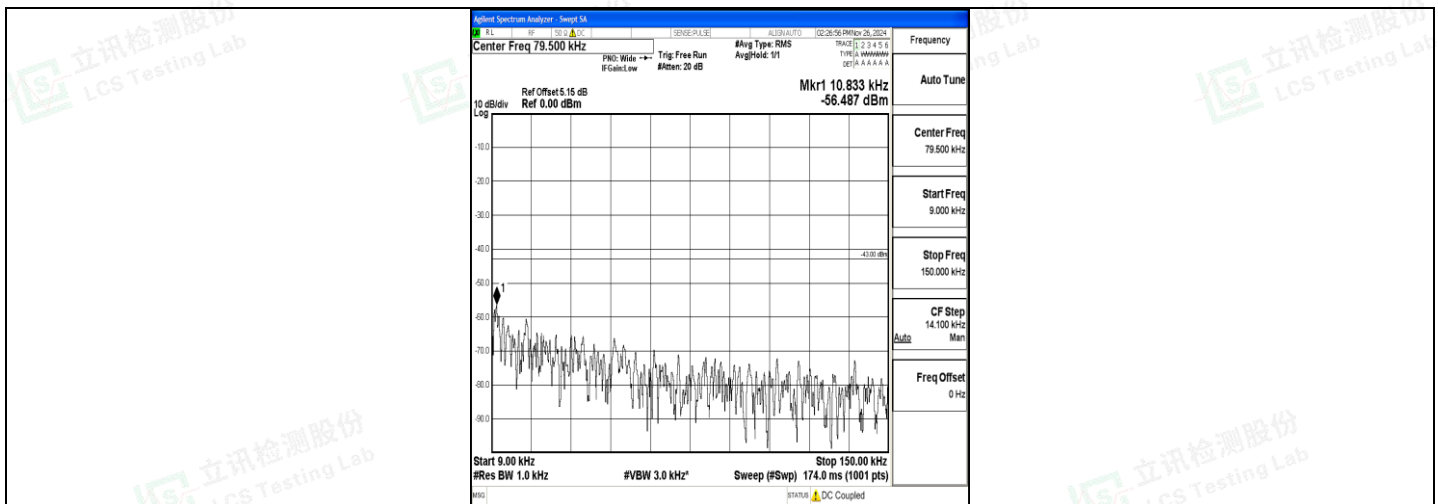
Band4_1.4MHz_16QAM_20393_1RB#0_0.009~0.15_0.009~0.15
