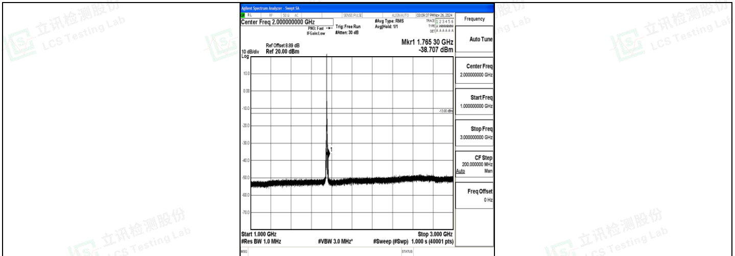
Band4_5MHz_16QAM_20375_1RB#0_1000~3000_1000~3000
