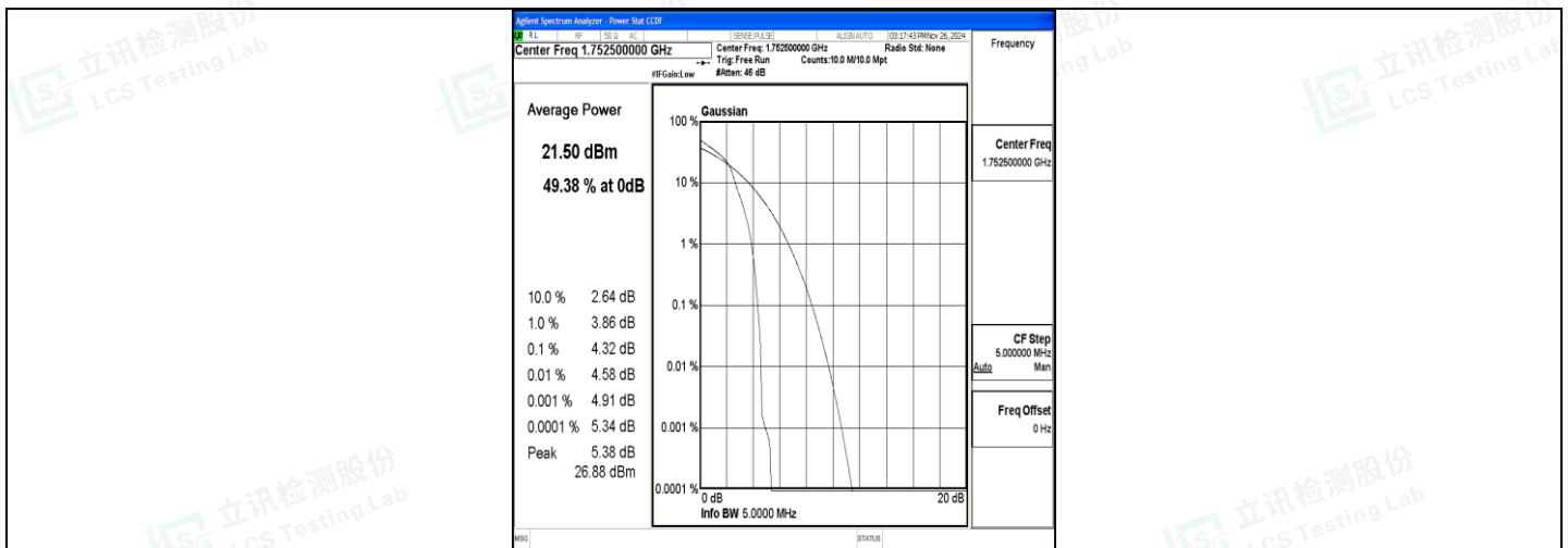
Band4-5MHz-16QAM-20375-1RB#0-PASS
