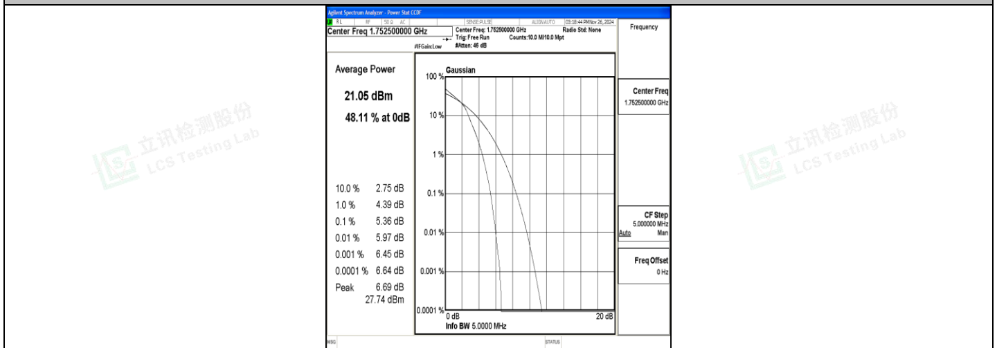
Band4-5MHz-16QAM-20375-25RB#0-PASS
