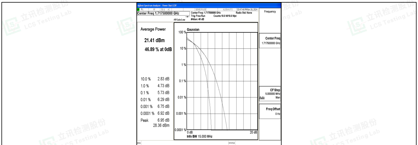
Band4-15MHz-16QAM-20025-75RB#0-PASS
