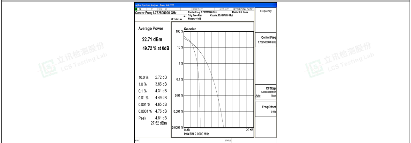
Band4-1.4MHz-16QAM-20175-1RB#0-PASS
