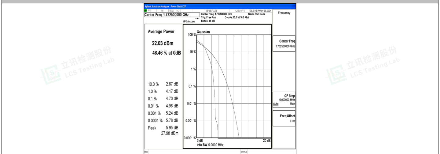
Band4-5MHz-16QAM-20175-1RB#0-PASS
