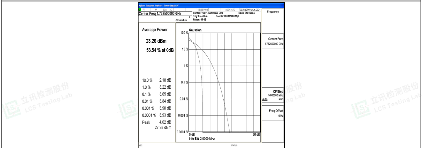
Band4-1.4MHz-QPSK-20175-1RB#0-PASS
