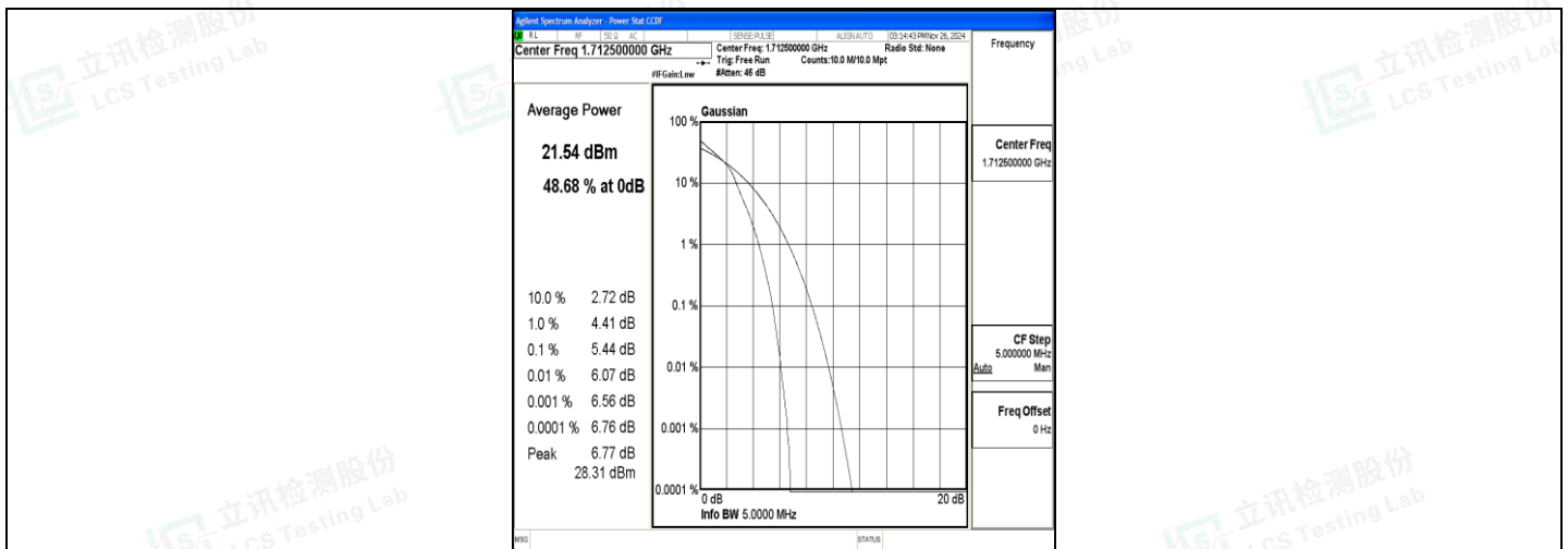
Band4-5MHz-16QAM-19975-25RB#0-PASS
