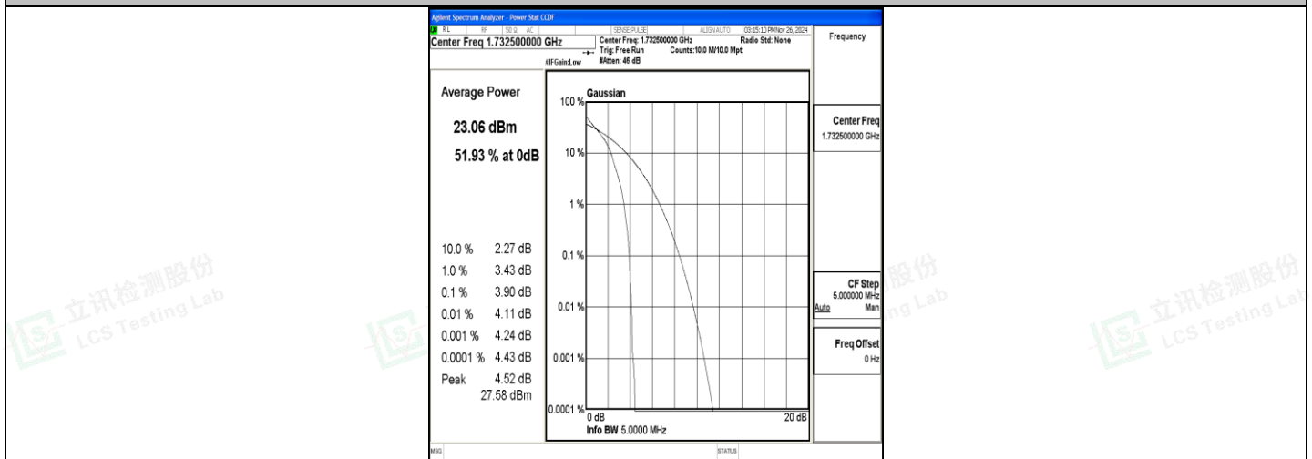
Band4-5MHz-QPSK-20175-1RB#0-PASS
