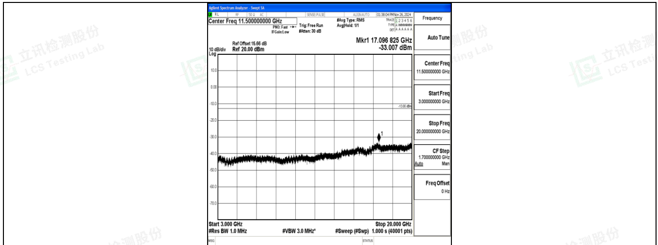
Band2_10MHz_16QAM_18900_1RB#0_3000~20000_3000~20000
