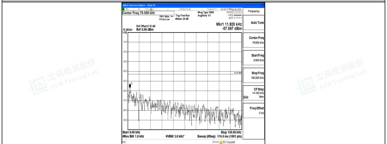
Band2_20MHz_16QAM_18900_1RB#0_0.009~0.15_0.009~0.15
