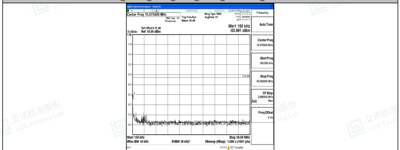
Band2_20MHz_QPSK_18900_1RB#0_0.15~30_0.15~30
