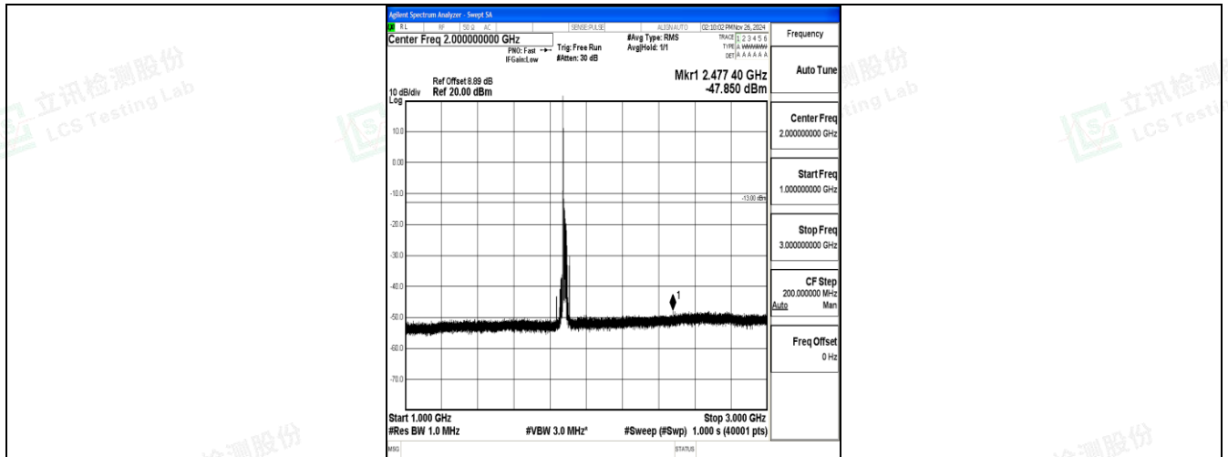
Band2_20MHz_QPSK_18900_1RB#0_1000~3000_1000~3000
