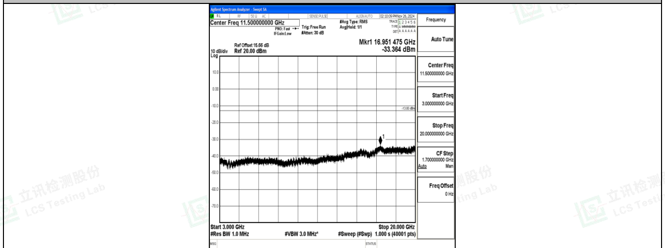
Band2_20MHz_QPSK_18900_1RB#0_3000~20000_3000~20000
