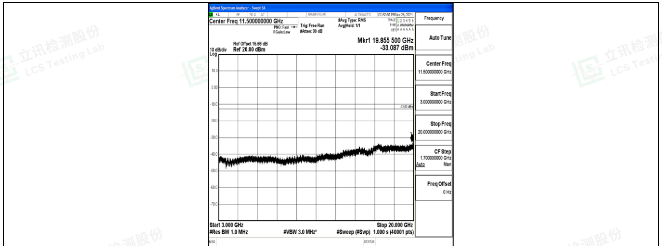
Band2_15MHz_QPSK_18675_1RB#0_3000~20000_3000~20000
