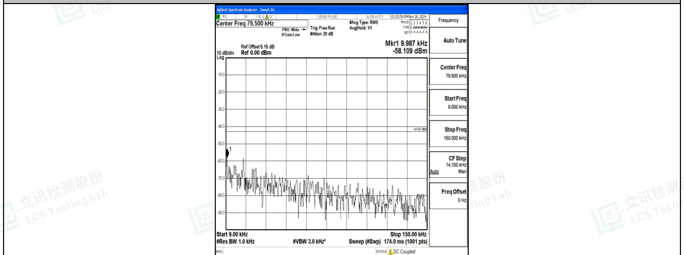
Band2_15MHz_16QAM_18675_1RB#0_0.009~0.15_0.009~0.15
