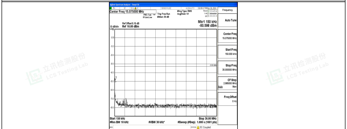
Band2_20MHz_16QAM_18700_1RB#0_0.15~30_0.15~30
