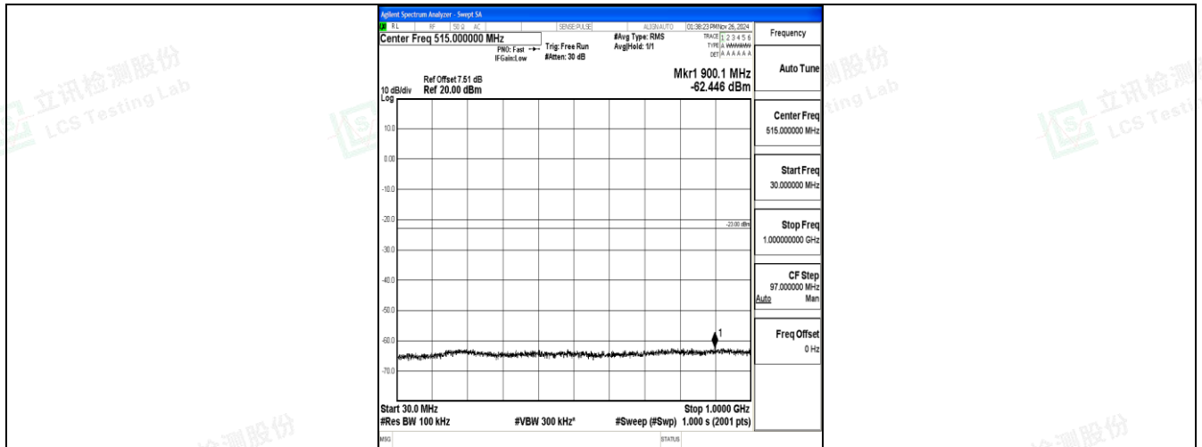
Band2_10MHz_QPSK_19150_1RB#0_30~1000_30~1000
