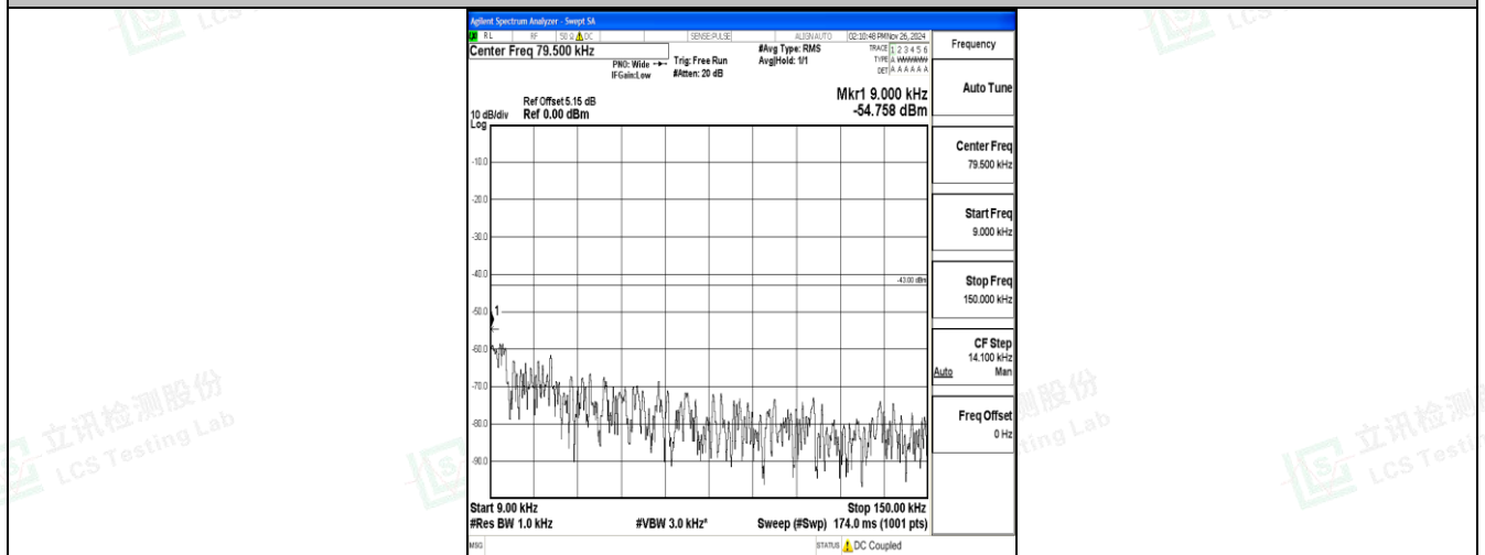
Band2_20MHz_QPSK_19100_1RB#0_0.009~0.15_0.009~0.15
